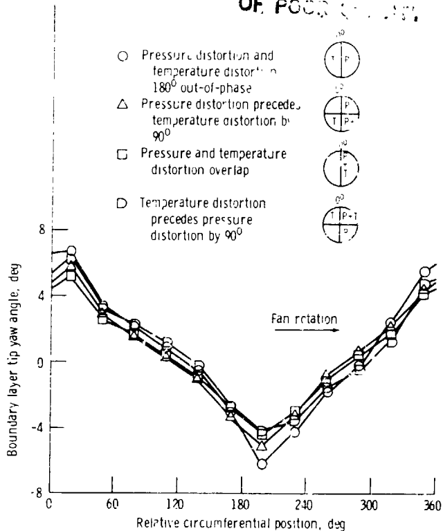
Figure 12 - Boundary layer tip yaw angle variation at station 2 for combined total-pressure and total-temperature distortion
