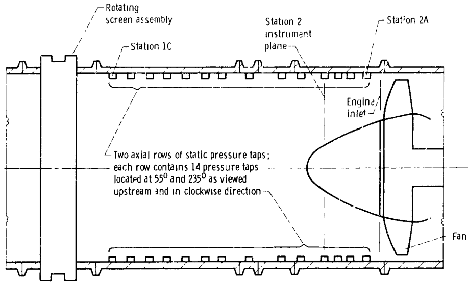
Figure 5. - Inlet ducting assembly.
