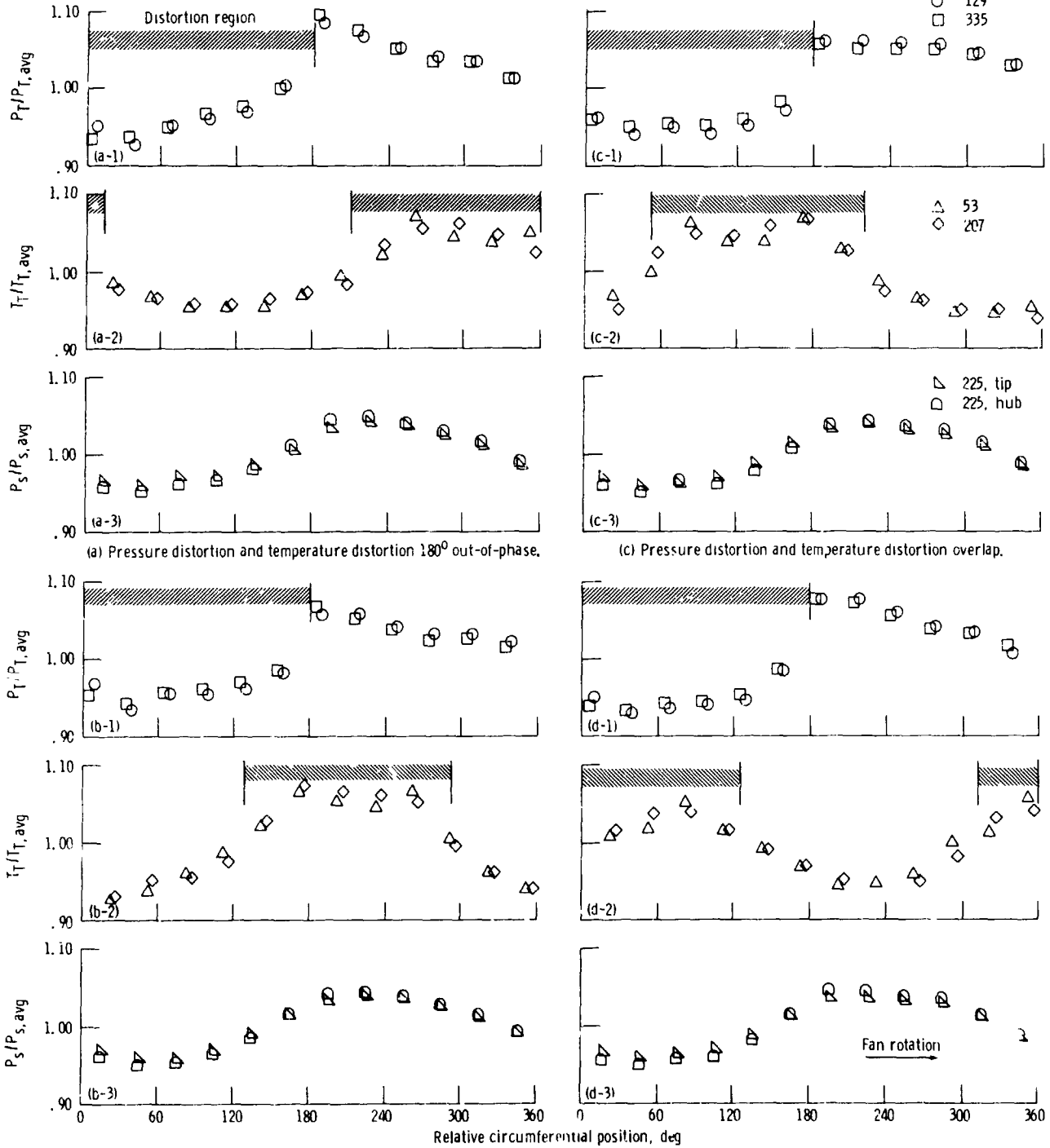
Figure 20. - Circumferential variation of total-pressure, total temperature, and static-pressure profiles at station 2C.
