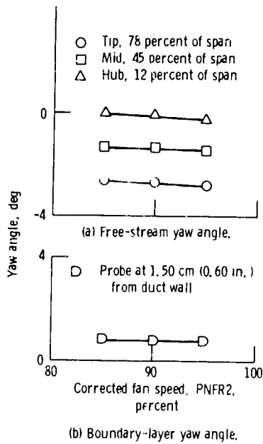
Figure 9. - Flow angle at station 2 versus corrected fan speed with no pressure and temperature distortion (clean inlet).
