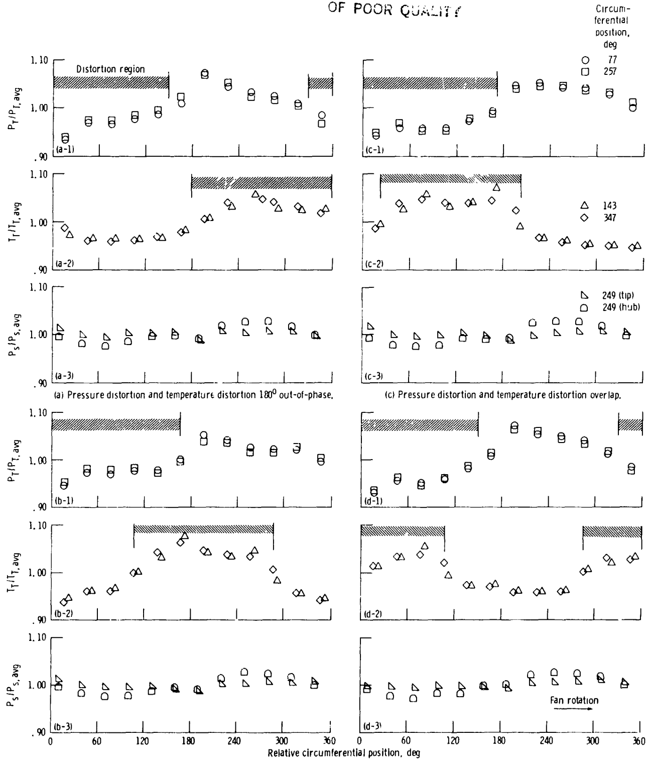
Figure 17. - Circumferential variation of total-pressure, total-temperature and static pressure profiles at station 2.4.
