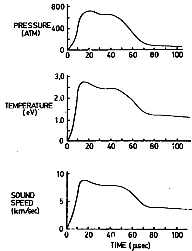
Fig. 13. Calculated Capillary Performance, 2 kJ shot
