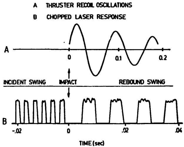
Fig. 5. Thrust Stand Recoil and Calibration Response
