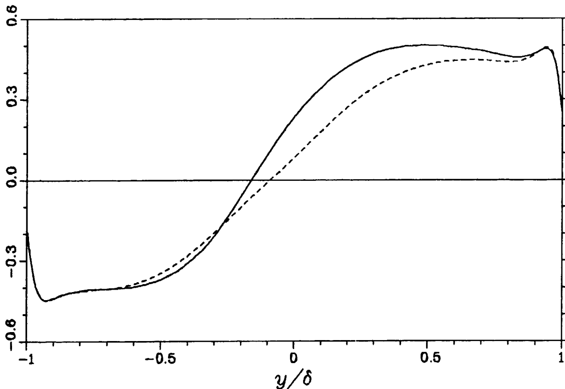
Figure 5.7. Correlation coefficient with and without the contribution of the Taylor-Görtler vortices. ——— \left(\frac{\overline{uv}}{(\overline{u^2}\overline{v^2})^{1/2}}\right) , ---- \left(\frac{u'v'}{(\overline{u'^2}\overline{v'^2})^{1/2}}\right) .
