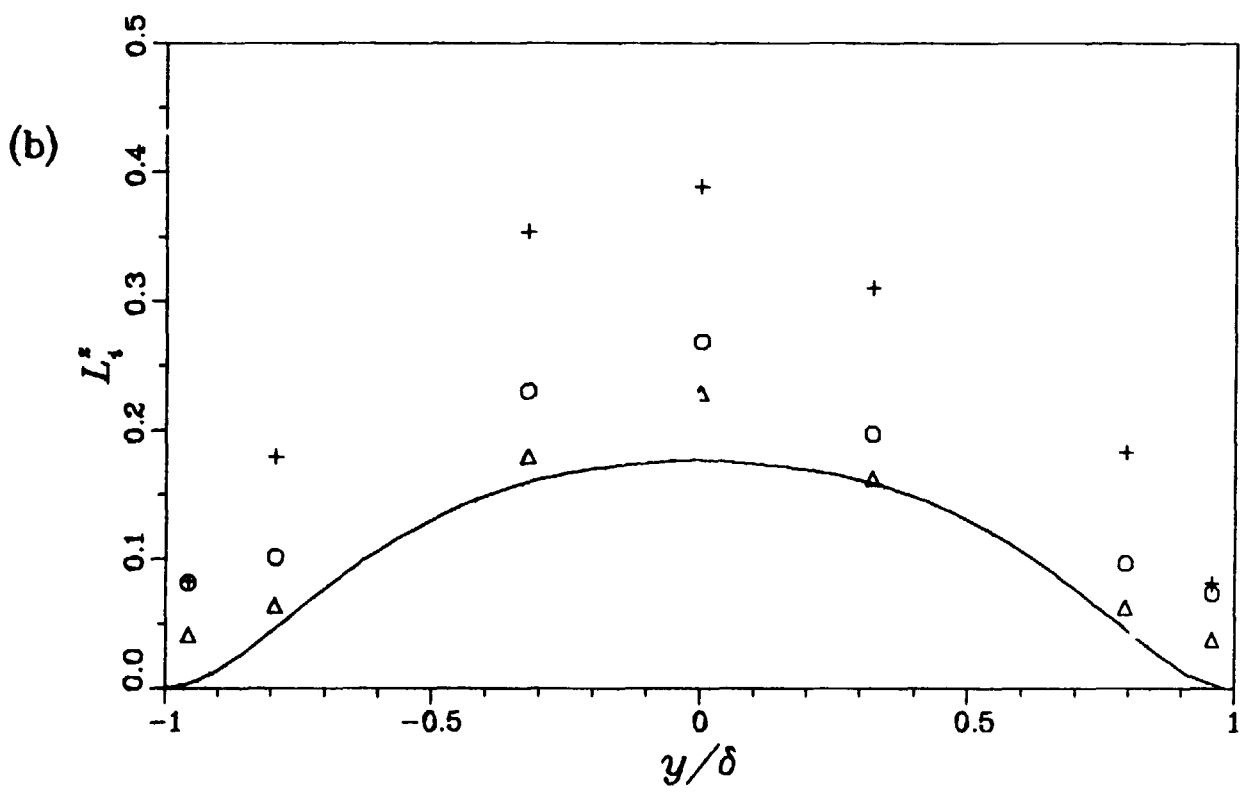
Figure 5.30. Length scales as a function of y . (a) L_i^0 , (b) L_i^z . \circ L_0^j , \Delta L_r^j , + L_z^j , — Norris and Reynolds (1975) for plane channel.
