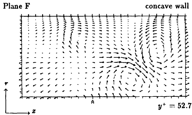
Figure 5.51. Velocity vectors projected into (r, z) -planes at the \theta locations marked "B" through "F" in Figures 5.49 and 5.50. The domain is 135 wall units in the z direction.
