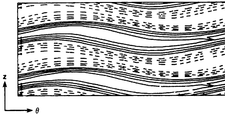
Figure 4.2. Contours of axial velocity at r = 0.822r_0 for fully developed wavy vortices ( Re = 458 , \lambda = 3.0 , \eta = 0.868 , m = 6 ).
