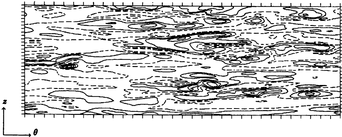
Figure 5.45. Contours of streamwise velocity u' in the (\theta, z) -plane, (a) near the concave wall, y^+ = 6.14 , (b) near the convex wall, y^+ = 5.29 .
