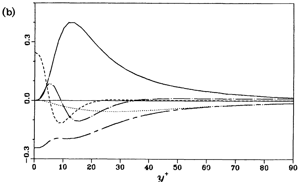
Figure 5.20. Terms in the balance of \overline{u^2}^{1/2} in local wall coordinates, (a) concave wall, (b) convex wall. Legend: — production; - - - radial turbulent diffusion; - · - · - streamwise turbulent diffusion; · · · · · velocity-pressure gradient; - - - - - dissipation; - - - - - radial viscous diffusion.
