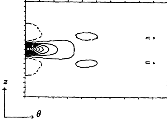
Figure 5.31. Isocorrelation contours in the (\theta, z) -plane at y = .966 , y^+ = 6.13 , (a) R_{00} , (b) R_{rr} , (c) R_{zz} . Contour levels are incremented by 0.1. Domain is 720 local wall units in \theta and 470 units in z .
