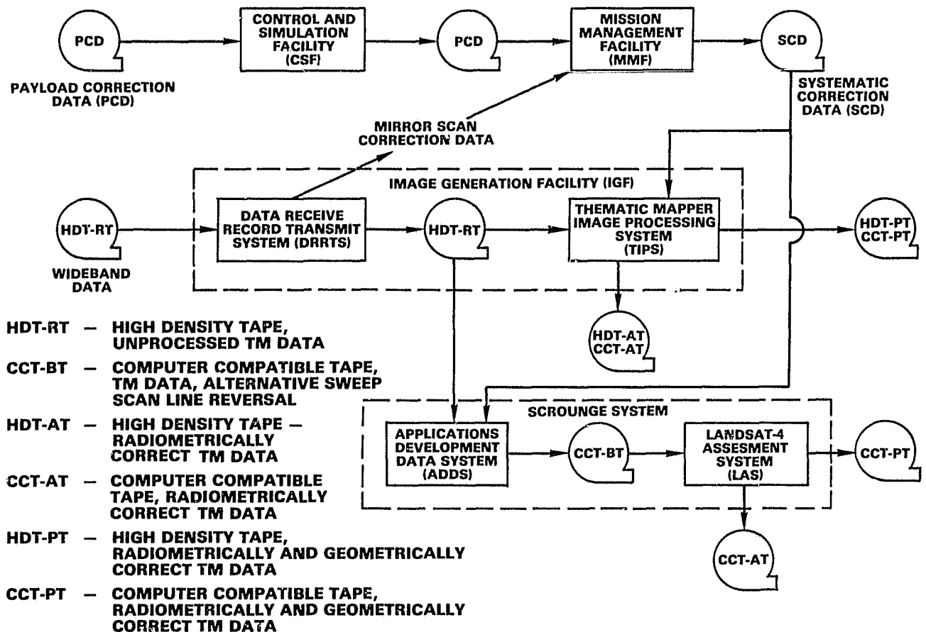
Figure II-10 Thematic Mapper data flow through the ground segment facilities. Note that the use of the
