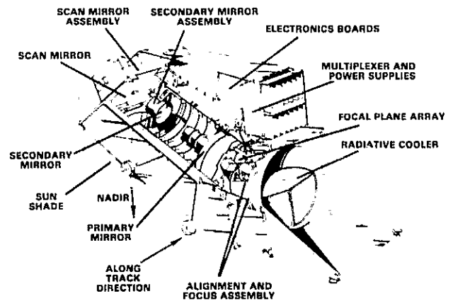
Figure II-5 Cut-a-Way view of the Thematic Mapper.
