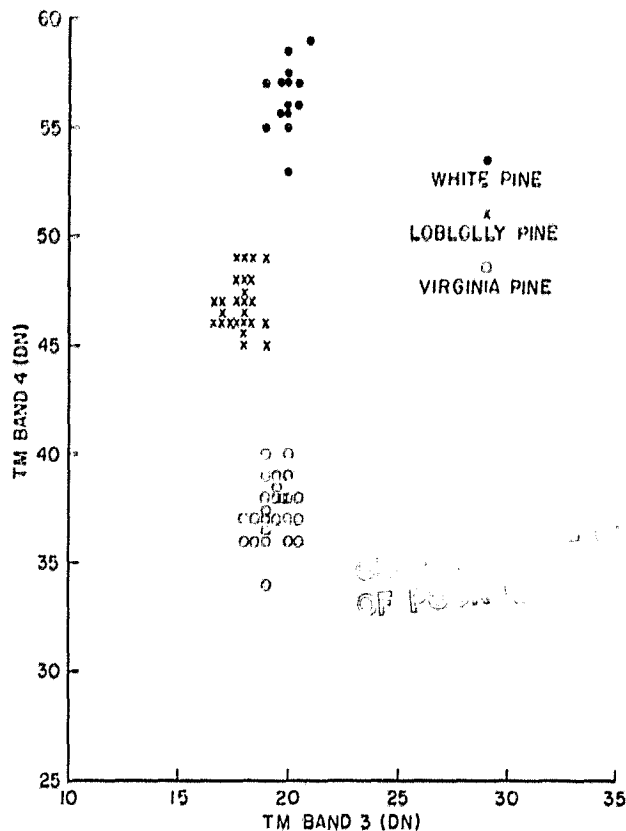
Figure III-1 This graph illustrates the relative spectral response of different evergreen tree species observed in a Landsat 4 TM image of northern Virginia acquired in the fall of 1982. These species have a relatively similar spectral response in the red portion of the visible spectrum (TM band 3), but markedly different spectral characteristics in the near infrared (TM band 4). The level of species discrimination achieved in this scene is due in part to the improved spatial resolution of the TM. (Illustration courtesy of Nancy Milton, U. S. Geological Survey).
