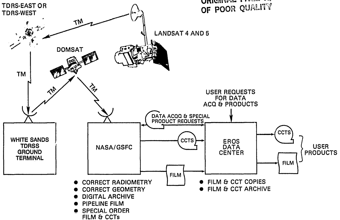
Figure 11-9 End-to-end flow of TM image data from the Landsat 4 and 5 spacecraft to ground-based users.
