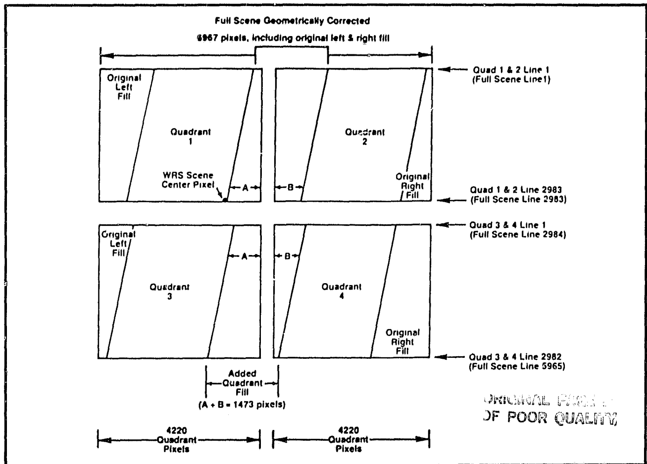
Figure II-15 Pixel and scan-line dimensions of TM scene quadrants for P-data store on CCT's.
