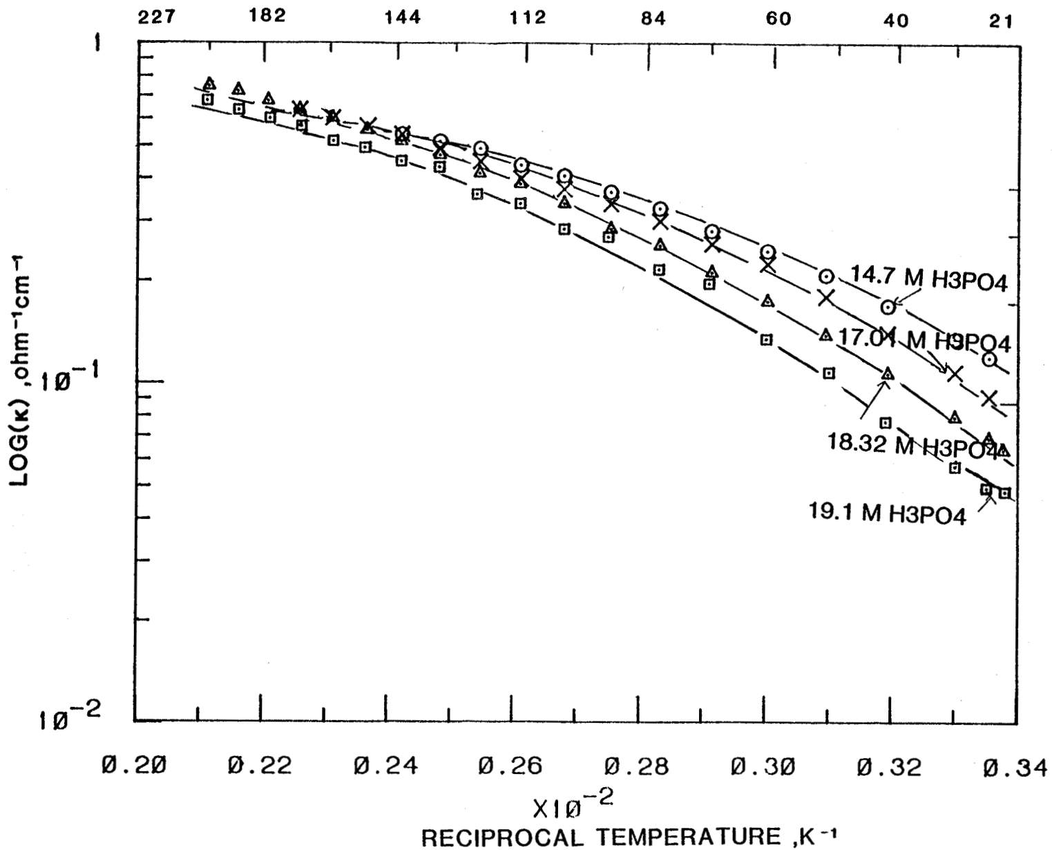
Figure 22 Plot of specific conductivity versus reciprocal temperature at concentrates H 3 PO 4
