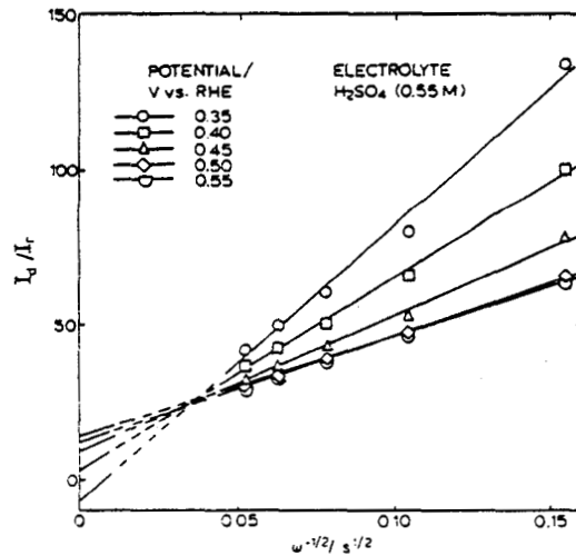
Fig. 7. I_d/I_r vs. \omega^{-1/2} in the potential region 0.55–0.35 V vs. RHE.
