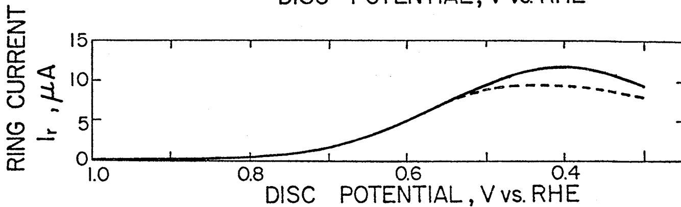
The rotating ring-disc electrode data at \omega = 900 rpm for oxygen reduction at Pt in 6.0 M TFMSA.
