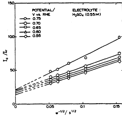
Fig. 6. I_d/I_r vs. \omega^{-1/2} in the potential region 0.75–0.55 V vs. RHE.
