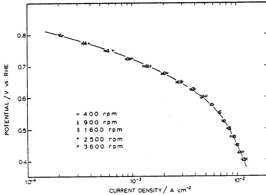
Fig. 4. Mass transfer corrected Tafel plot for O 2 reduction on Pt in 0.55 M H 2 SO 4 at 25°C. The scale in the horizontal axis is for the mass transfer corrected current density, i_{d1}i_d/(i_{d1} - i_d) .
