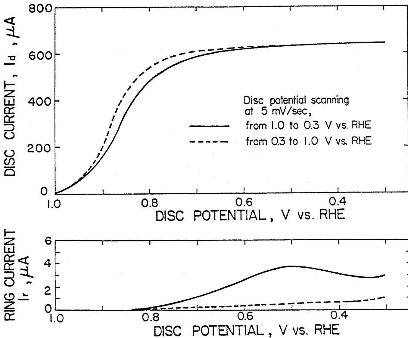
Fig. 11 The rotating ring-disc electrode data at \omega = 900 rpm for oxygen reduction at Pt in 0.05 M TFMSA.
