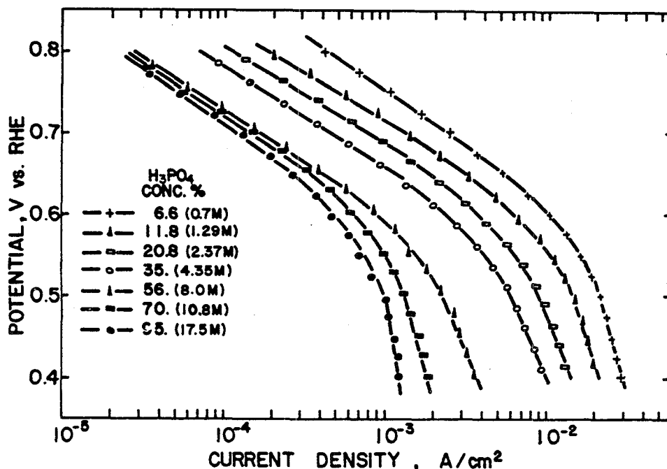
Fig. 2. Mass-transfer-corrected Tafel behavior for oxygen reduction on Pt in H_3PO_4 over the concentration range 6.6-95 w/o at 25°C. Tafel behavior is independent of electrode rotating speed in the 400-3600 rpm region.
