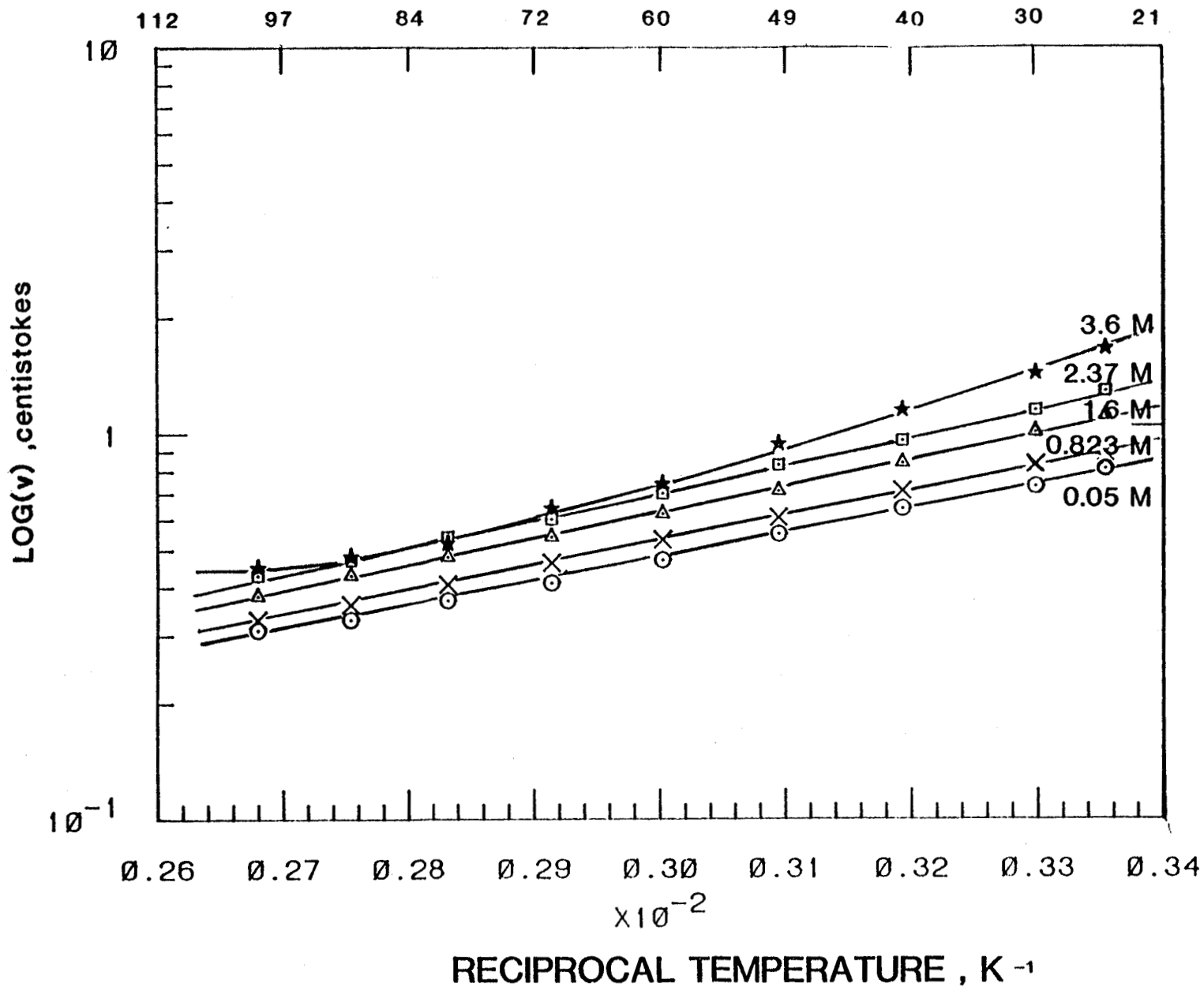
Figure 24 Plot of kinematic viscosity versus reciprocal temperature at dilute concentrations
