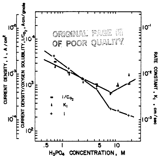
Fig. 7. Dependences of i , i/c_{O_2} , and k_1 for oxygen reduction at Pt on H_3PO_4 concentration at 25^\circ C .
