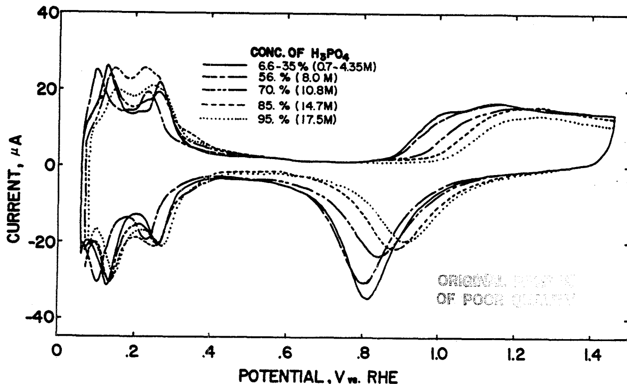
Fig. 1. Cyclic voltammograms on Pt at a scan rate of 50 mV/s in H_3PO_4 over the concentration range 6.6-95 w/o (weight percent) at 25°C.
