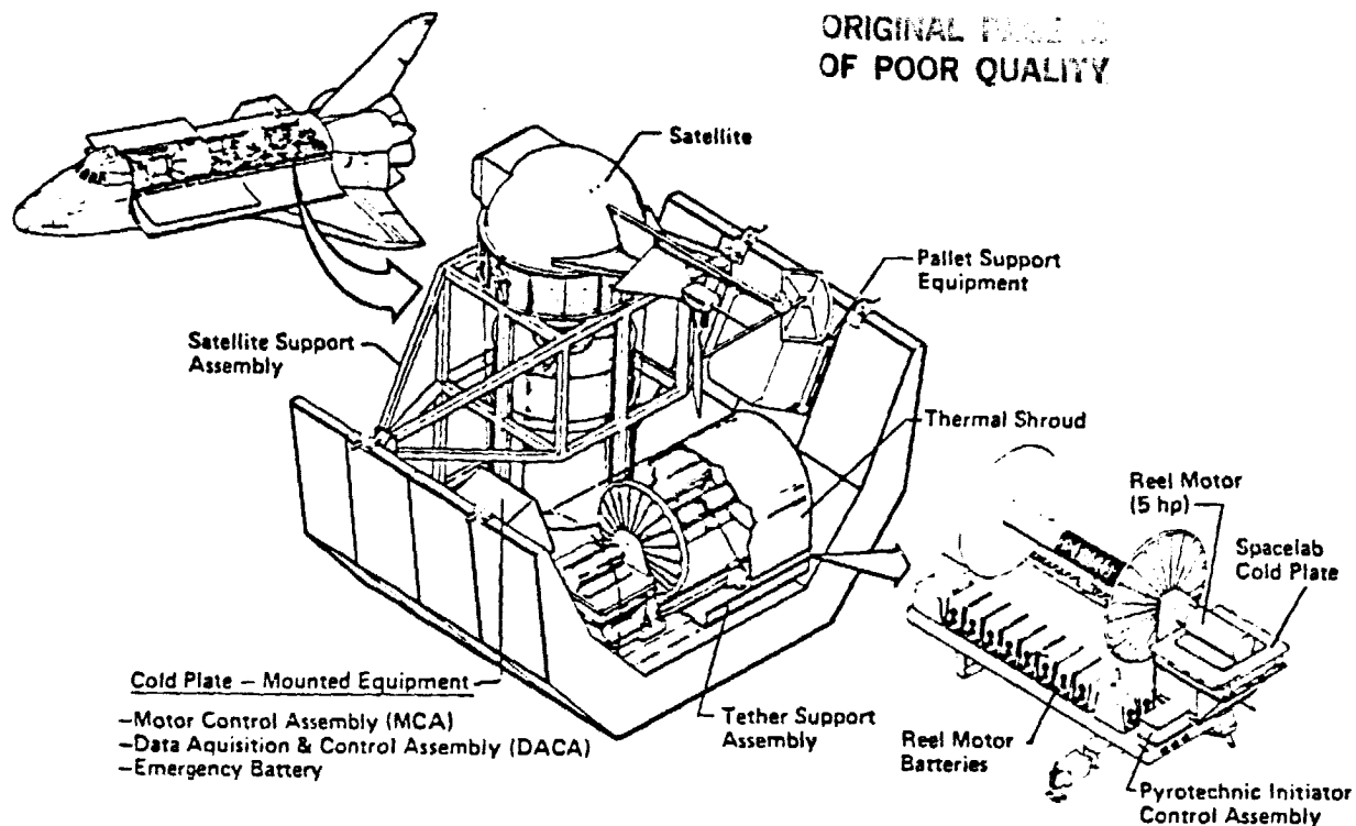
Figure 4. Design Overview - TSS/Pallet/Orbiter Interface
