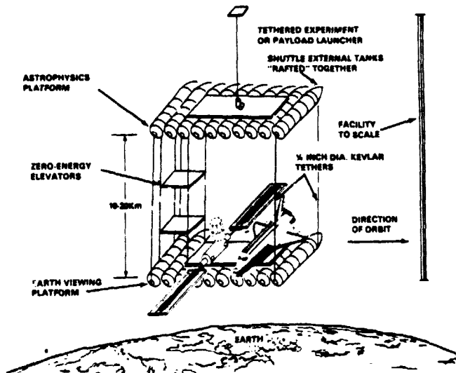
Figure 9. Passive Space Facility
