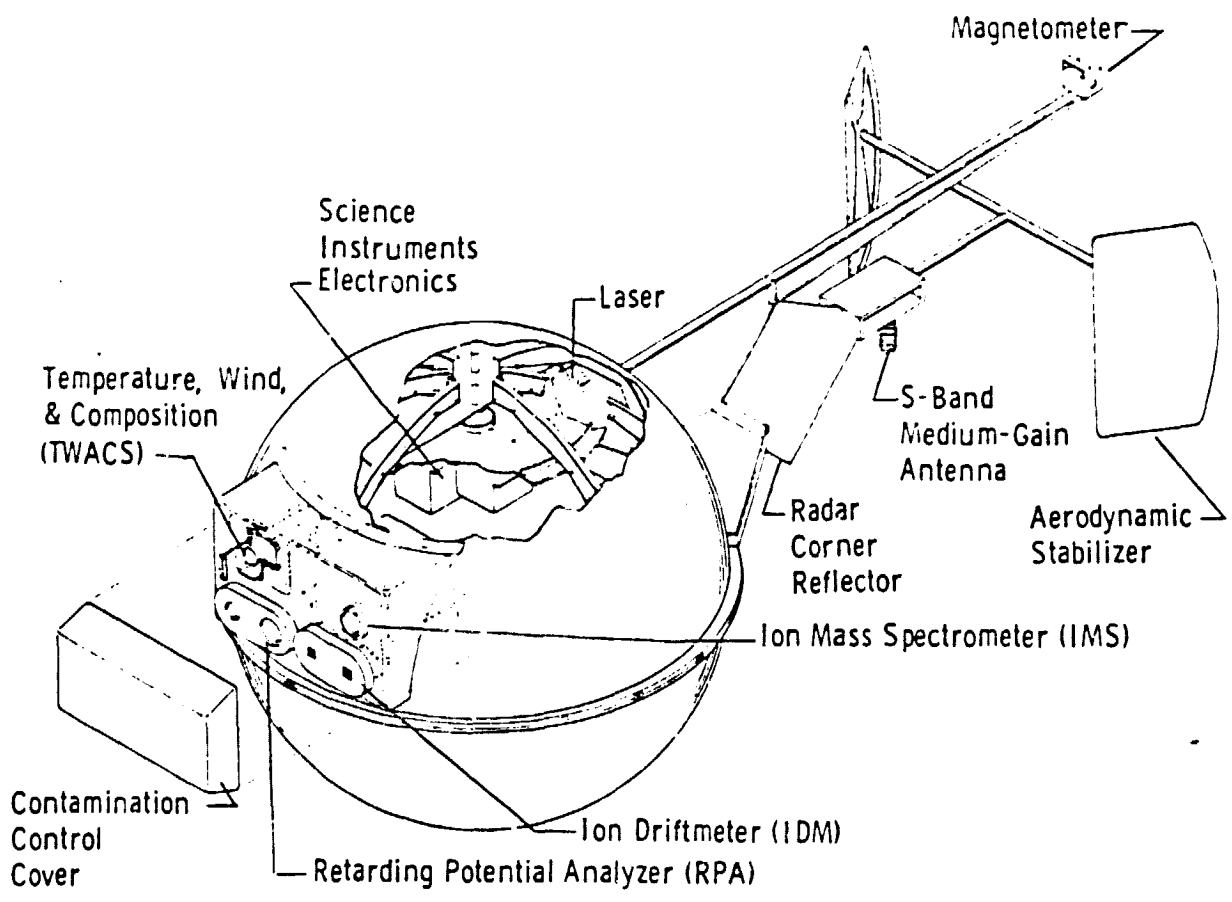
Figure 8. Design Overview - Atmospheric Probe Satellite
