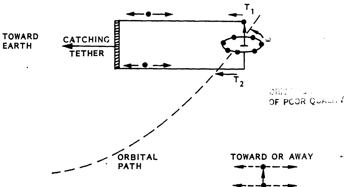
Figure 6. Tether Tension Force to Control Spin Axis
