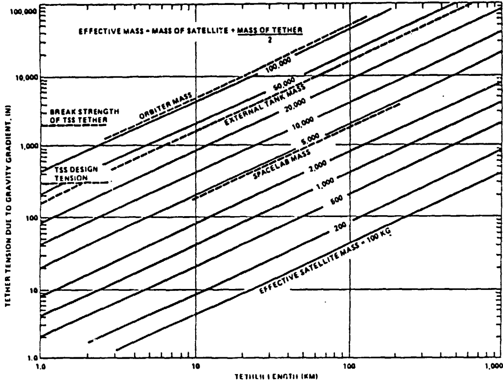
TETHER TENSION TO GRAVITY GRADIENT VERSUS TETHER LENGTH FROM CENTER OF GRAVITY AND EFFECTIVE SATELLITE MASS
