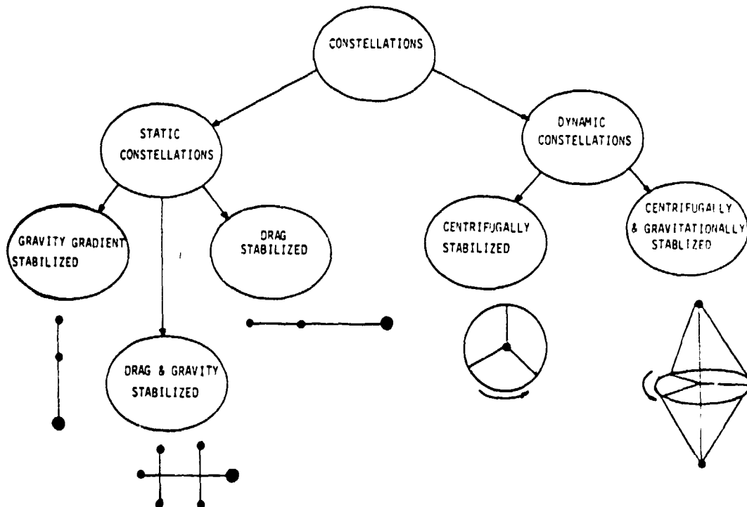
Figure 1. Tethered Constellations
