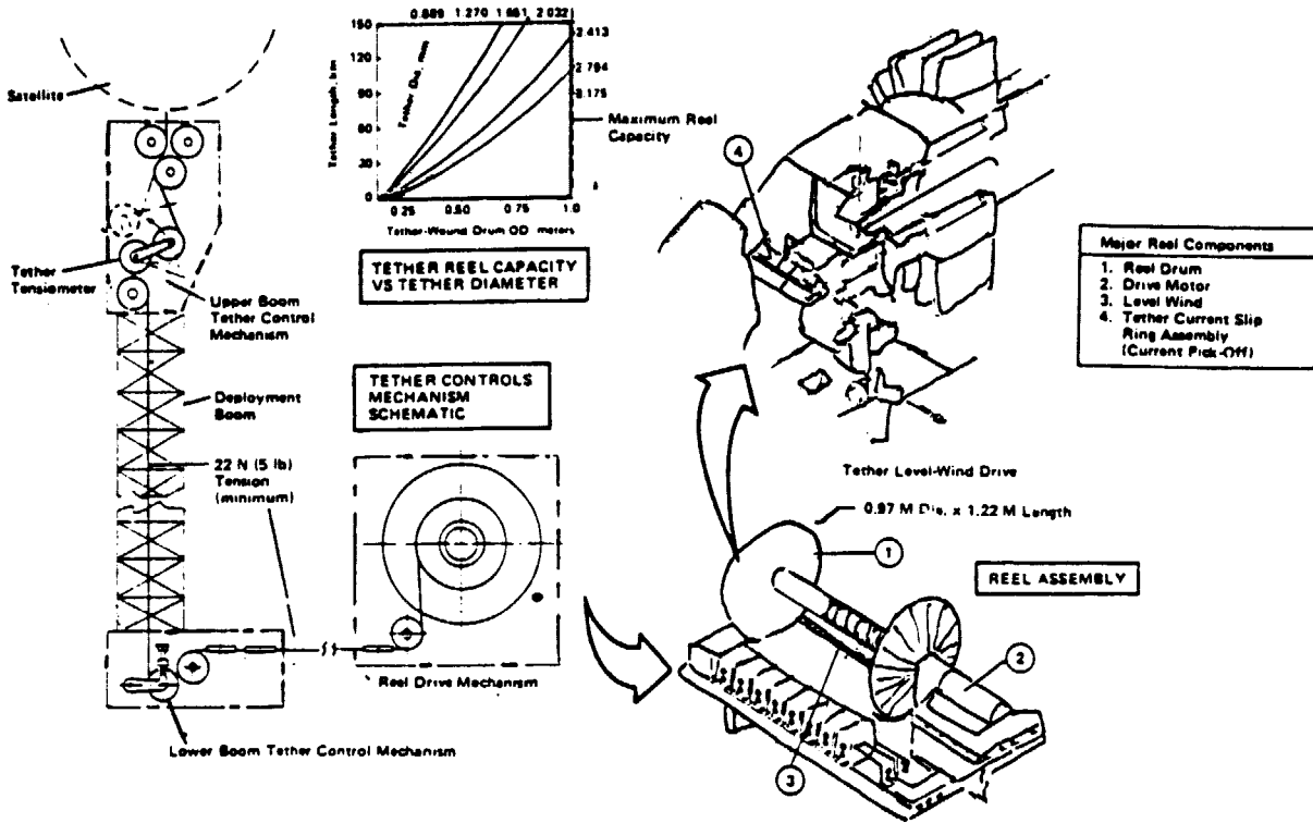
Figure 5. Design Overview - Tether Control Mechanisms
