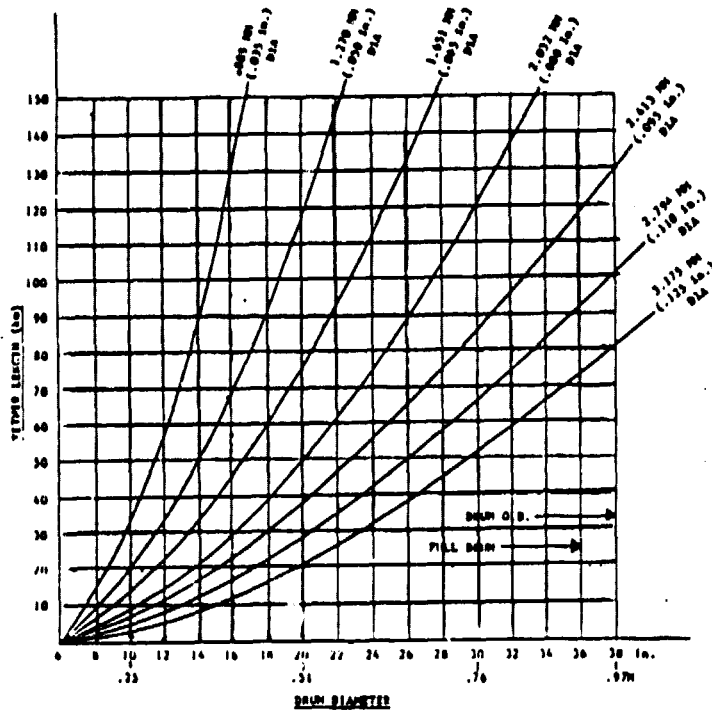
Tether Reel Capacity Vs Tether Diameter
