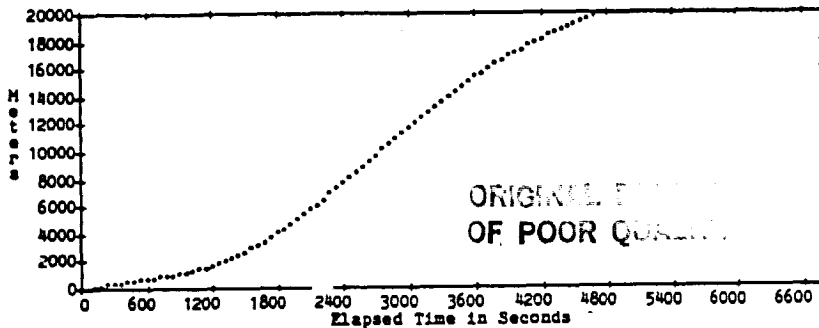
Figure 3. Deployed Tether Length vs Time
