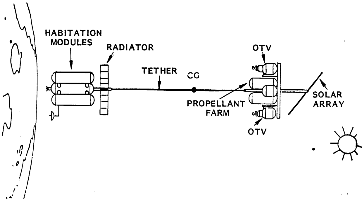
Figure 6. Tethered Orbital Refueling, Space Station
