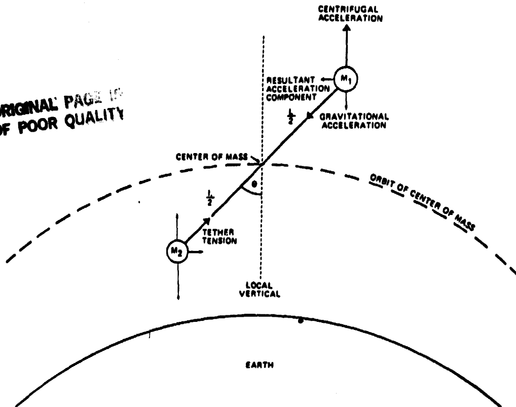
Figure 1. Stabilizing Forces Acting on Tethered Masses
