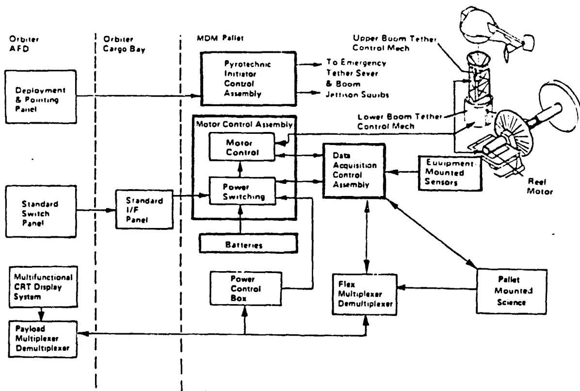
Figure 6. Design Overview - TSS Electrical Interfaces
