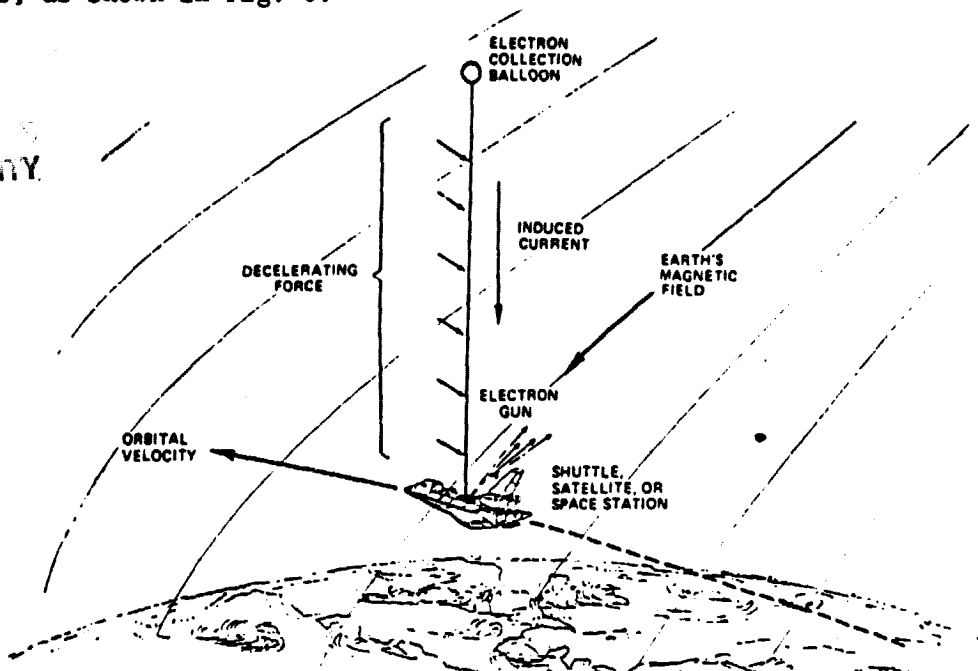
Figure 5. Tether As a Generator of High Power
