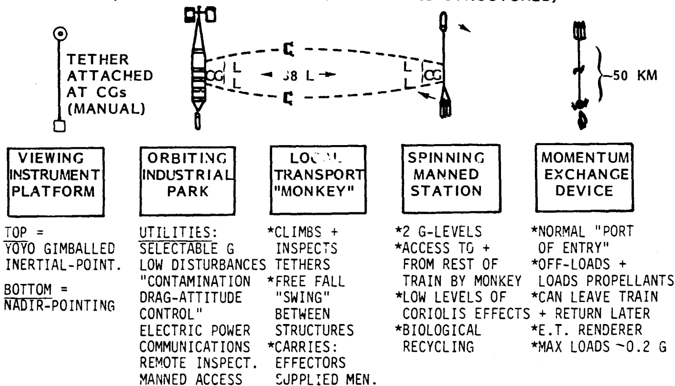
Figure 9. A Space Station "Train" or "Parade"
