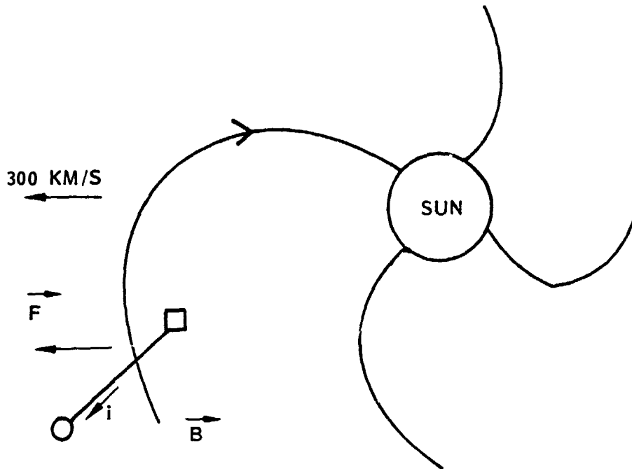
Figure 3. A Tether Thrust Generator for Interplanetary Missions
