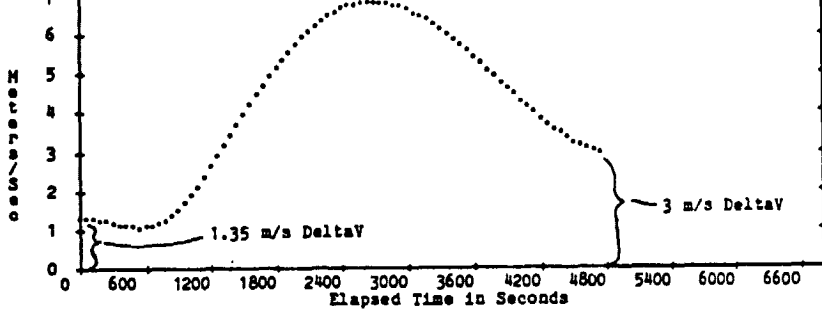
Figure 2. Tether Deployment Rate vs Time
