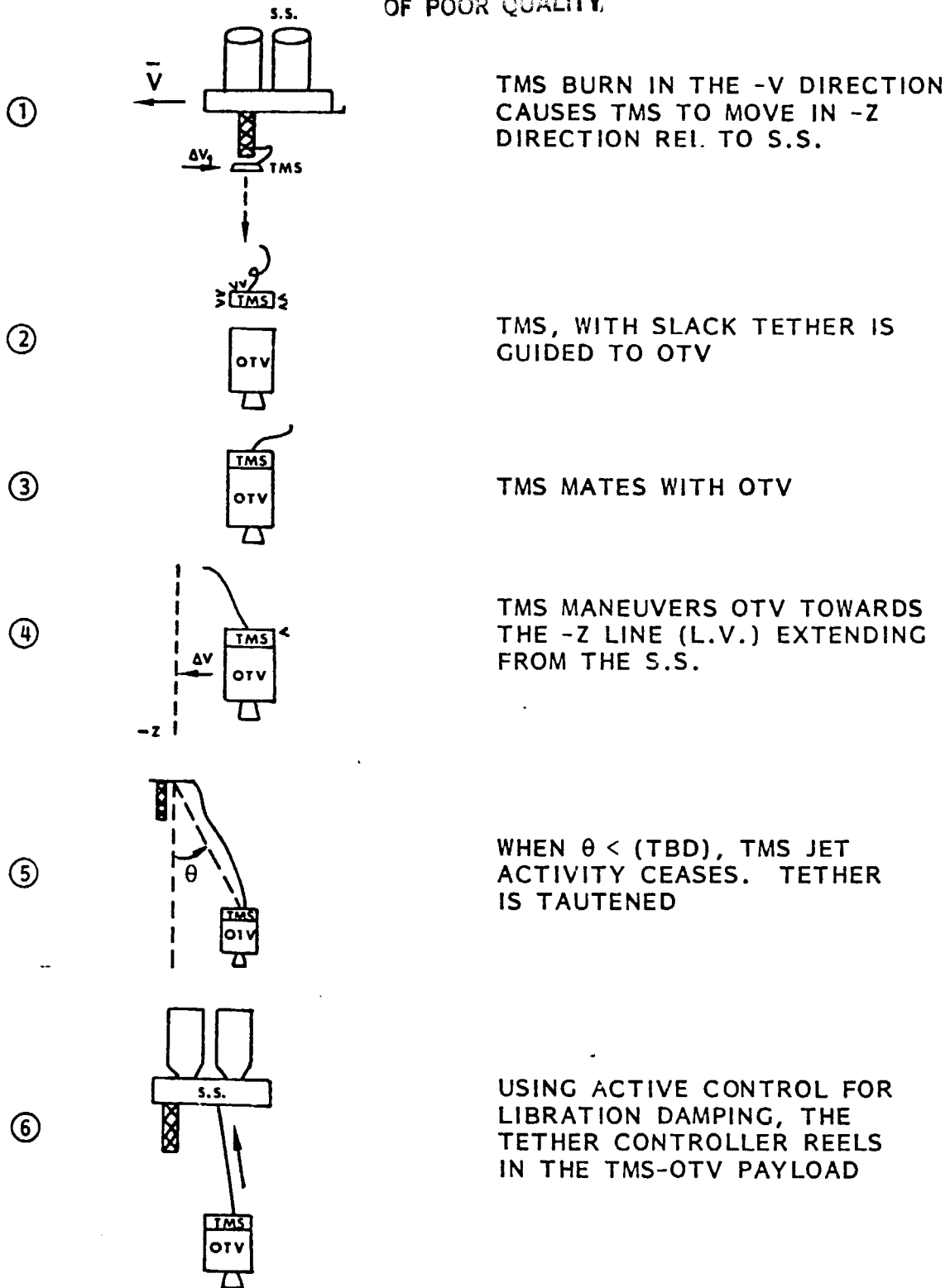
Figure 9. OTV Retrieval with Tethered TMS
