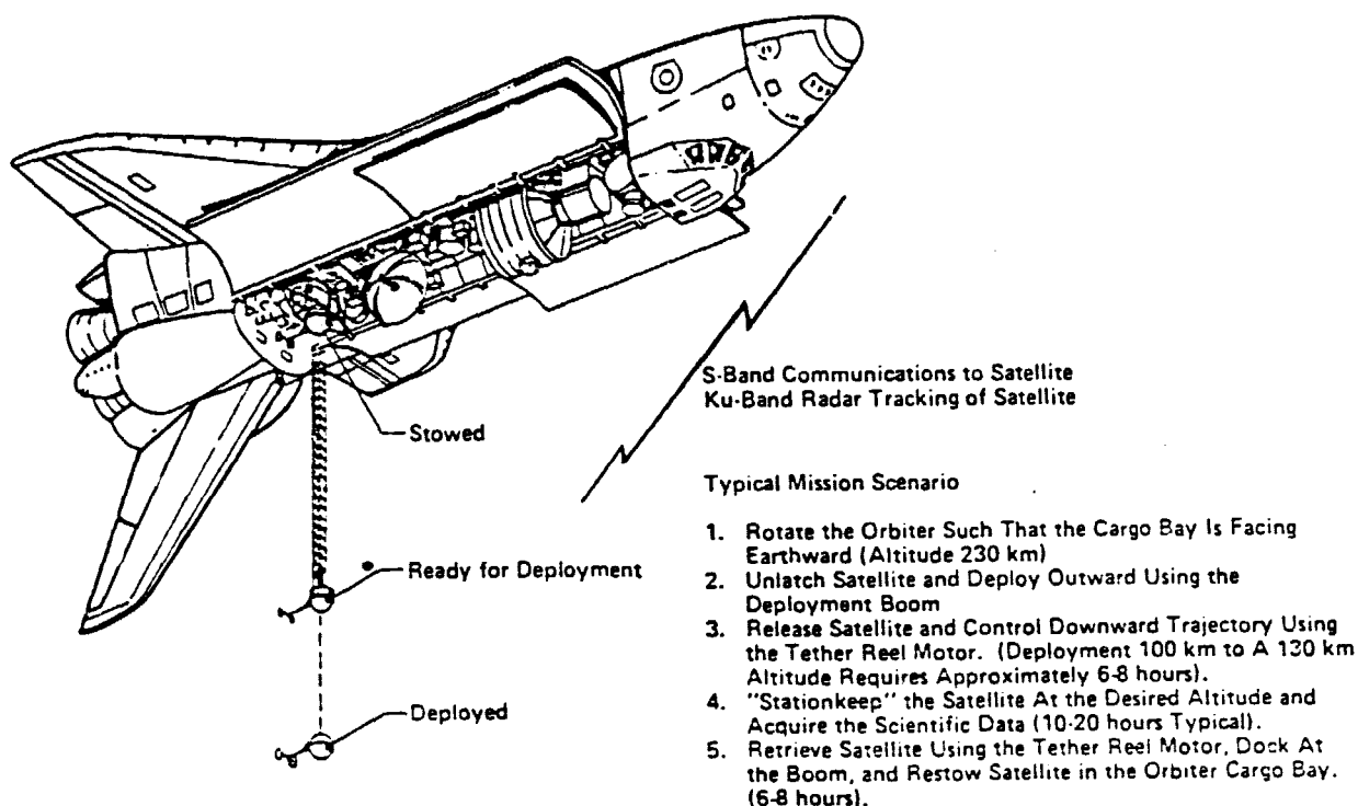
Figure 2. Design Overview - TSS Deployment Concept
