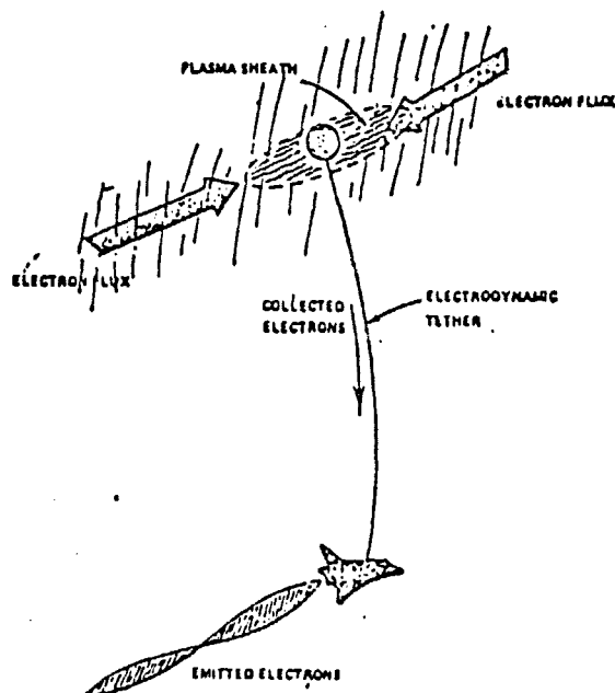
Figure 4. Basic Components of Electrodynamic Experiments with the Tethered Satellite System. The conducting tether is insulated along its length from the iono- spheric plasma so electrons can enter or leave the system only at the satellite and the Orbiter. Active electron emission occurs at the Orbiter, while electron collection takes place at the electrodynamic satellite.
