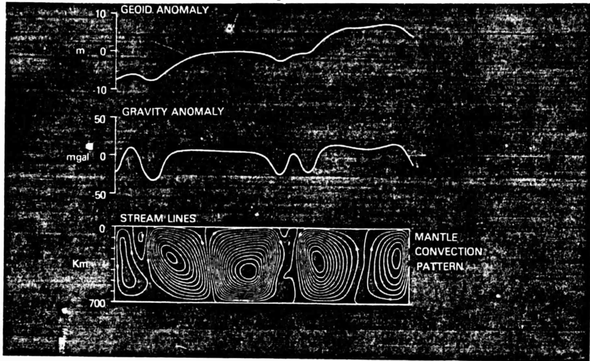
EXAMPLE OF GRAVITY AND GEOID ANOMALIES PRODUCED BY CONVECTION IN THE MANTLE (AFTER WATTS AND DALY, 1981)
