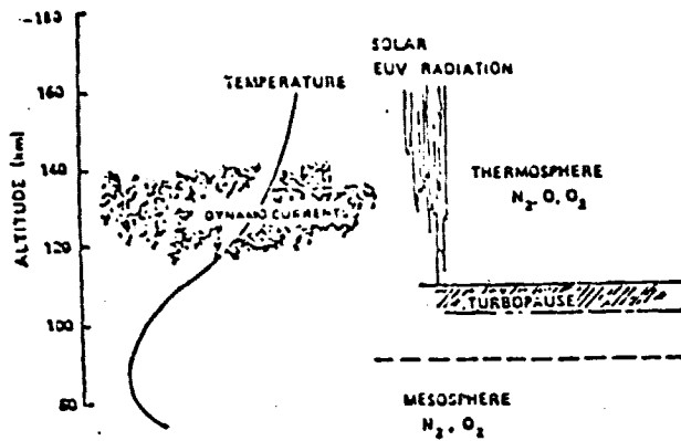
Figure 2. Upper Atmosphere Regions Showing Schematically the Transition from the Mesosphere to Lower Thermosphere, the Turbopause and the Zone Where Dynamo Currents are Present
