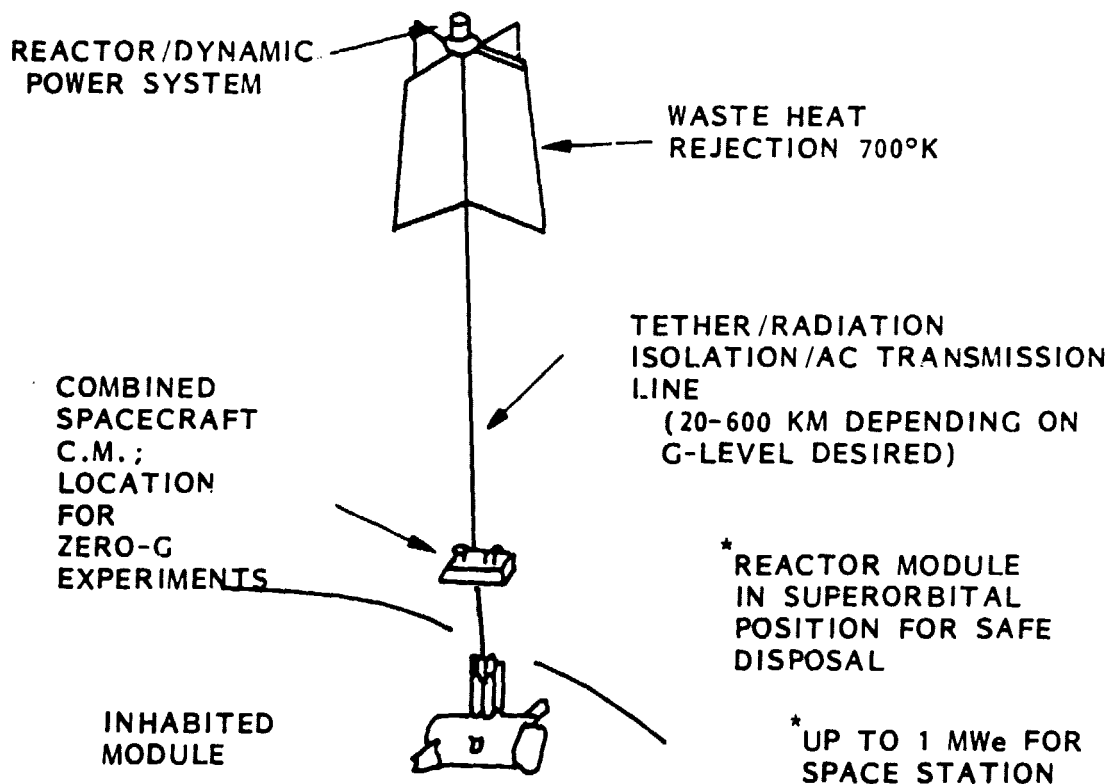
Figure 4. Nuclear Powered Tethered Platform (Gravity Gradient Stabilized)
