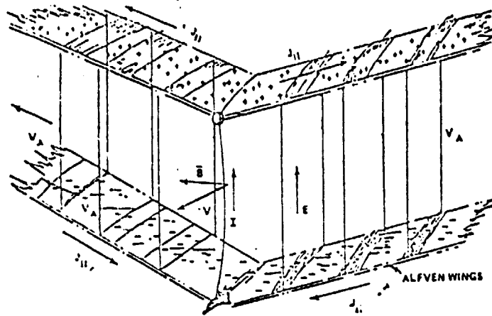
Figure 5. Schematic View of the Upper and Lower Current Sheets Which Spread Out from the Electrodynamic Tether System. The periodic darkened regions represent the outward propagation of Alfvén waves along the magnetic field. There is a net positive charge excess on the top wing and a net negative charge density on the lower wing.
