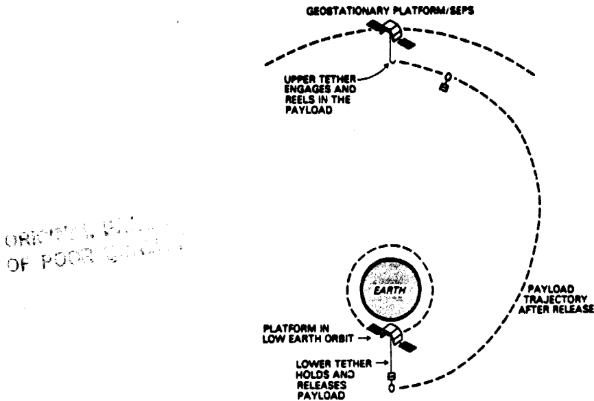
Figure 12. Two-Piece Tether "Elevator"
