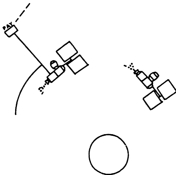
Figure 12. Using Station-Based Tether to Assist GEO or Deep Space Launch, Plus Electric Propulsion to Restore Orbit
