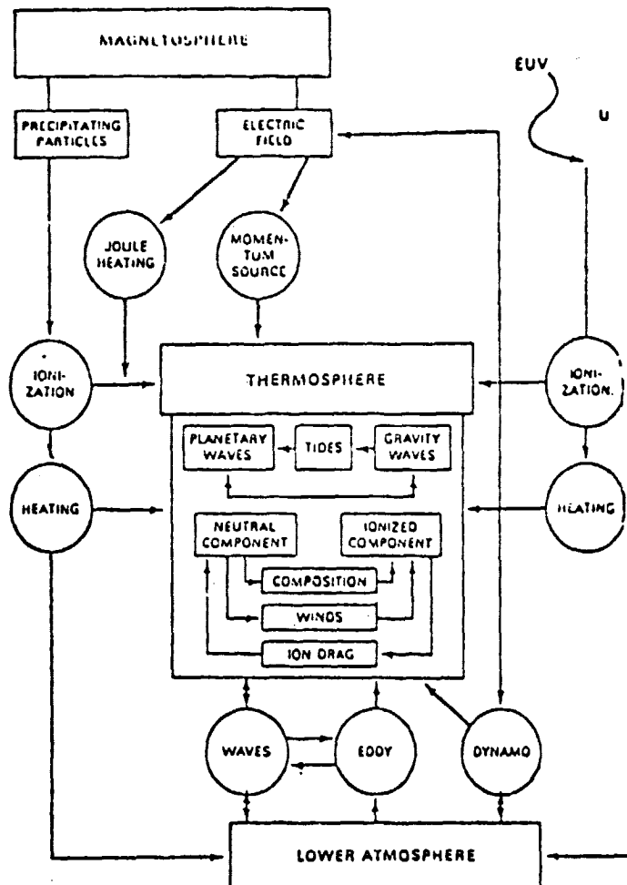
Figure 1. Schematic Diagram Illustrating the Important Processes Linking the Lower Atmosphere, Thermosphere, and Magnetosphere. Within the thermosphere a variety of waveforms are generated ranging from planetary scale to gravity waves.
