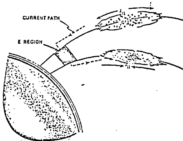
Figure 6. Illustrating the Magnetic Field-Aligned Currents Which Are Caused in the Ionosphere by the Transfer of Electrons from the TSS Satellite to the Shuttle. The net charge imbalance spreads along the magnetic field until the perpendicular resistivity is sufficiently high to permit transverse currents to connect the two magnetic flux shells.
