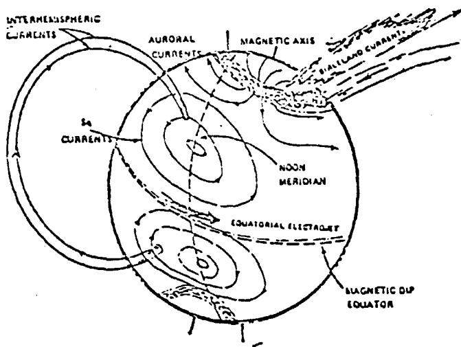
Figure 3. Schematic View of the Global System of Upper Atmospheric Currents Including Wind-Driven Currents at Mid-Latitudes, High Latitude Auroral Currents, and Inter-Hemispheric Field-Aligned Currents
