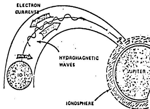
Figure 7. Schematic View of the Interaction of Io with the Rapidly Rotating Jovian Ionosphere. Large magnetic field-aligned currents connect to the Jovian ionosphere, propagating at the Alfvén speed in the moving medium.
