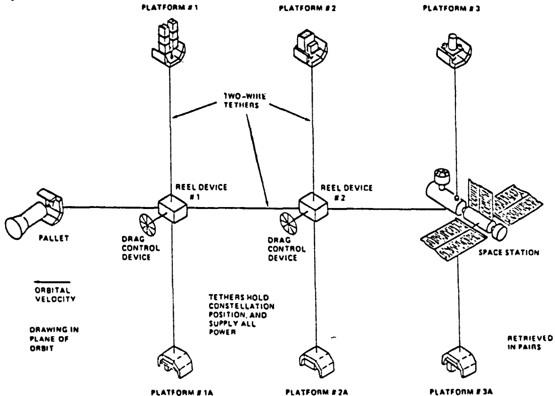
Figure 10. Two-Dimensional Tethered Constellation
