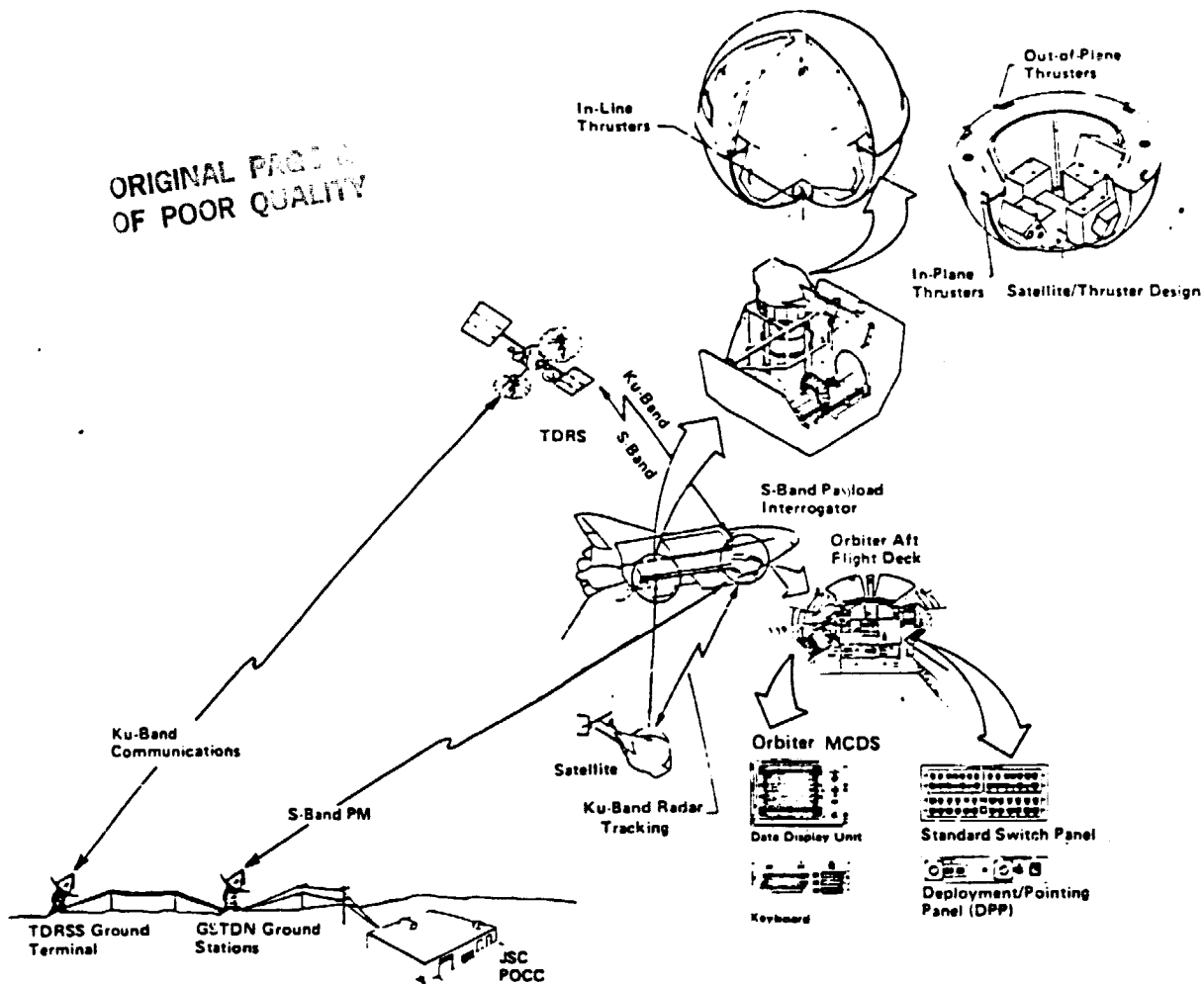
Figure 1. Design Overview - TSS/Orbiter/Ground Interfaces
