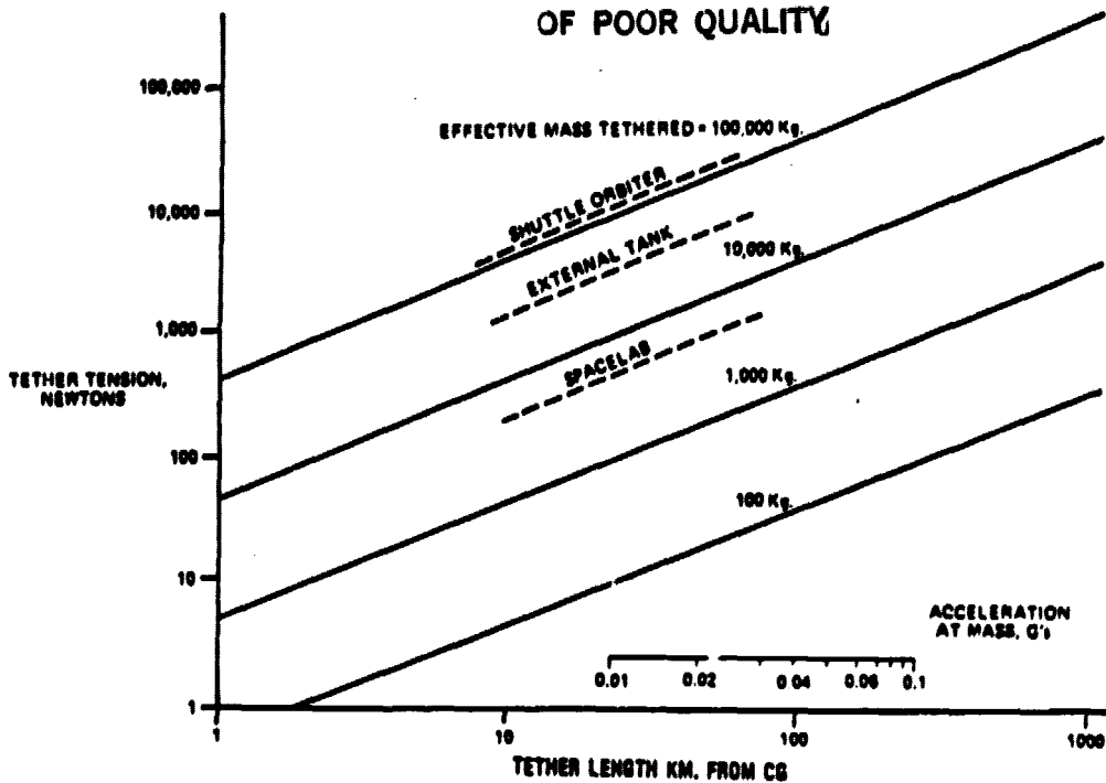
Figure 2. "Artificial Gravity" at Tethered Masses
