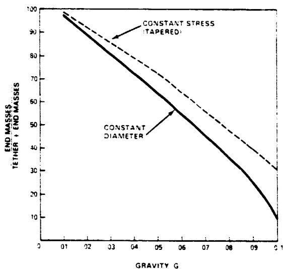
Figure 7. Mass of Tether Grows with Desired Gravity Level
