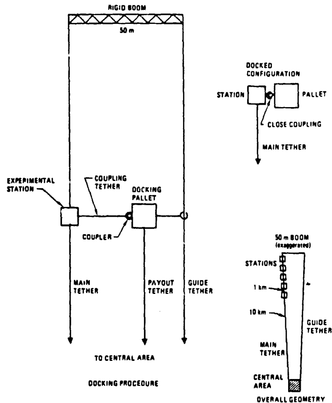
Transferring Pallet to Experimental Station
