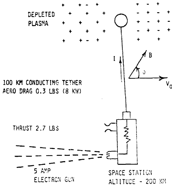
TETHER POWER GENERATOR
