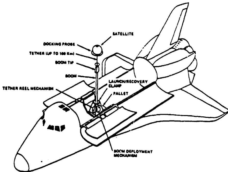
SHUTTLE/TETHERED SATELLITE SYSTEM
