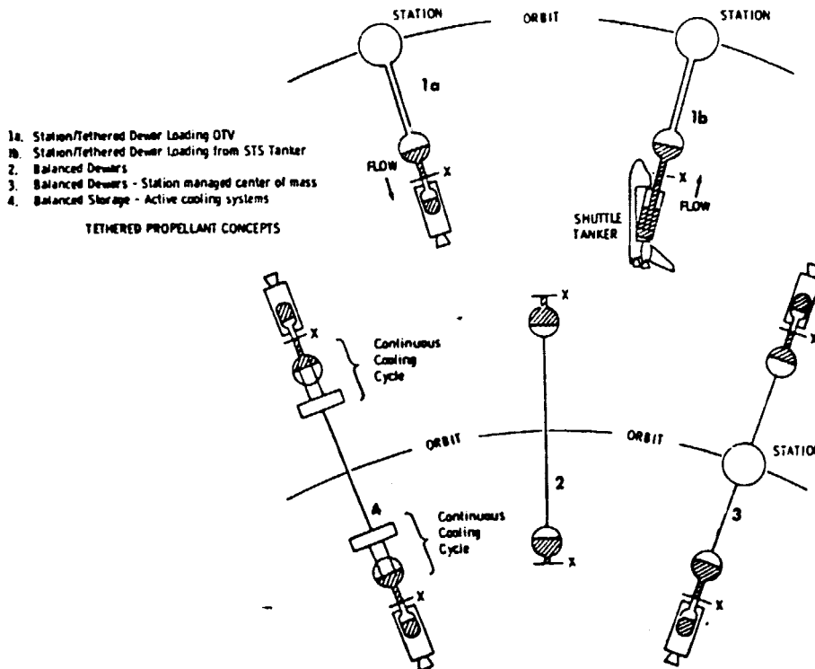
Figure 7. Tethered Propellant Concepts
