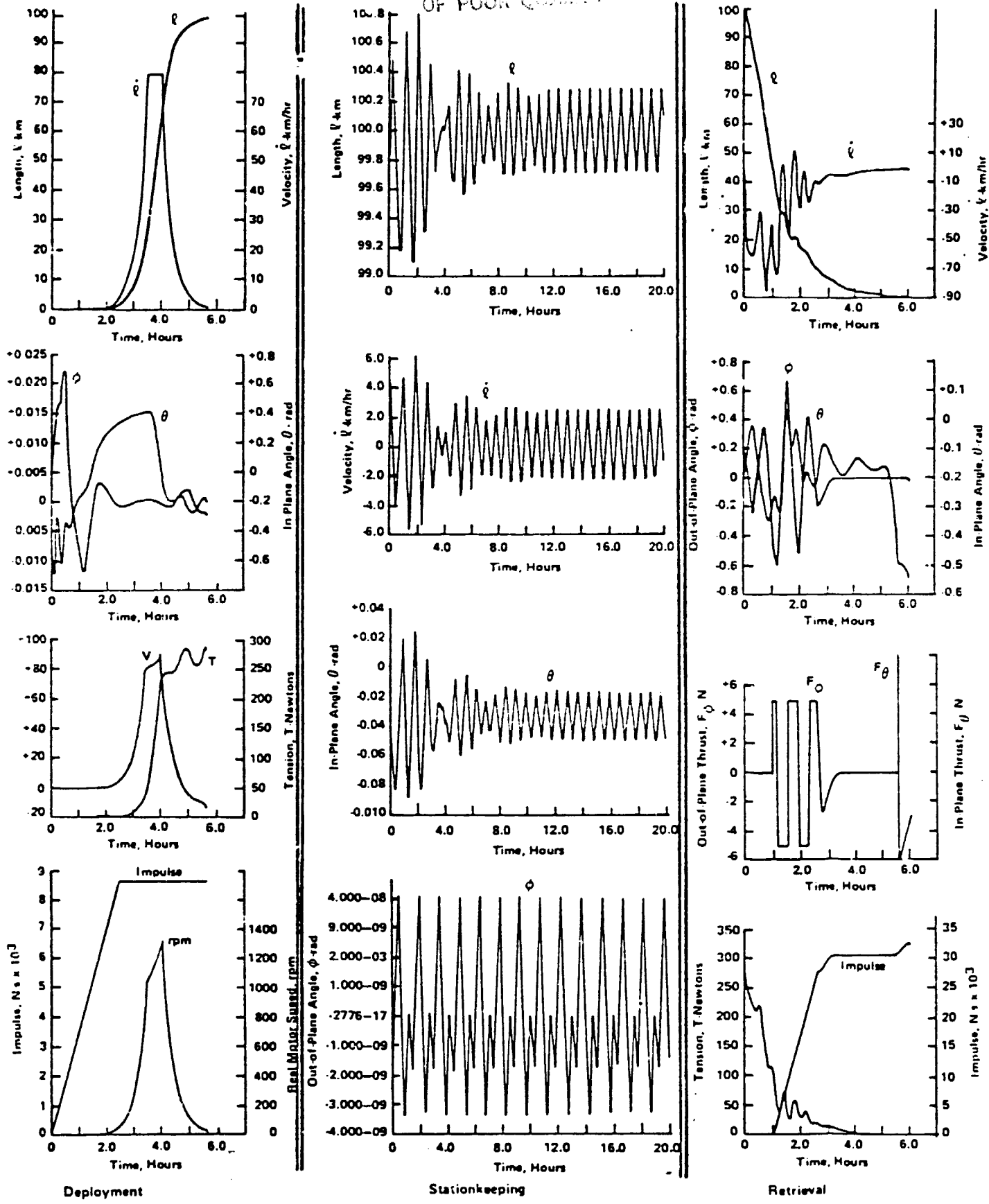
Figure 3. Typical Satellite Deployment, Stationkeeping, and Retrieval Profiles (130 km Deployment Altitude)
