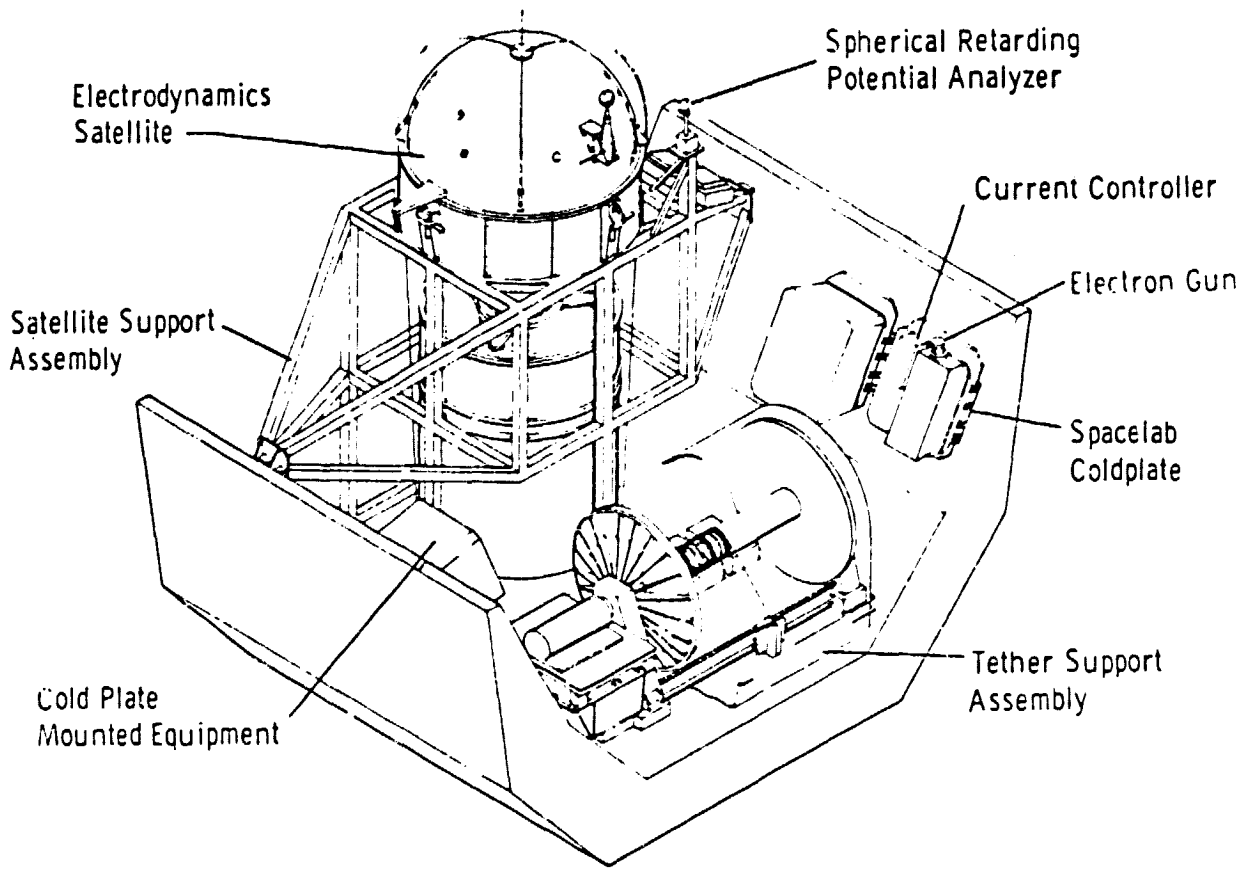
Figure 7. Design Overview - Electrodynamic Satellite
