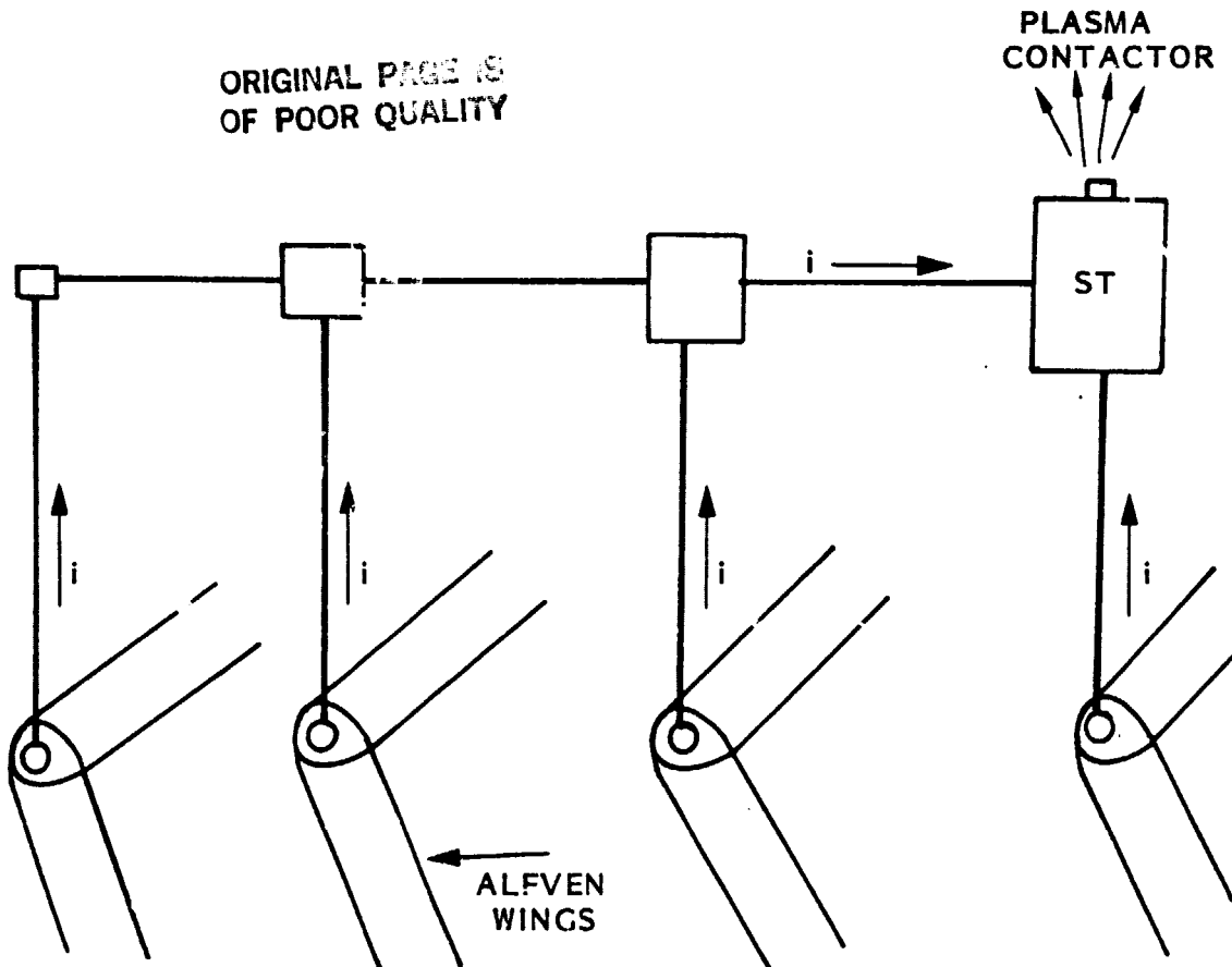
Figure 1. A Parallel Tether Current Generator
