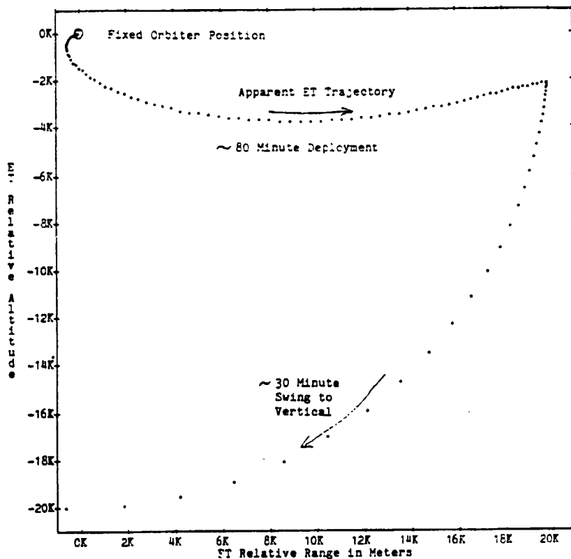
Figure 1. ET Position Relative To Orbiter at One-Minute Intervals
