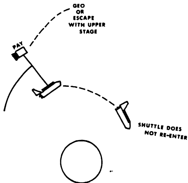
Figure 10. Using Shuttle-Based Tether to Assist Launch of Upper Stage for GEO or Interplanetary Orbits
