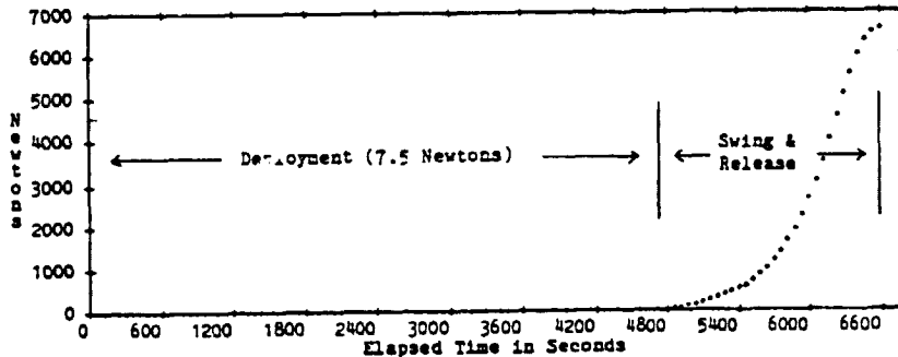
Figure 4. Tether Tension vs Time
