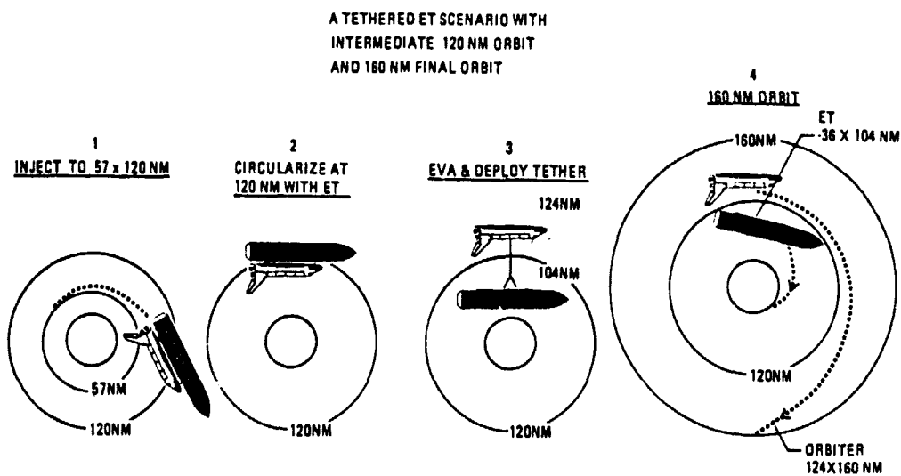
Figure 3. Downward Release of ET from Shuttle Orbit
