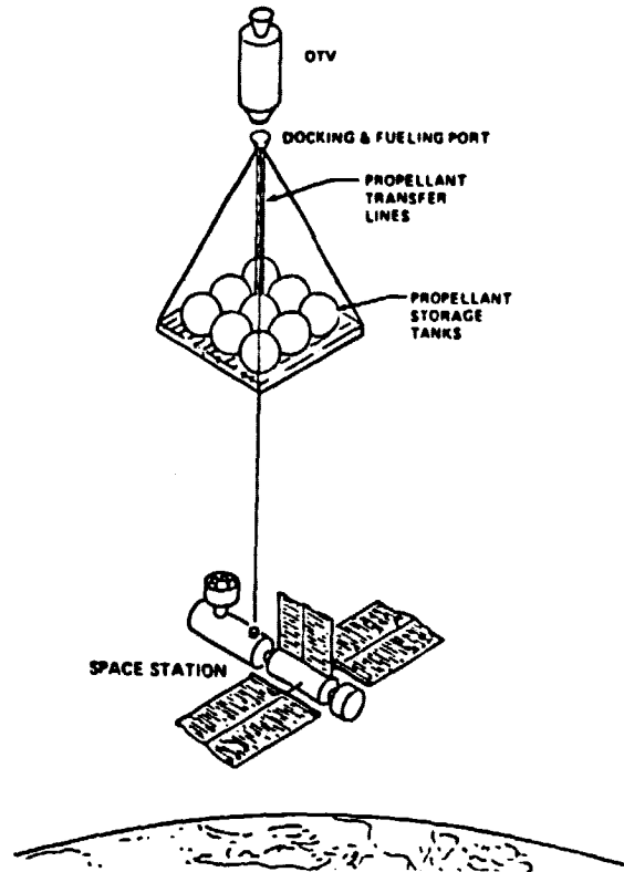
Figure 8. Cryogenic Propellant Storage and Transfer Platform
