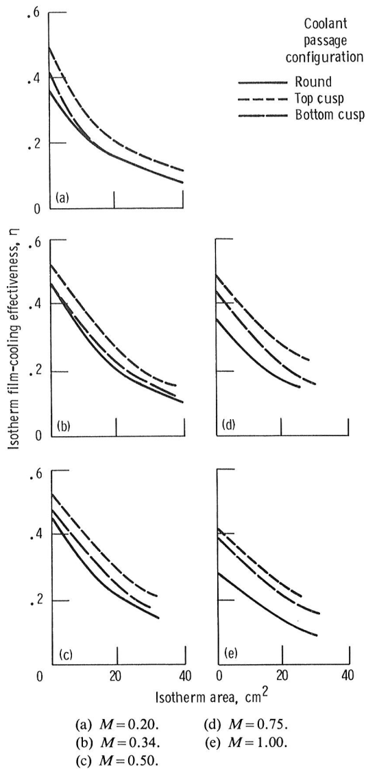
Figure 22.—Comparison of film-cooling coverage data for free-stream velocity of 45.0 m/s.
