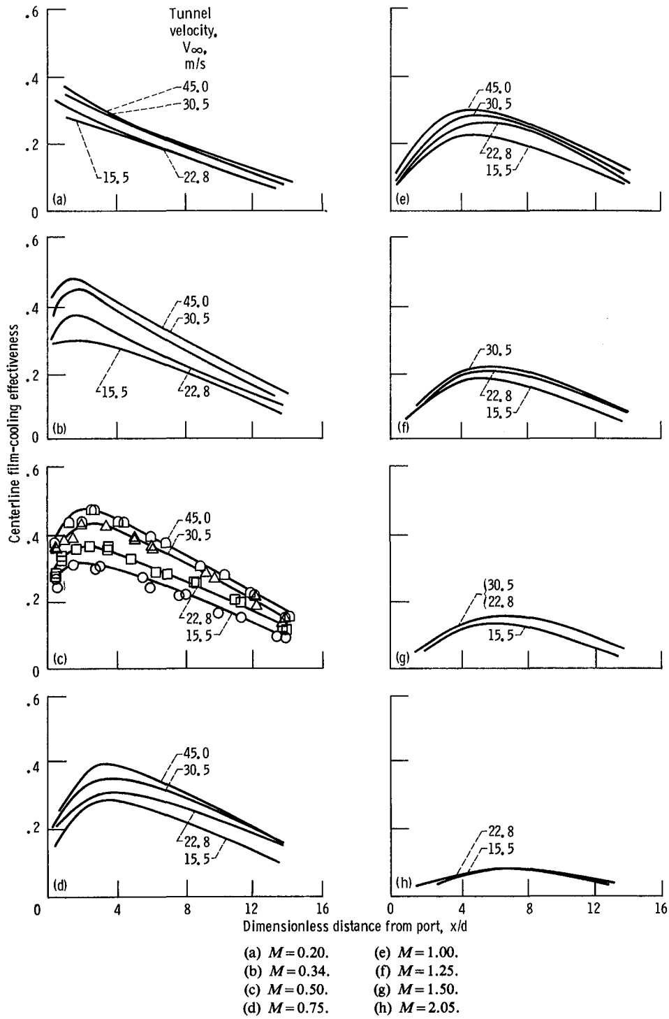
Figure 9.—Basic round coolant passage data.
