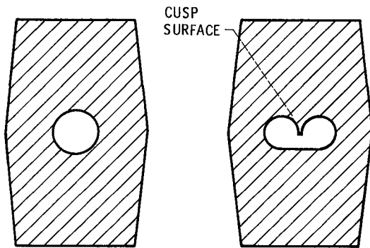
(a) ROUND STANDARD HOLE VORTEX GENERATING HOLE
