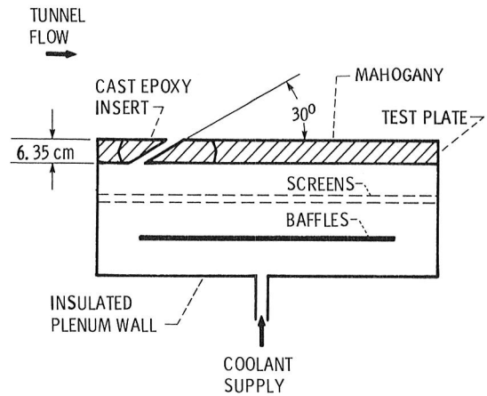
Figure 6.—Test plate and coolant-supply plenum.
