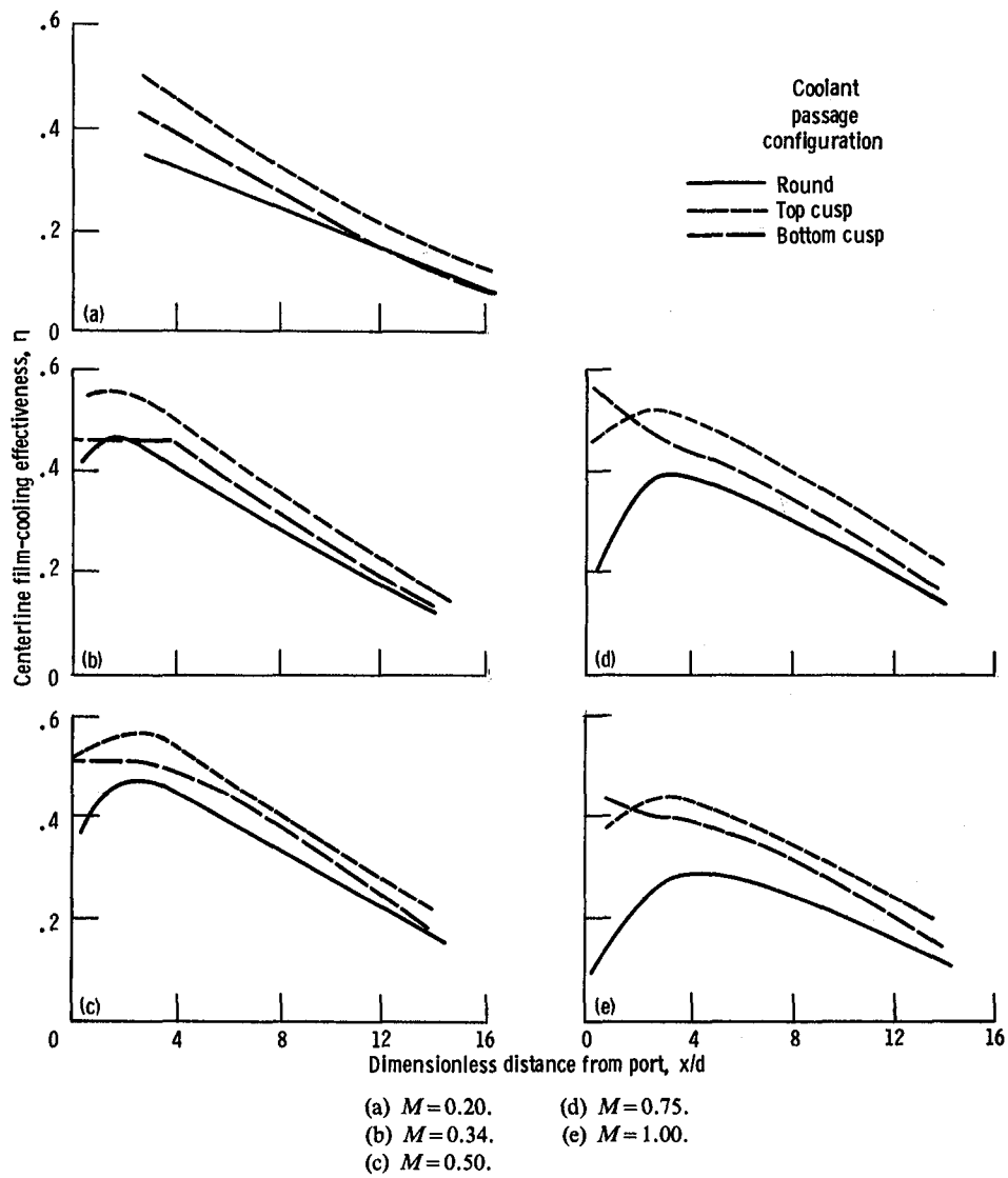
Figure 15.—Comparison of centerline film-cooling effectiveness distributions for free-stream velocity of 45.0 m/s.
