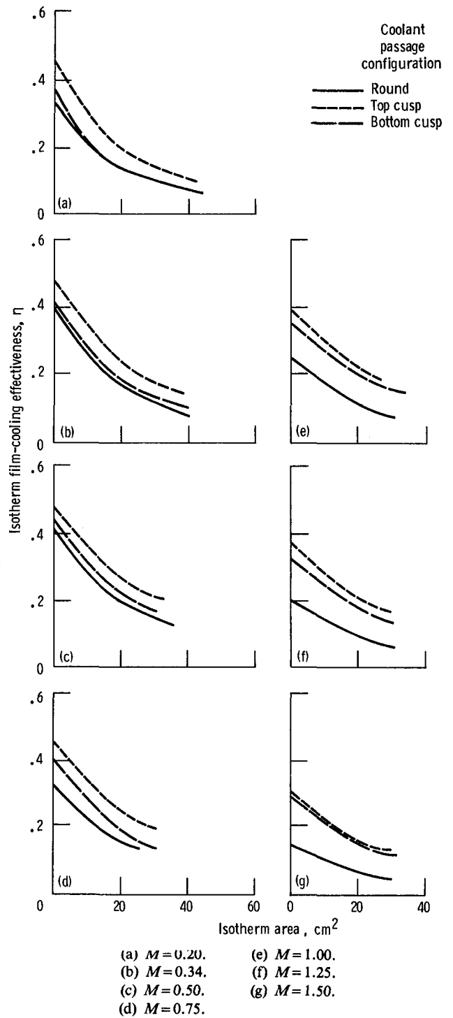
Figure 21.—Comparison of film-cooling coverage data for free-stream velocity of 30.5 m/s.
