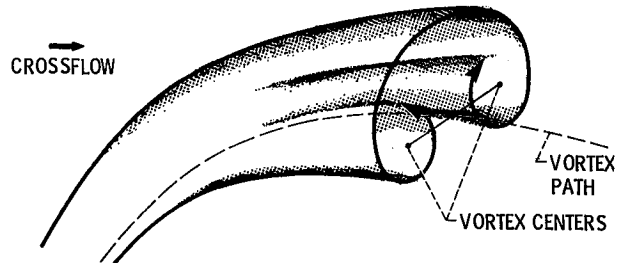
Figure 2.—Counterrotating vortex pair structure within the jet induced by the crossflow.
