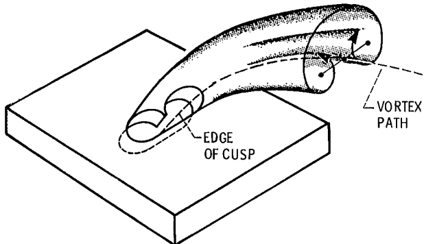
(a) Coolant flow passage cross sections. (b) Counterrotating vortex-generating coolant passage.
