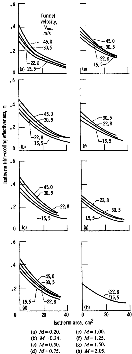
Figure 18.—Basic bottom-cusp film-cooling coverage data.
