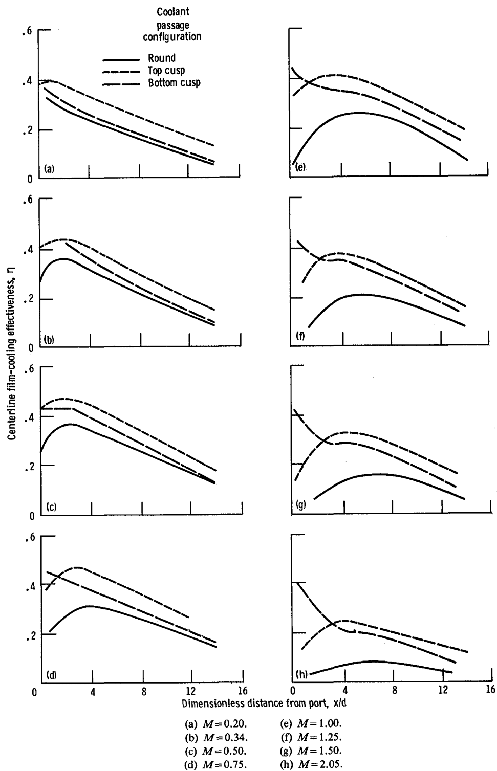
Figure 13.—Comparison of centerline film-cooling effectiveness distributions for free-stream velocity of 22.8 m/s.
