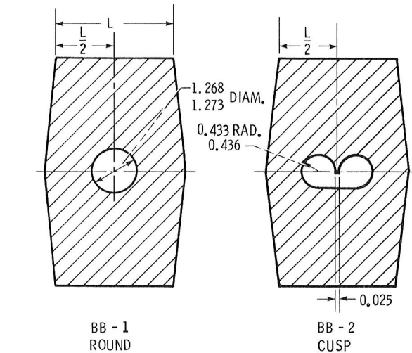
Figure 5.—Design details of passage cross sections. (All dimensions in centimeters.)
