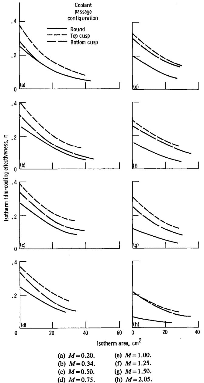
Figure 19.—Film-cooling effectiveness as function of isotherm area for free-stream velocity of 15.5 m/sec.
