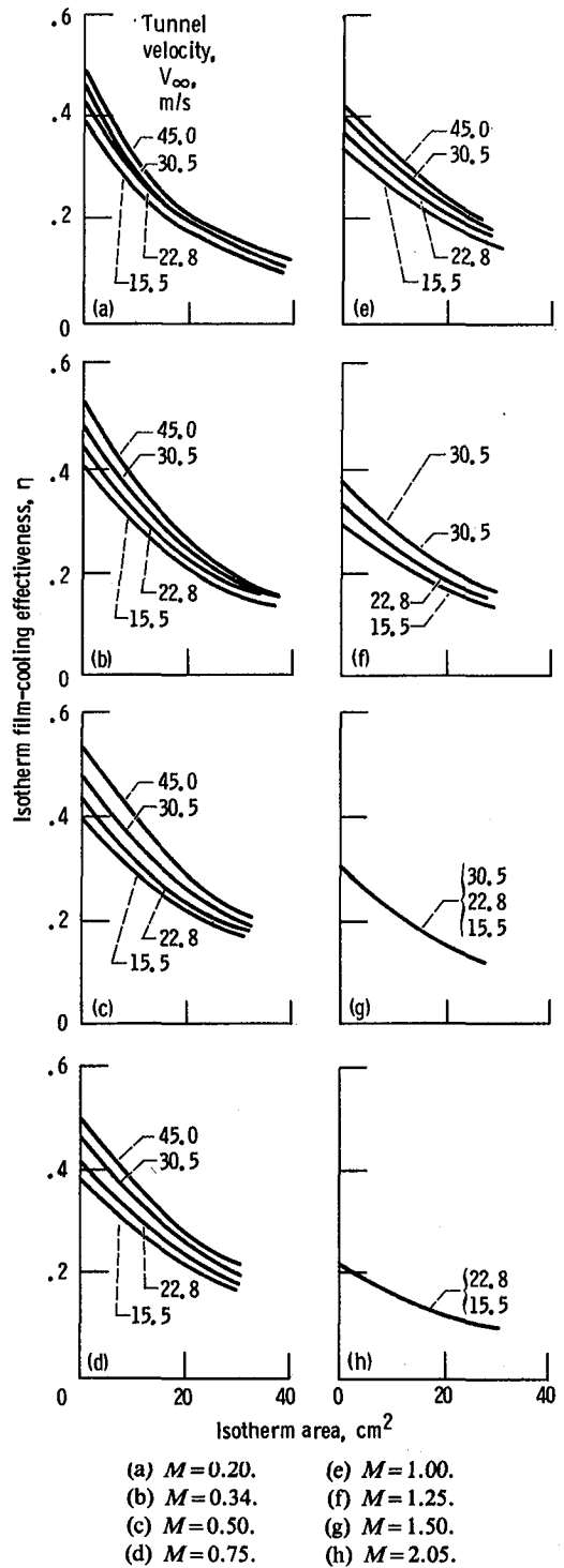
Figure 17.—Basic top-cusp film-cooling coverage data.
