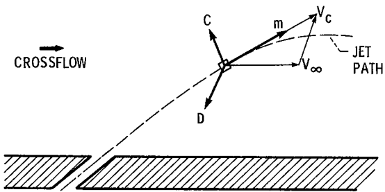
Figure 1.—Inclined jet in crossflow showing forces on a control element.
