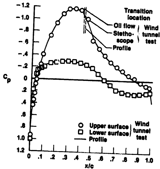
Figure 6. Transition location and pressure coefficient comparison for FX66-4II-182 airfoil in the wind tunnel at Re = 1.5 \times 10^6 , \alpha = 0^\circ , and C_L \approx 0.4 ; low-speed airfoil program at Re = 1.5 \times 10^6 , \alpha = 7^\circ , and C_L = 0.368 .
