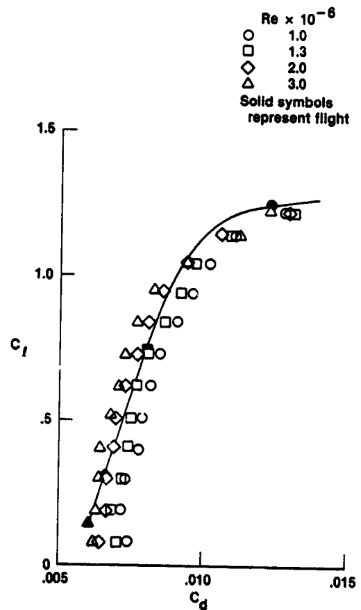
Figure 12. A comparison of computed and flight data (ref. 4) for the flight airfoil with 6° flap deflection.
