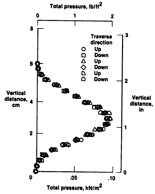
Figure 4. Typical total pressure wake profiles. Six consecutive wakes; flap deflection = 0°; velocity = 44.0 knots; q_0 = 0.31 \text{ kN/m}^2 (6.5 lb/ft 2 ). (From ref. 4.)
