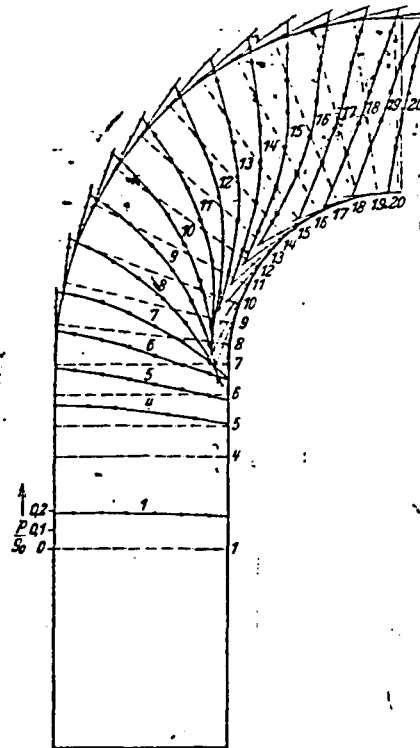
Figure 6. The static pressure on the measurement plate.
