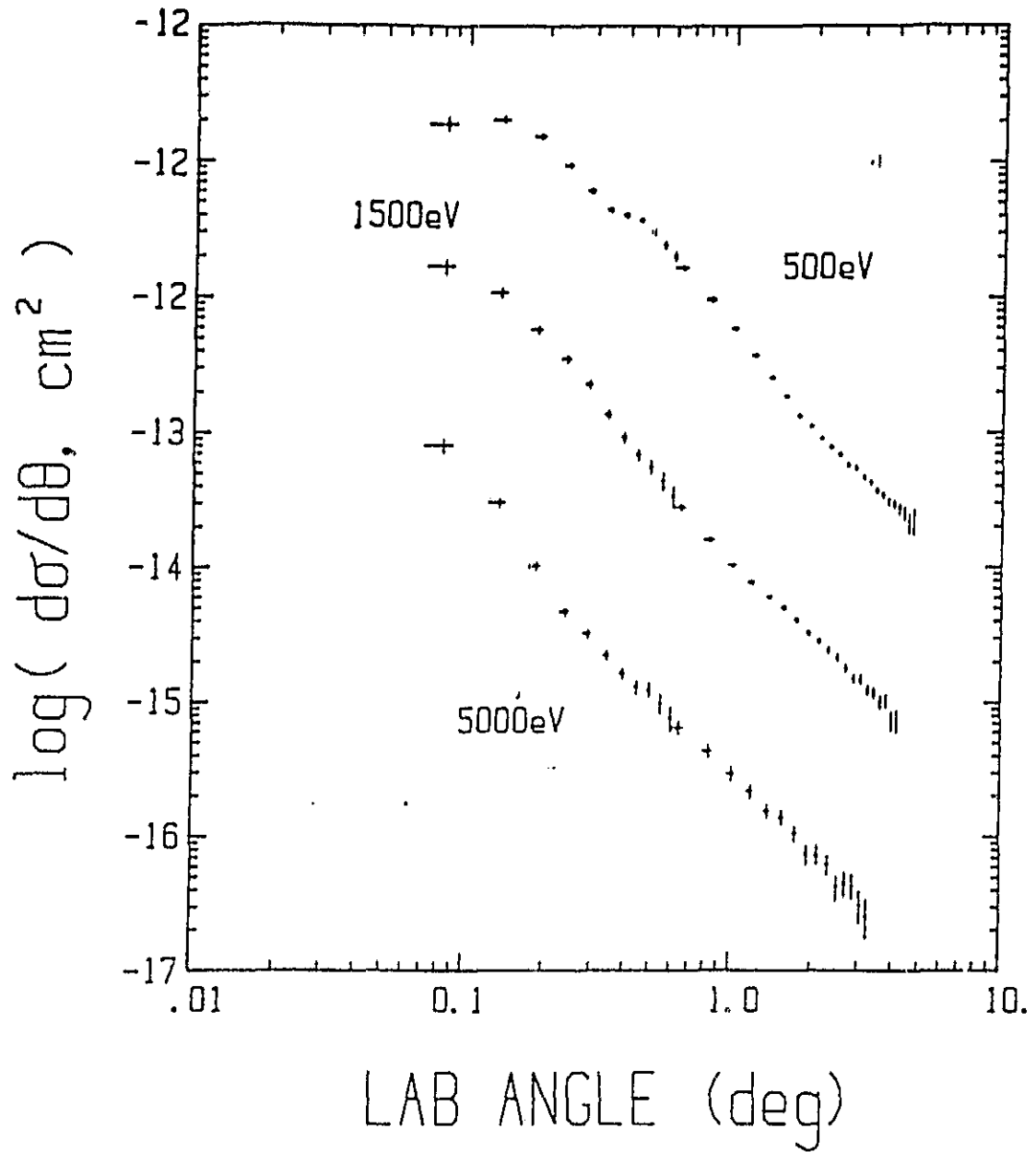
FIGURE 6 DIFFERENTIAL CROSS SECTIONS FOR COLLISIONS OF HYDROGEN WITH HELIUM,
