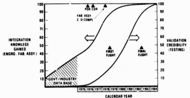
Figure 5. HiMAT Learning and Validation Experience
