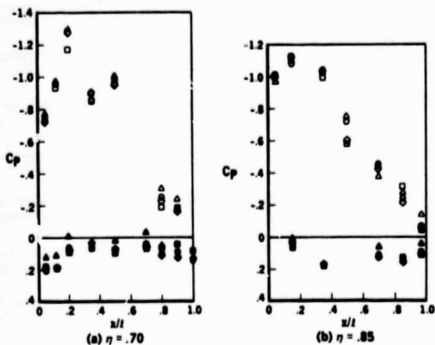
Figure 20. Wing Pressure Distribution for Maneuvering Flight at Mach 0.9, \bar{q} = 440 lb/sq ft, \alpha = 10^\circ
