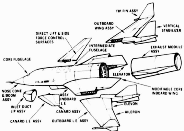
Figure 9. Modularity Features
