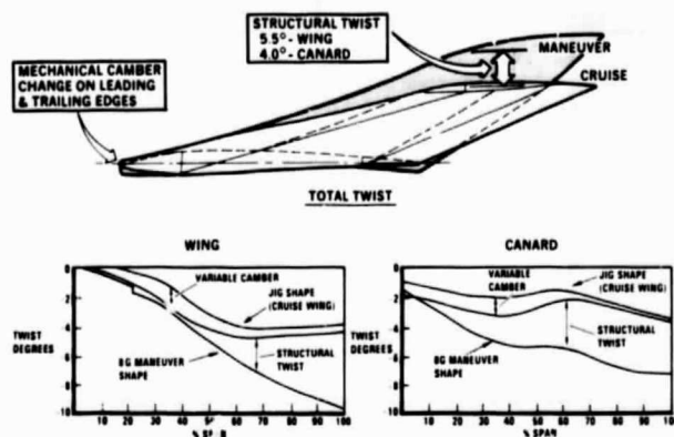
Figure 7. Aeroelastic Tailoring
