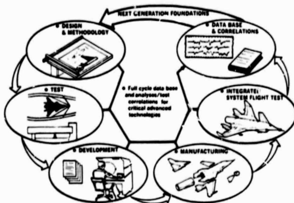
Figure 22. HiMAT Program Cycle
