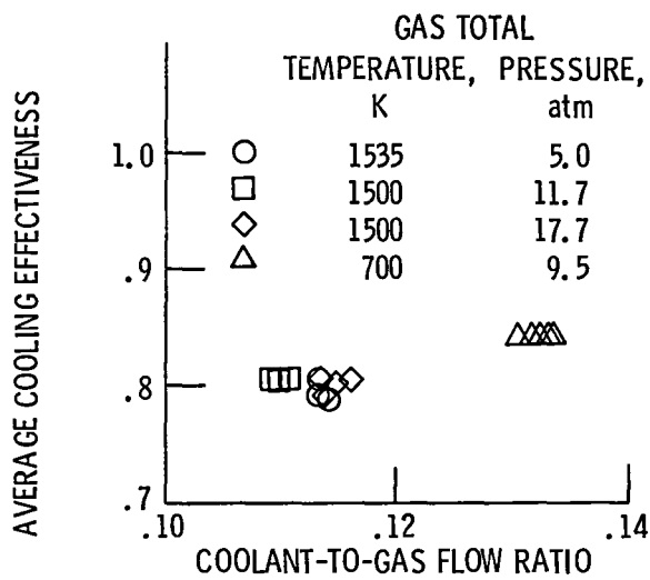
(b) Repeatability of HSF demonstrated by repetitive data taken at a specified set-point.
