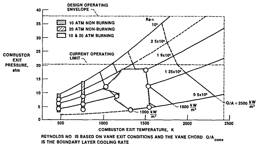
Figure 6. - Cascade rig simulation of real engine operating conditions.
