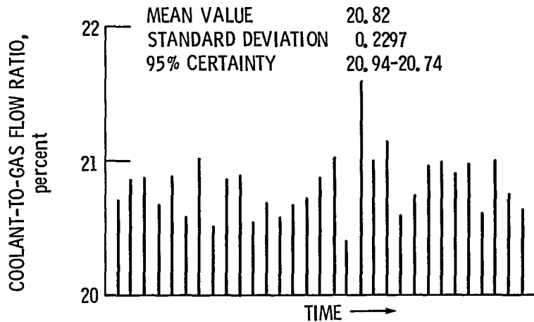
(a) Time history of the coolant-to-gas flow parameter.
