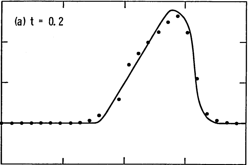
Figure 2.2 Godunov's method
