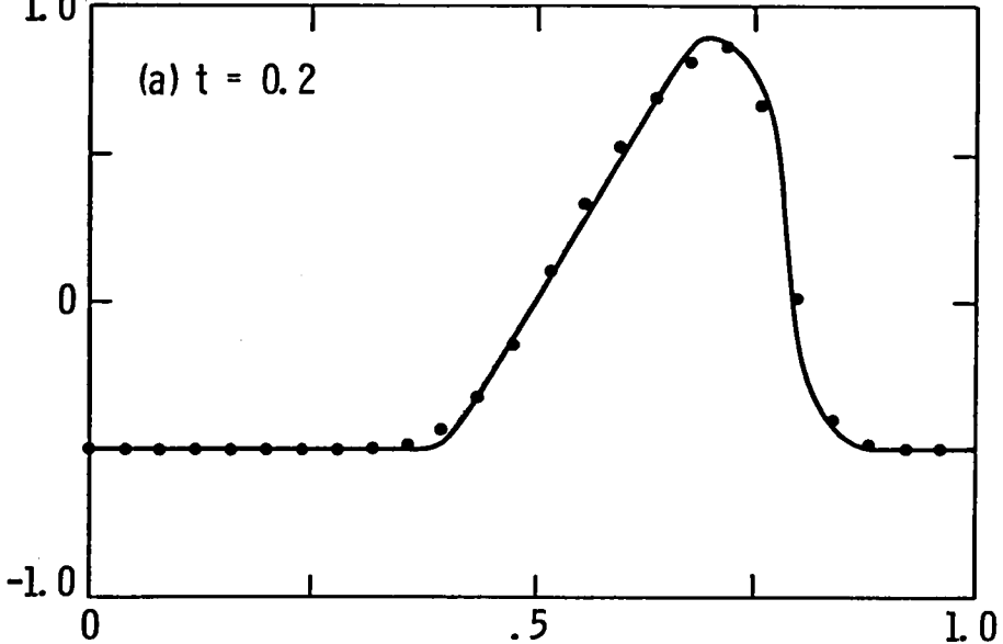
Figure 2.1 Algorithm 2.2
