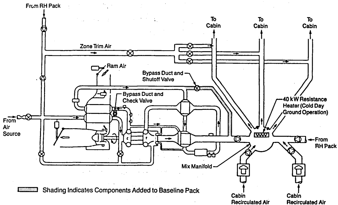
Figure 64. Air Conditioning Pack Schematic—Study Configuration 1
