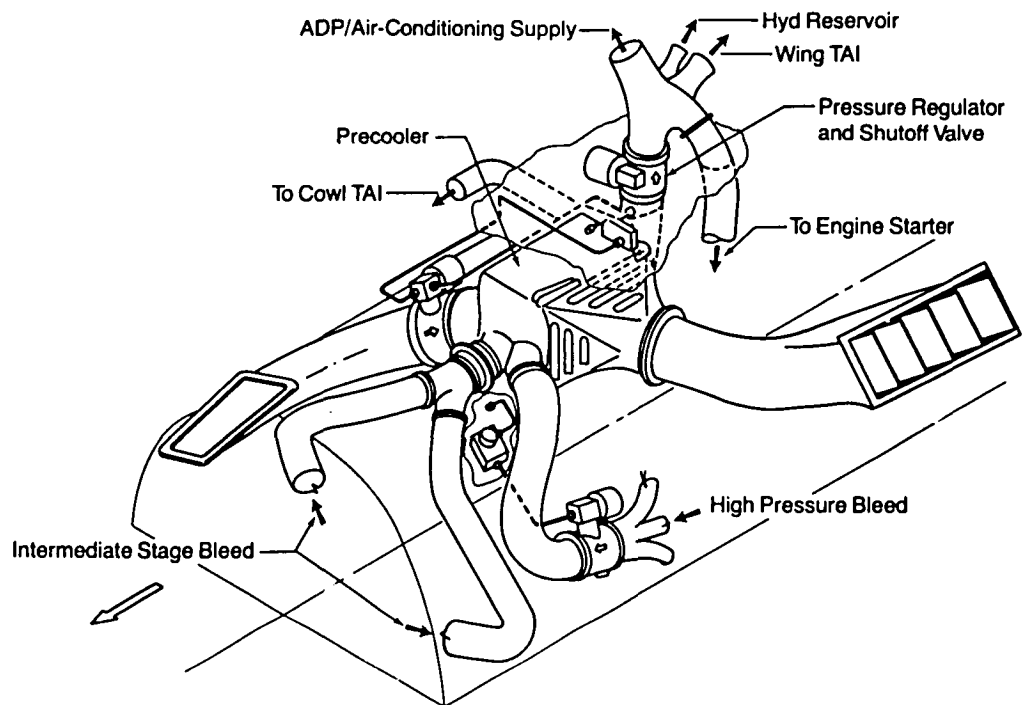
Figure 19. Engine and Strut-Mounted Air Supply Components
