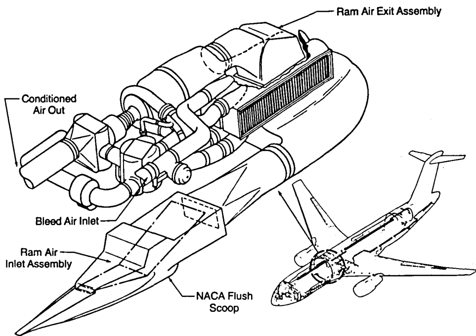
Figure 20. Baseline Air-Conditioning Packs Installation
