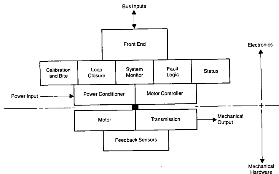
Figure 38. Smart Actuator Architecture
