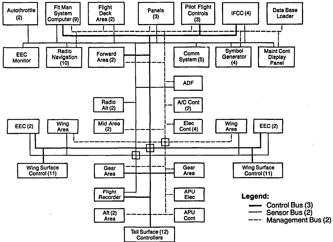
Figure 50. Data Distribution Overview
