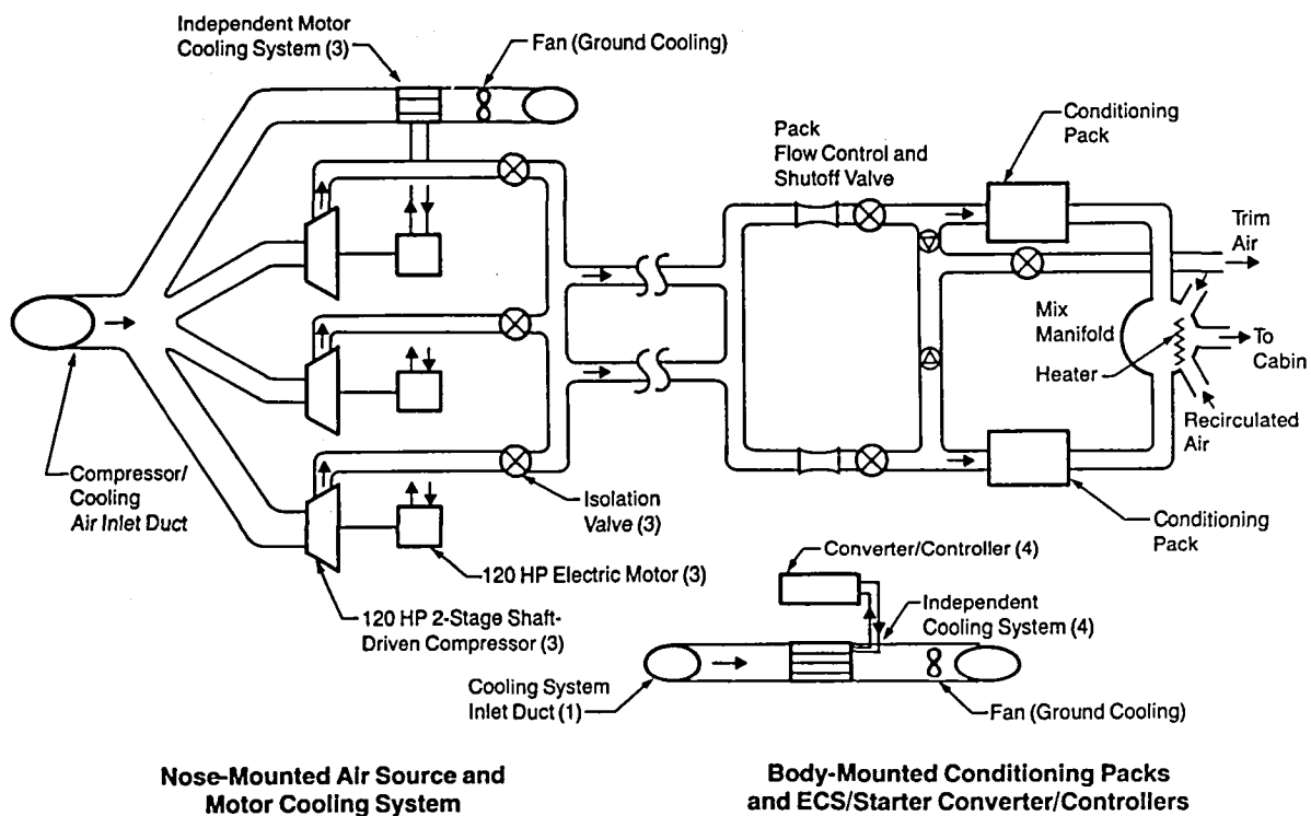
Figure 63. Selected ECS System—Study Configuration 1
