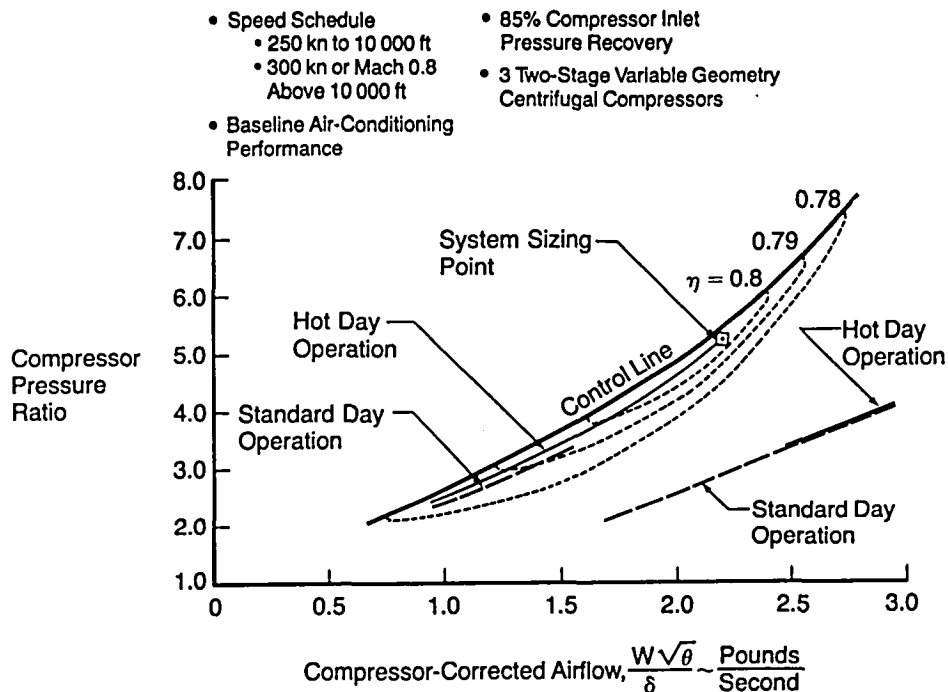
Figure 61. Representative Compressor Map—Study Configuration 1
