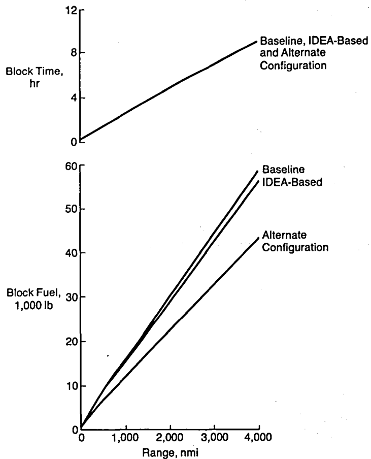
Figure 70. Block Fuel, Block Time Comparison
