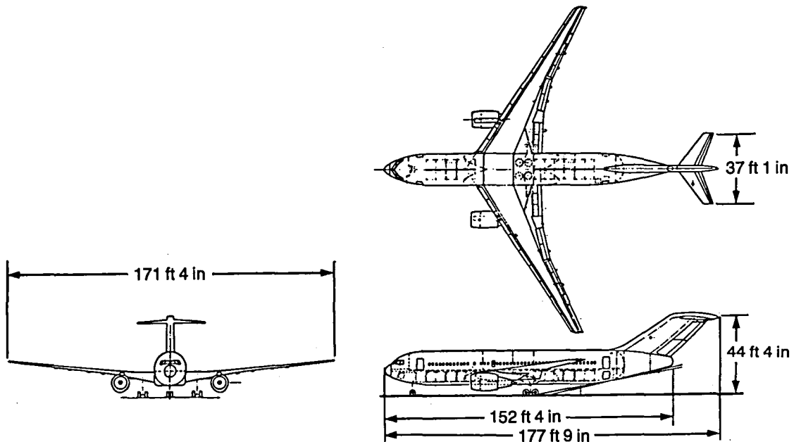
Figure 5. Final ACT Airplane
