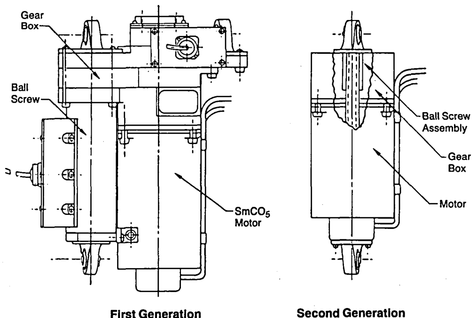
Figure 39. Electromechanical Actuator (EMA)
