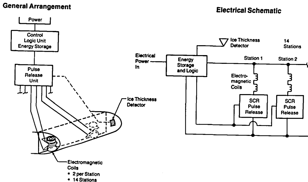
Figure 65. Electro-Impulse System
