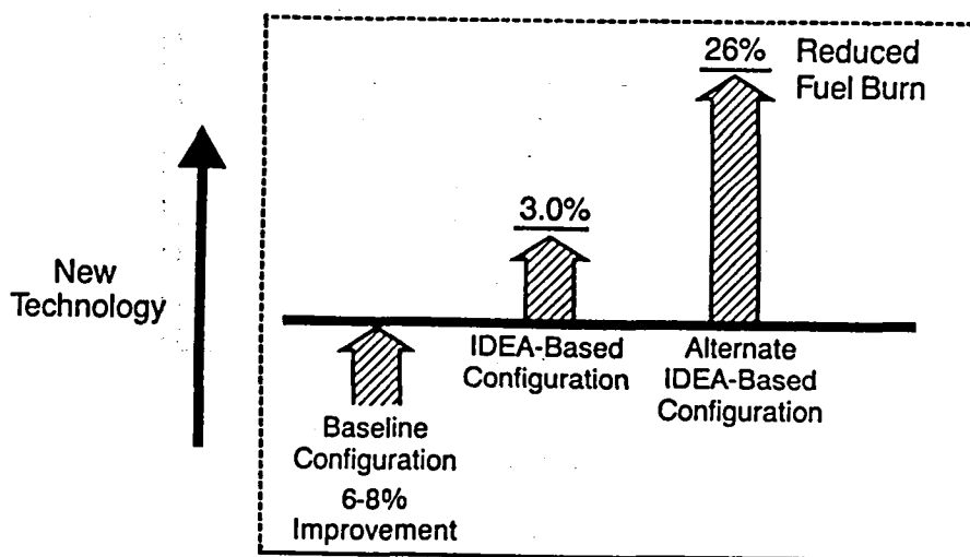
Figure 1. Fuel Burn Comparison (1000-nmi Segment)
