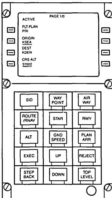
Figure 56. CDU Multifunction Keyboard
