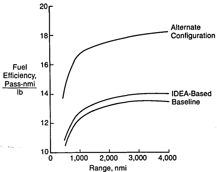
Figure 71. Fuel Efficiency Comparison
