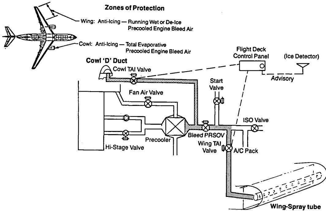
Figure 22. Baseline Airplane Ice Protection System
