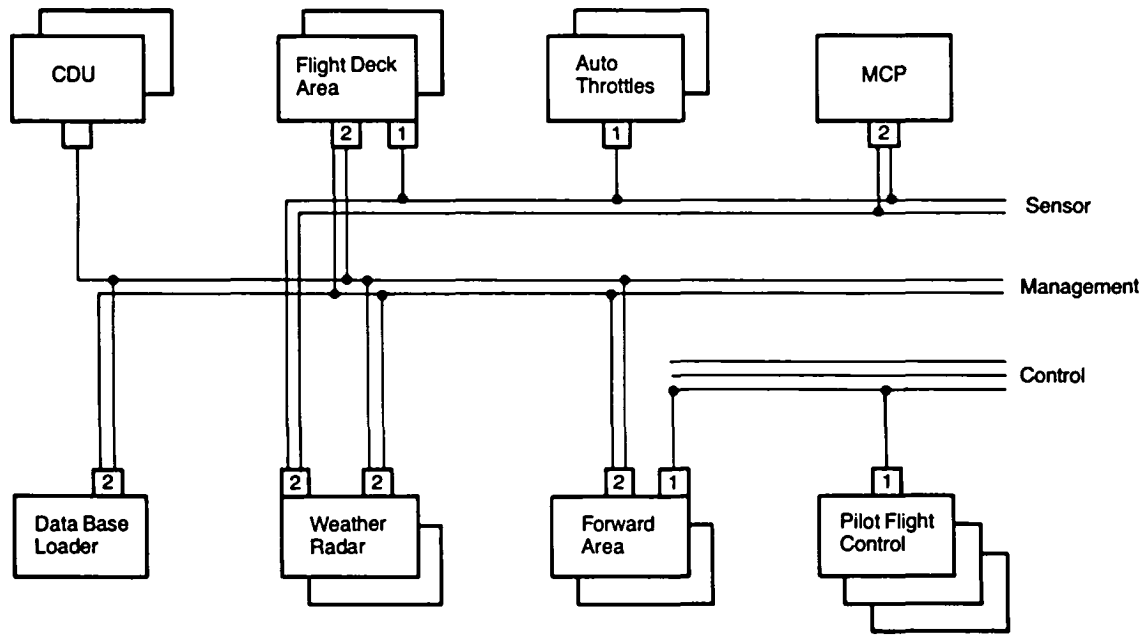
Figure 52. Flight Deck and Forward Area Detail
