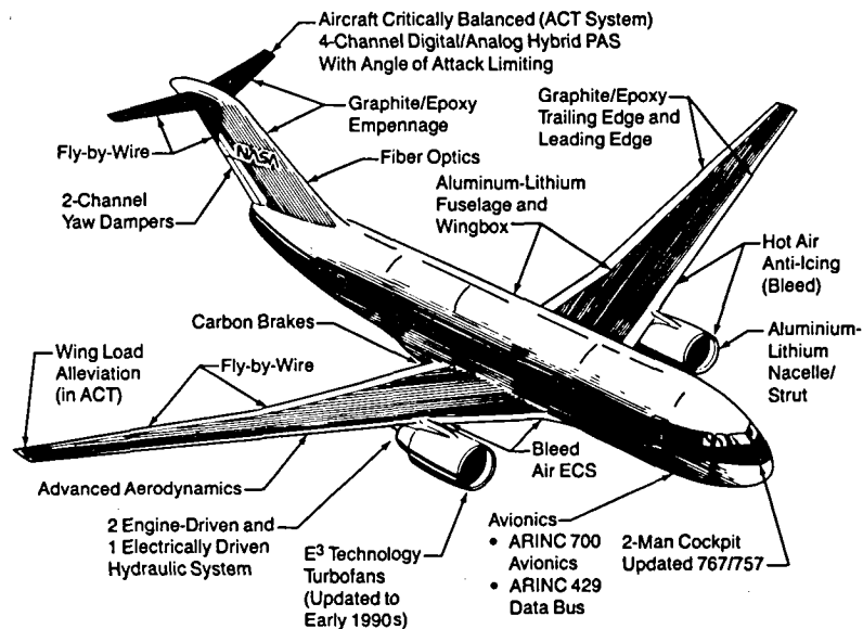
Figure 6. Baseline Configuration Summary
