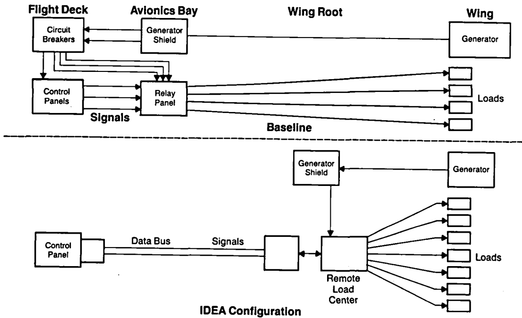
Figure 48. Power Switching and Circuit Protection Location
