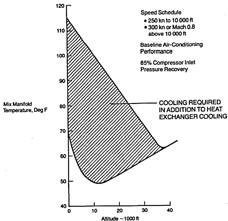
Figure 60. ECS Cabin Cooling Requirements—Hot Day
