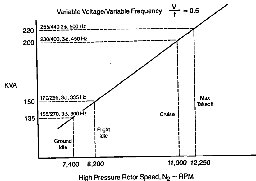
Figure 44. Generator Capacity
