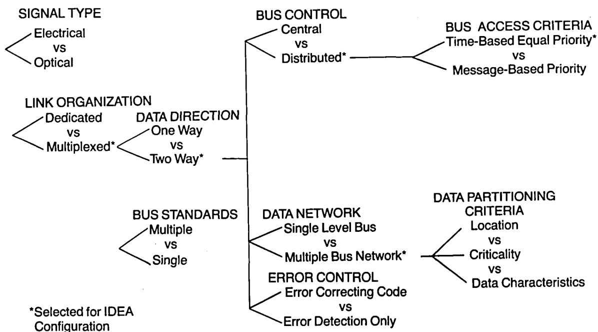
Figure 46. Data Distribution Options
