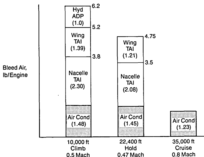
Figure 21. Baseline Required Bleed Airflow—Normal Operation
