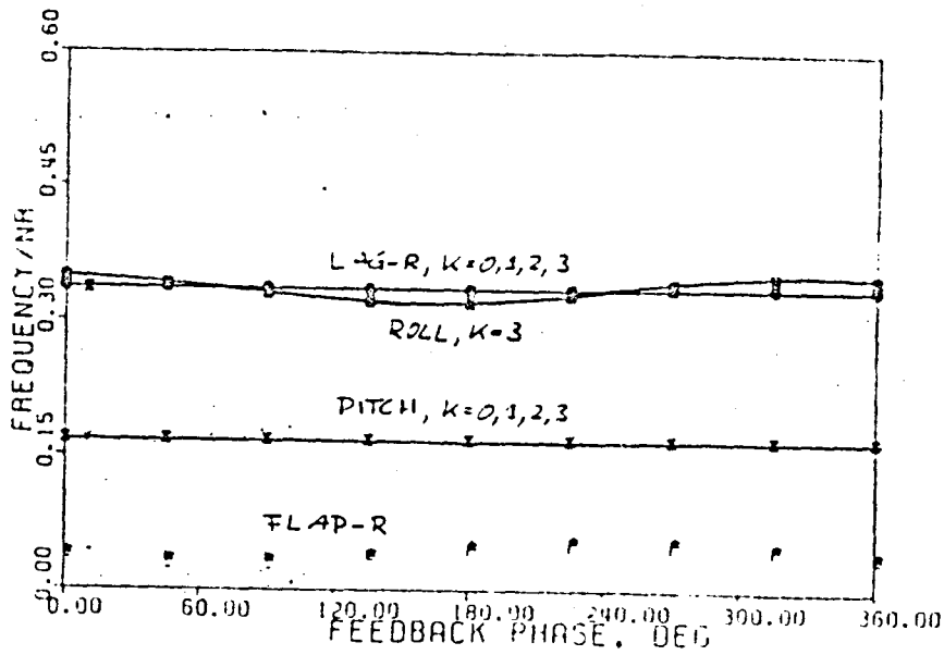
FIGURE 23. Modal Damping and Frequencies Versus Feedback Phase with Roll Acceleration Feedback, Configuration C.
