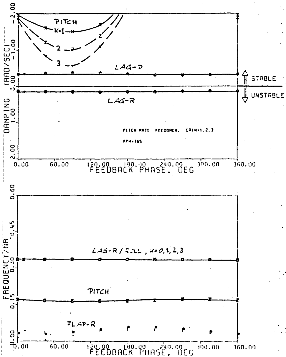
FIGURE 25. Modal Damping and Frequencies Versus Feedback Phase with Pitch Rate Feedback, Configuration C.
