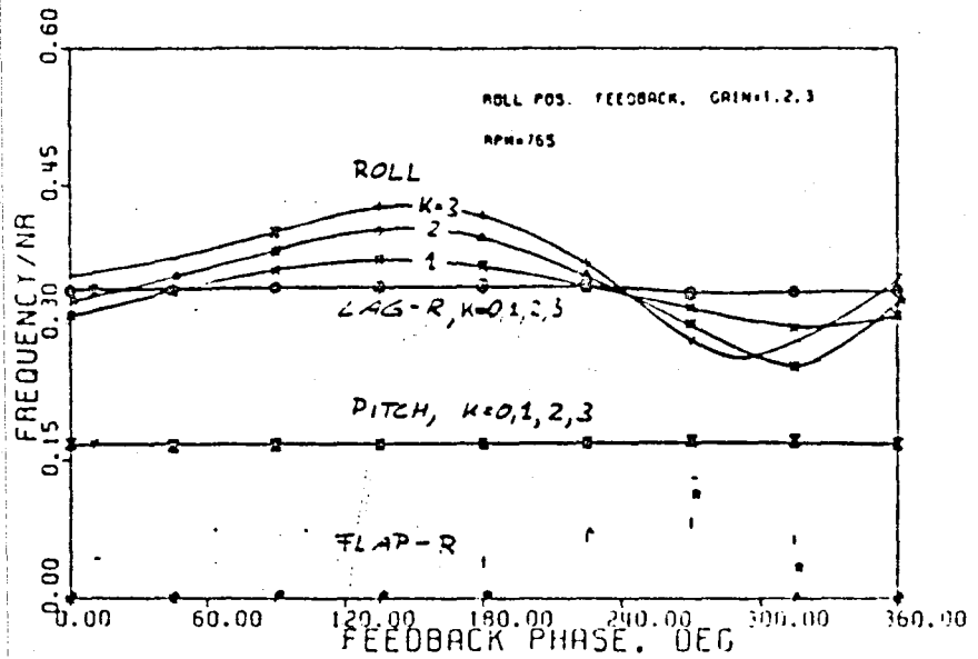
FIGURE 21. Modal Damping and Frequencies Versus Feedback Phase with Roll Feedback, Configuration C.
