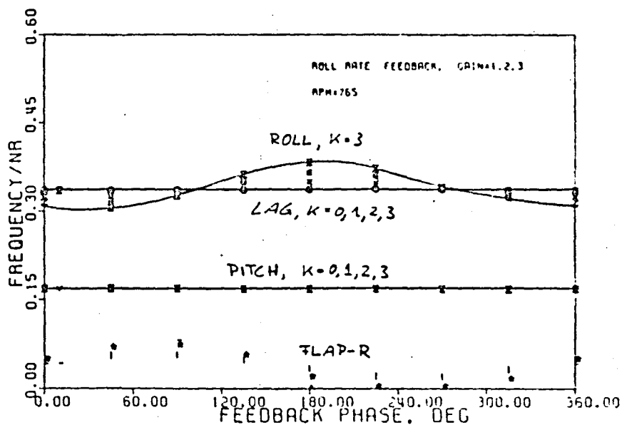
FIGURE 22. Modal Damping and Frequencies Versus Feedback Phase with Roll Rate Feedback, Configuration C.
