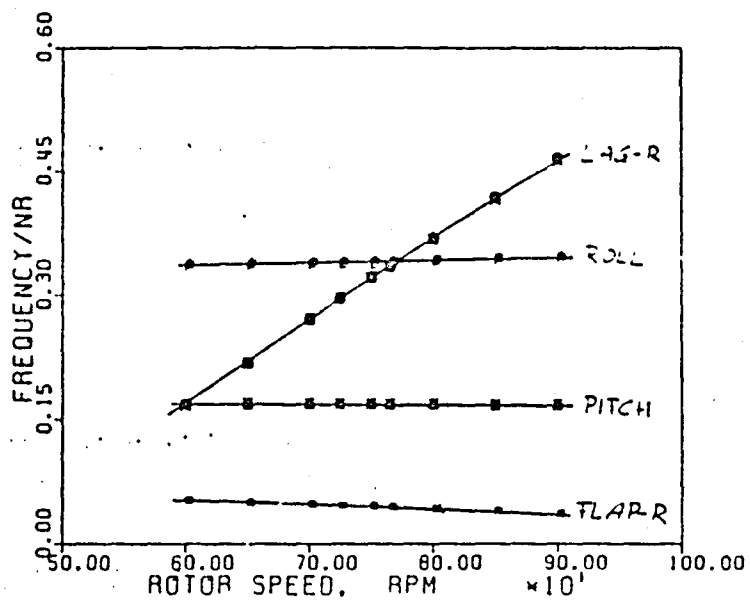
FIGURE 34. Effect of Sine Cyclic Lag Feedback Phase on Modal Damping and Frequencies, Plotted Versus Rotor Speed, Configuration C.
