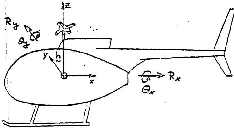
FIGURE 1. Fuselage Model
