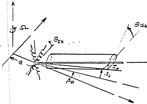
FIGURE 2. Rotor Blade Model
