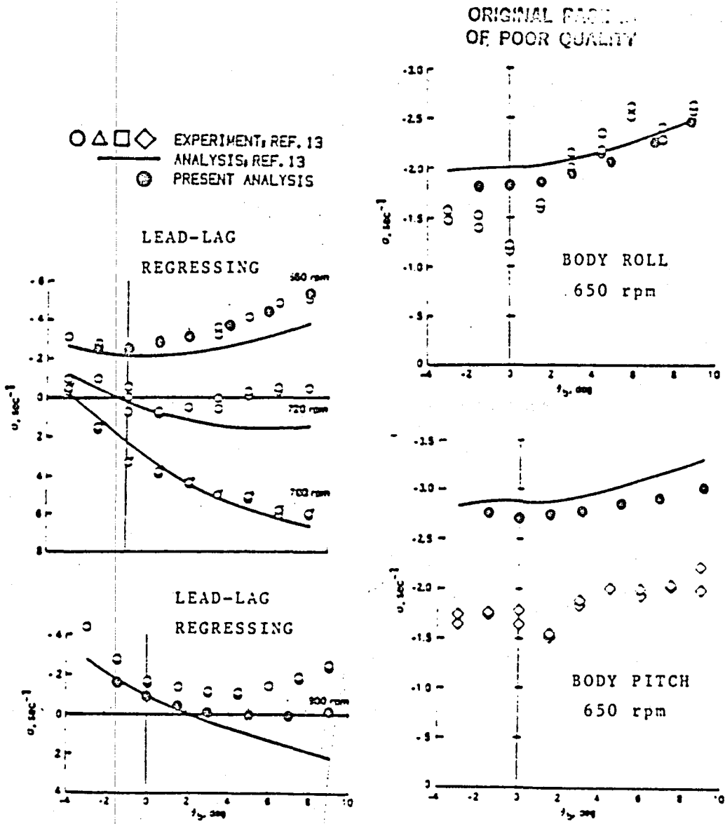
FIGURE 11. Modal Damping as a Function of Blade Pitch Angle, Configuration C.
