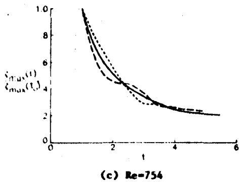
Fig. 7: Effect of Reynolds number on the decay of maximum vorticity for two vortex rings with R_0=15 and D_0=6 .
