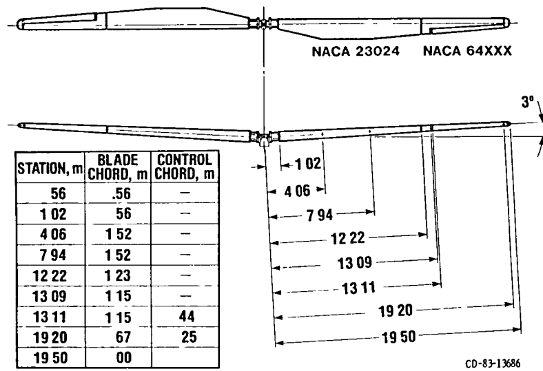
Figure 2 - Teetered, 38 percent chord aileron-control rotor.
