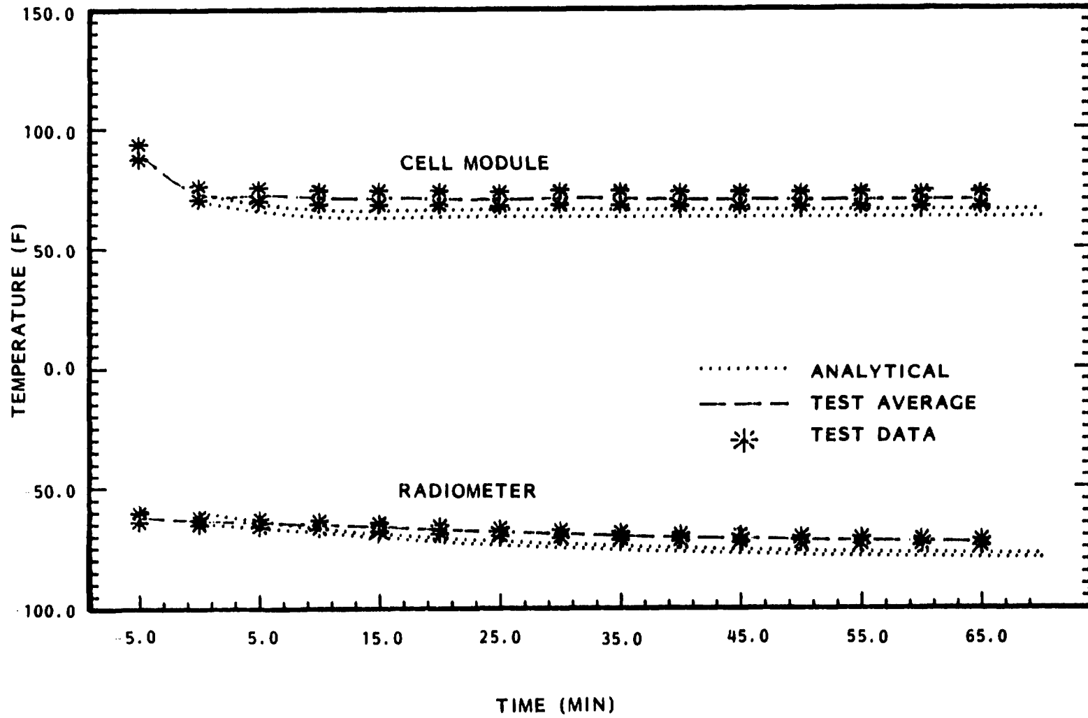
Figure 21 Module C (101.2 mW/cm 2 ) - Temperature vs Time
