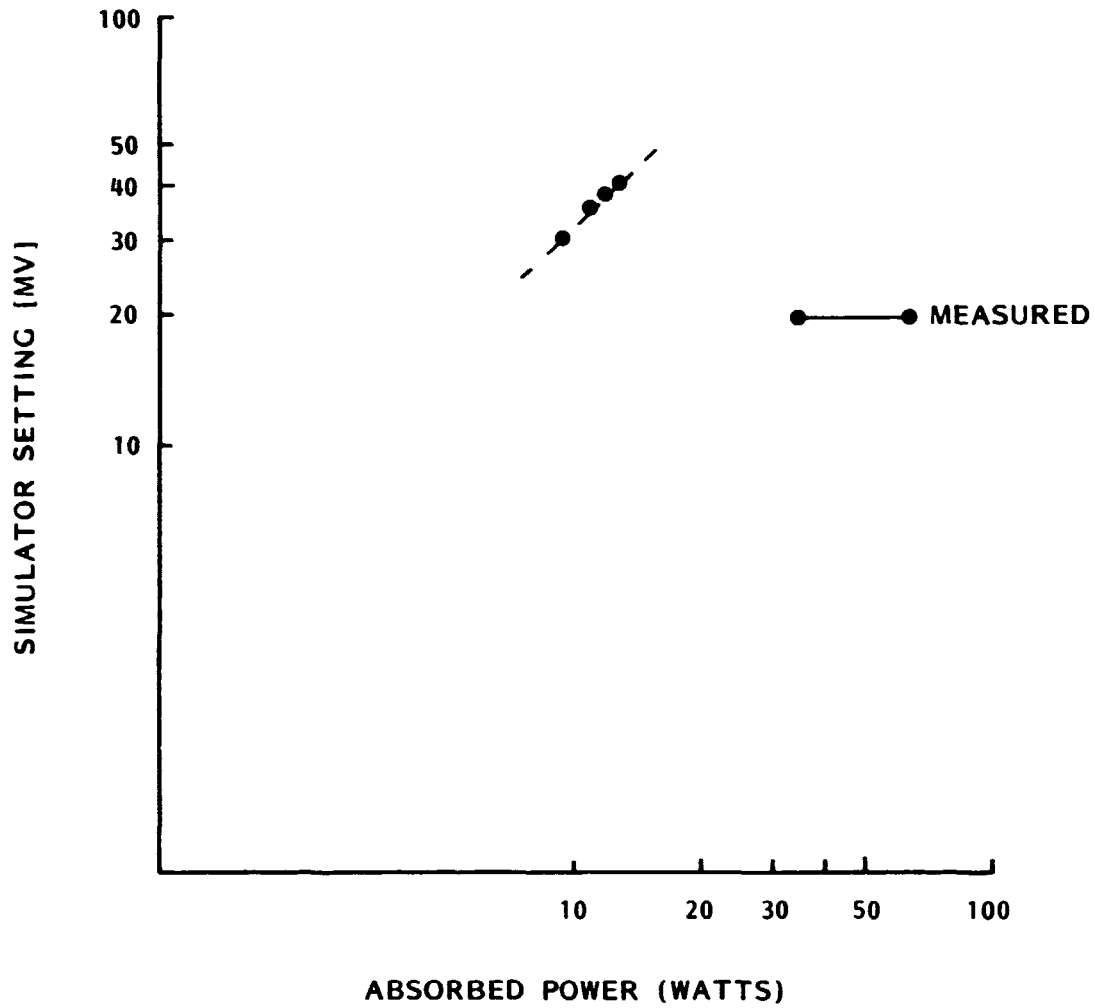
Figure 12 Simulator Setting vs Absorbed Power
