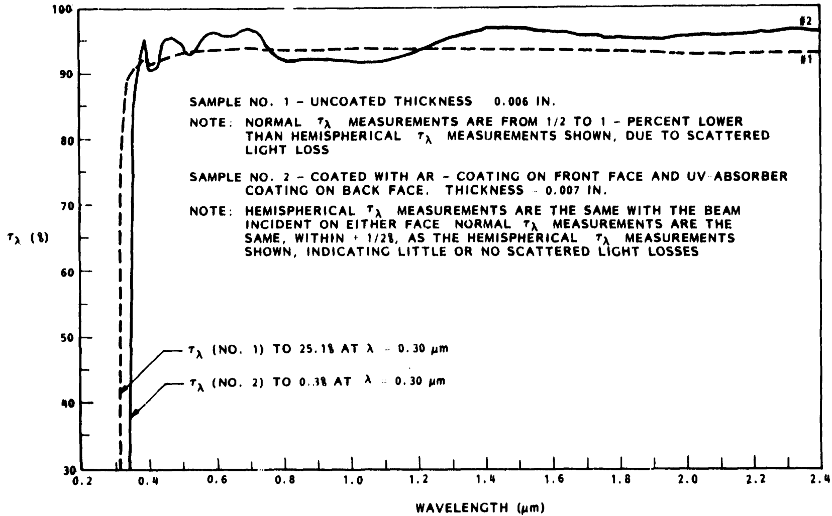
Figure 1 Spectral Transmittance Data for Coated and Uncoated Microsheet Samples
