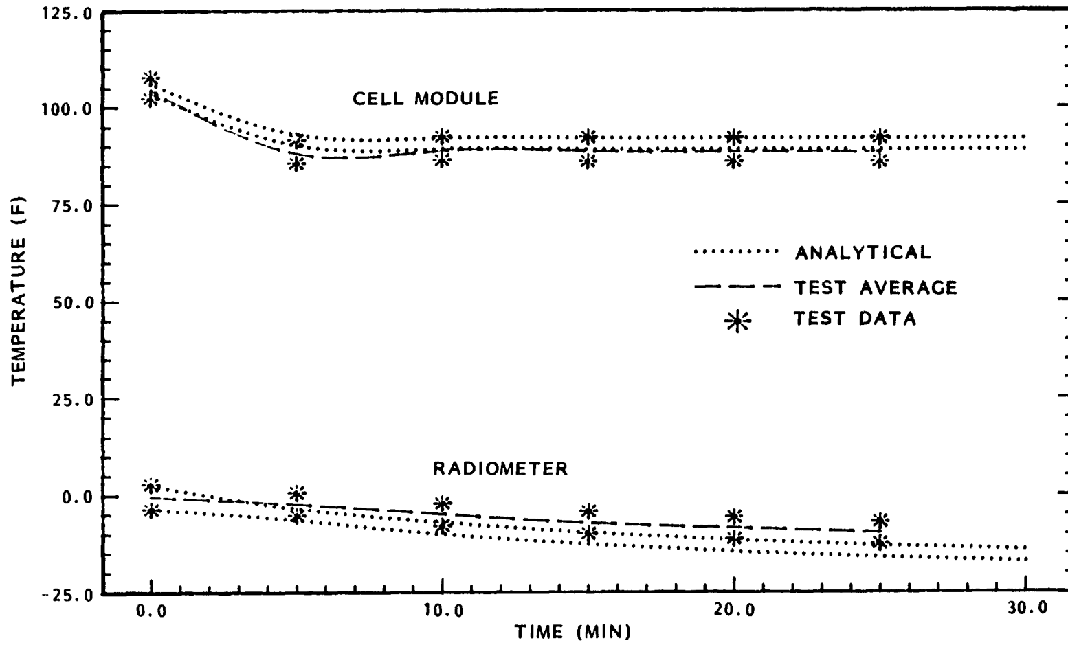
Figure 14 Module A (129.3 mW/cm 2 ) - Temperature vs Time
