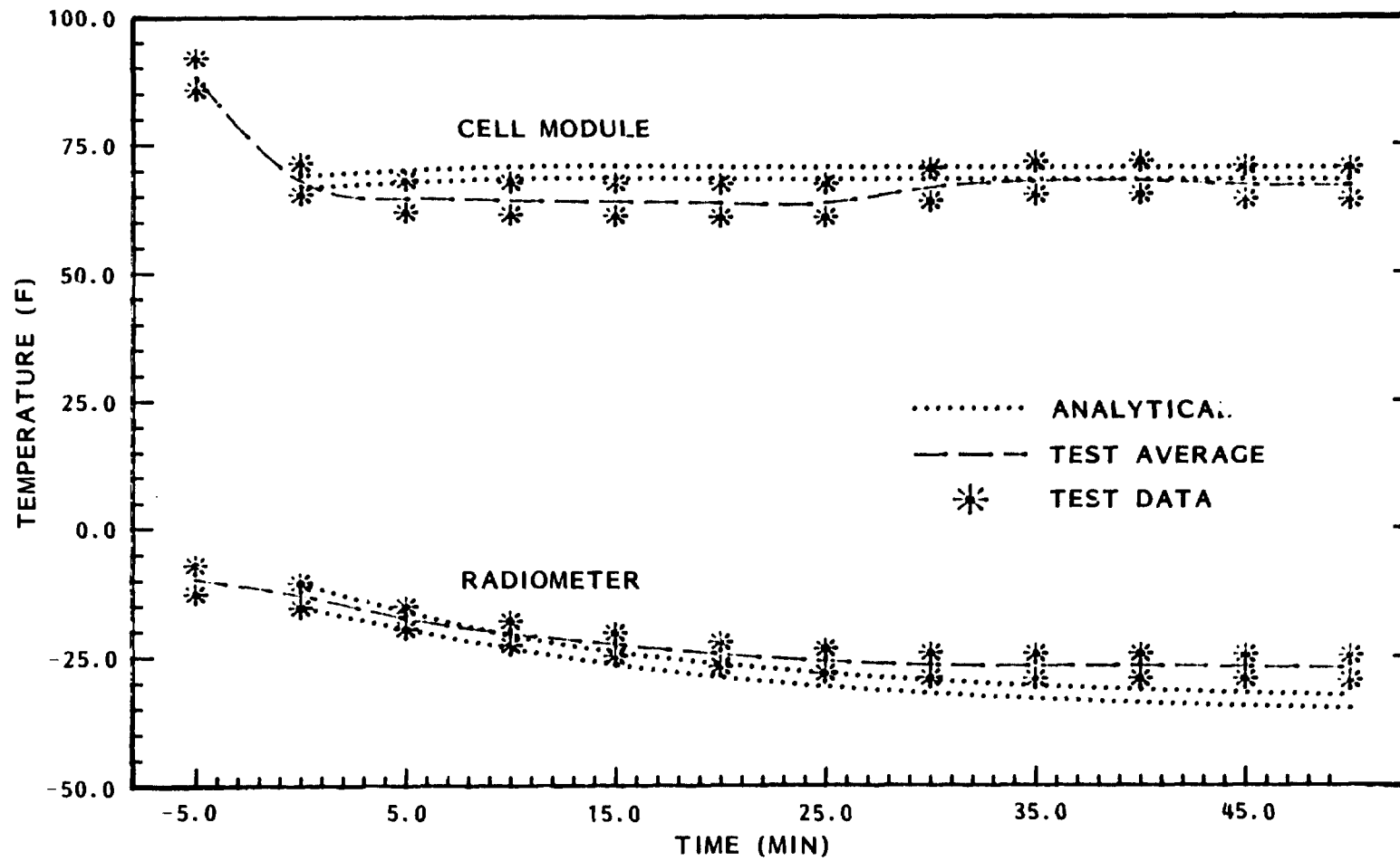
Figure 15 Module A ( 101.2 \text{ mW/cm}^2 ) - Temperature vs Time
