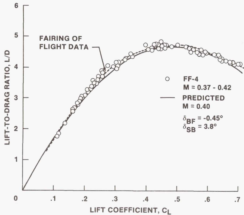
Figure 12. Tailcone-off Performance Comparisons of Flight Test and Predicted Data.
