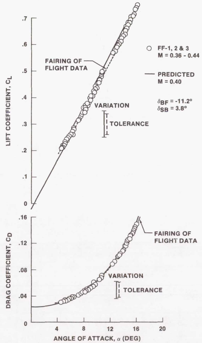
Figure 11. Tailcone-on Lift and Drag Coefficient Comparisons of Flight Test and Predicted Data.
