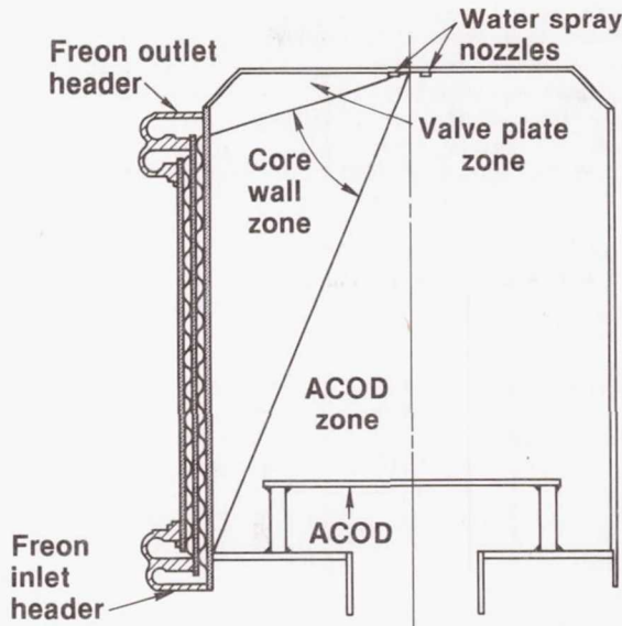
FIGURE 16 SPRAY ZONES
