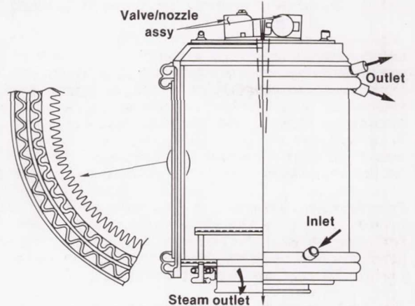
FIGURE 13 SHUTTLE EVAPORATOR
