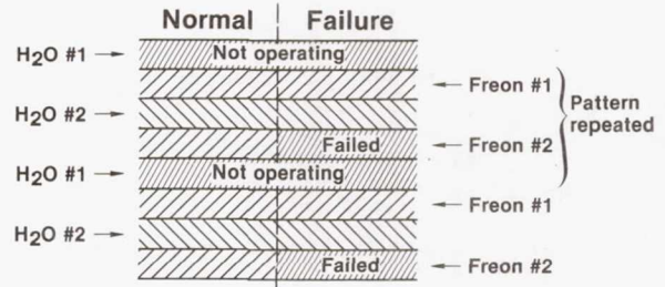
FIGURE 5 INTERCHANGER LAYERS
