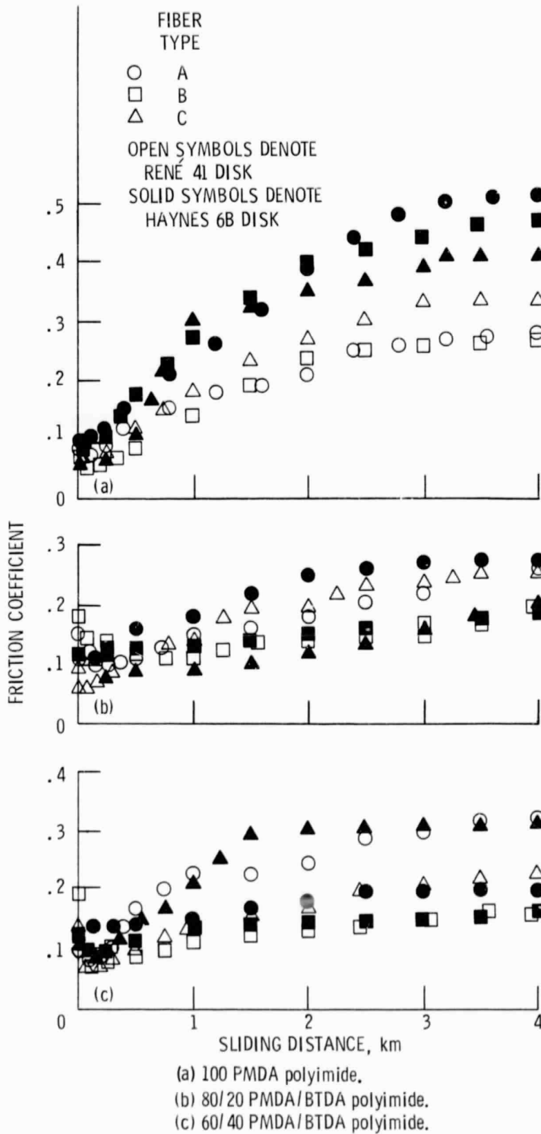
Figure 5. - Typical plots of friction coefficient as a function of sliding distance for GFRPI pins sliding against René 41 or Haynes 6B disks at 300 °C.
