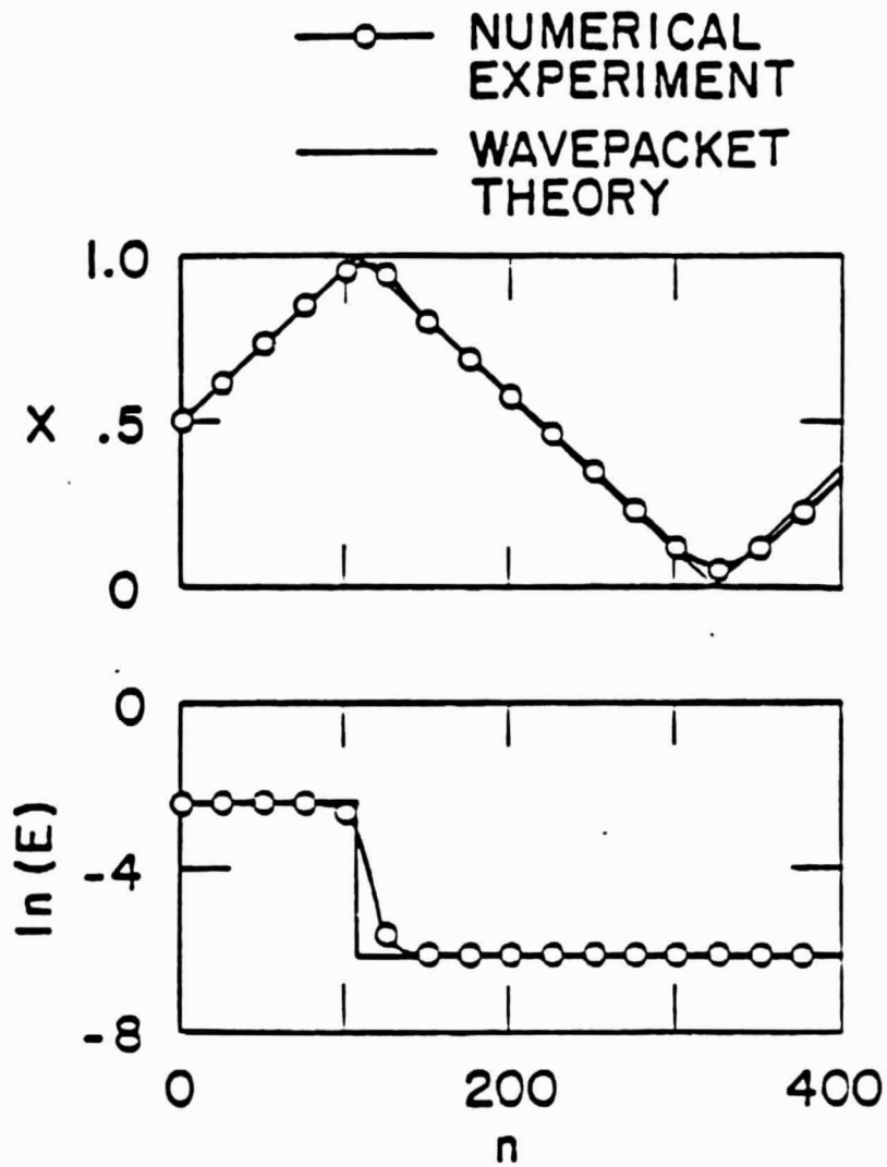
Figure 3. Position and Energy of Wavepacket: Reflections at Boundaries
