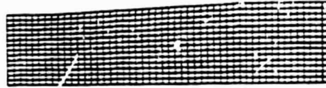
FIG. 4. Computational grid for strong shock calculations.
