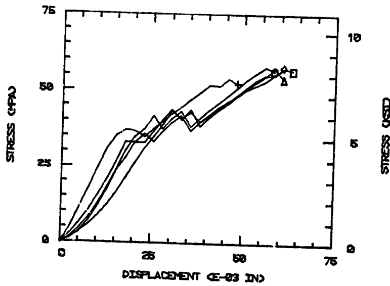
b) Stress-Displacement
