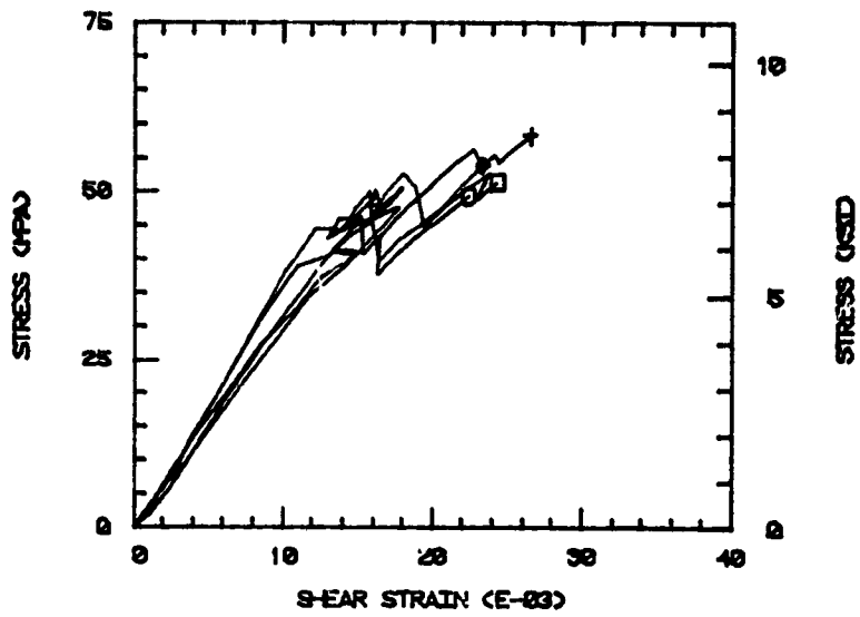
a) Stress-Strain
