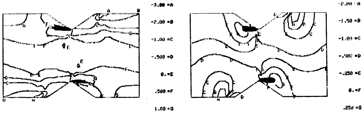
b) Normalized Transverse Normal Stress, \sigma_y/\bar{\tau}
