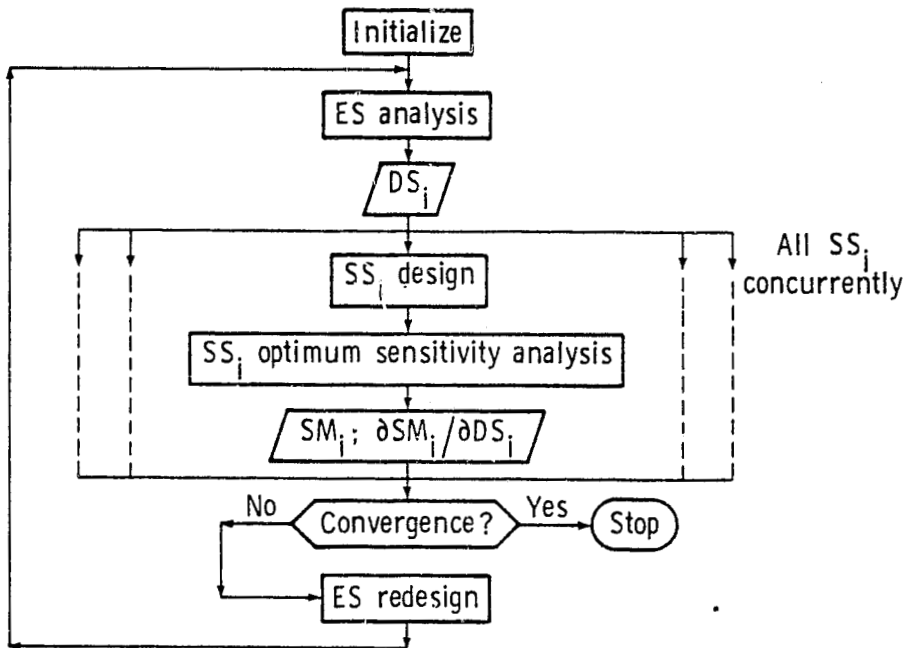
Figure 2 Two-level system optimization procedure.
