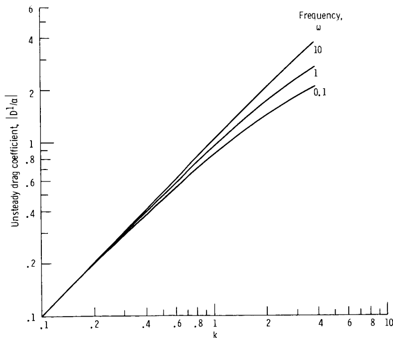
Figure 5.—Unsteady drag coefficient as function of k with frequency \omega = 0.1, 1, \text{ and } 10 .
