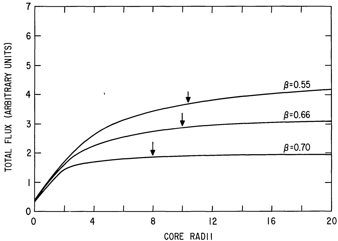
Figure 3 The total flux obtained from integrating the surface brightness profile S/S_0 = (1 + (r/a)^2)^{-3\beta+1/2} out to the specified radius (in units of core radius a ) for a value of \beta . The vertical arrows indicate the nominal cluster "edge" (90% of the total cluster flux). This determination is discussed in section IV of the text.
