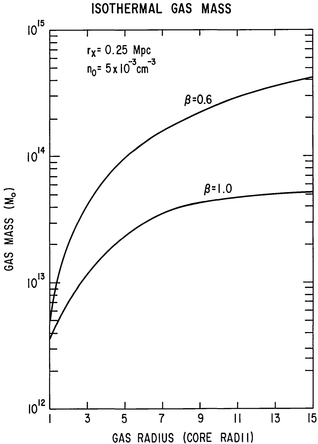
Figure 4 The mass of X-ray emitting gas is calculated under the assumption of isothermality. The total gas mass (in solar masses) within a specified number core radii is shown for the \beta = 0.6 model, and for the case of a King profile ( \beta = 1 )
