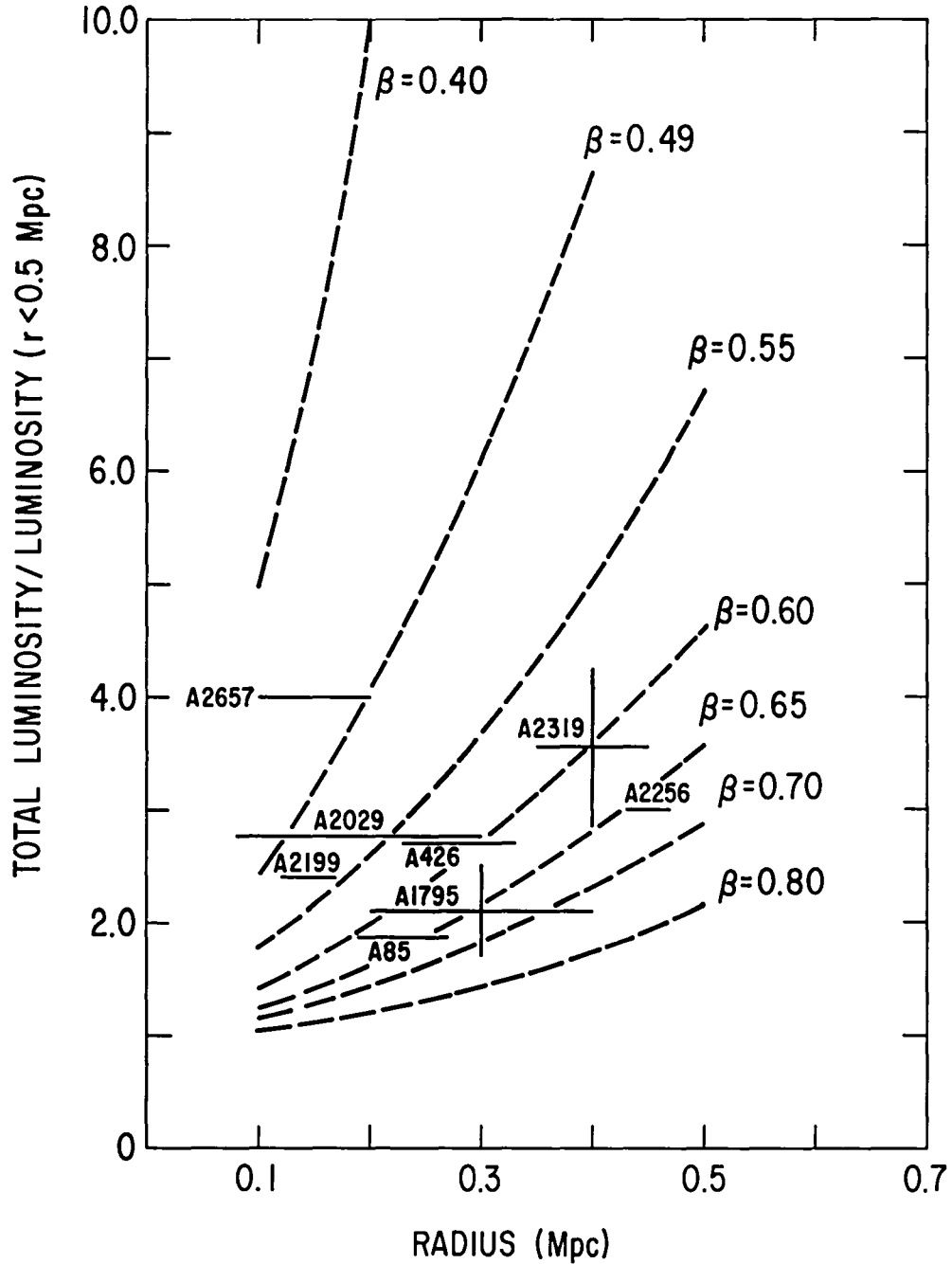
Figure 2: The parameter \beta measured using the published HEAO-1 A2 and Einstein IPC fluxes. The sample error bars combine the systematic uncertainty of the HEAO-1 A2 detector and the error in the IPC flux to give the error in the flux ratio. The IPC fluxes, core radii, and their associated errors are from Jones and Forman (1984)
