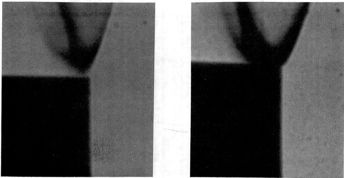
Fig.V-8a (contd.) Schlieren Pictures of Methane-Air Flame Stabilized Over Flame Holder D.
