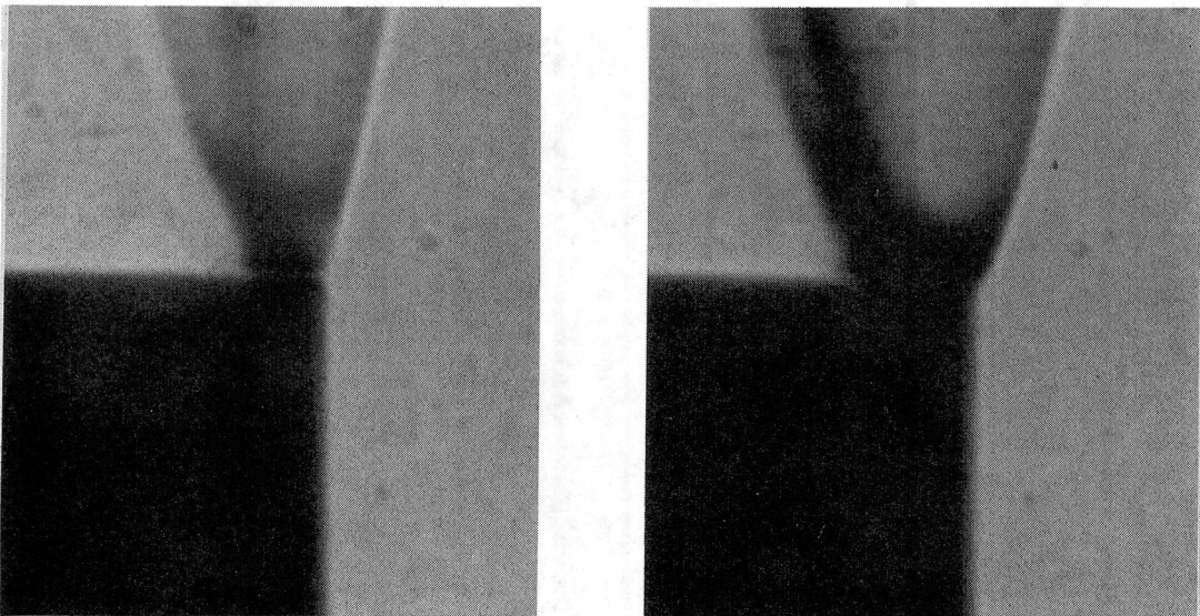
Fig.V-6 (contd.) Schlieren Pictures of Methane-Air Flame Stabilized Over Flame Holder B.
