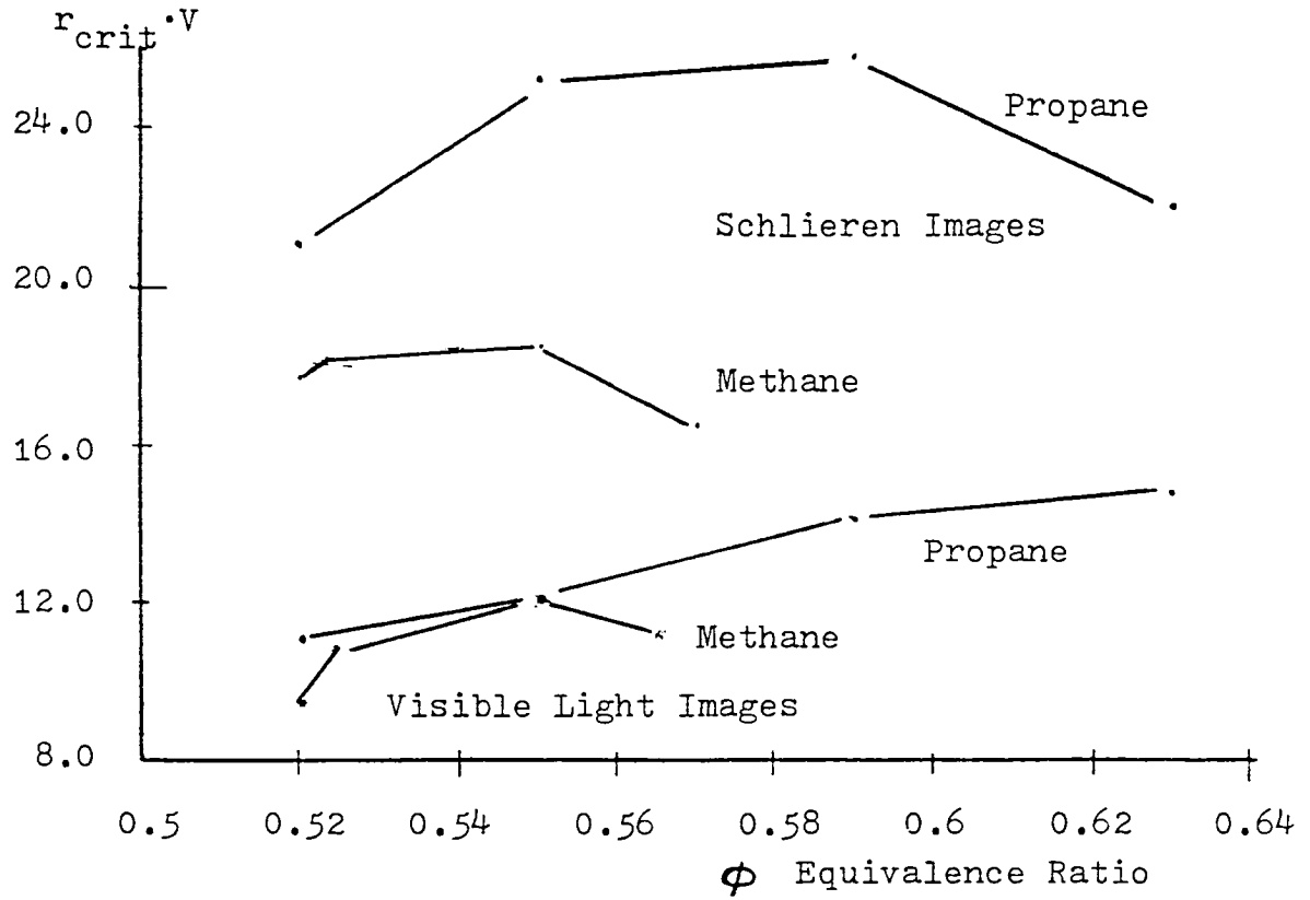
Fig.VI-4. Behavior of r_{crit} \cdot V for Flame Holder A.
