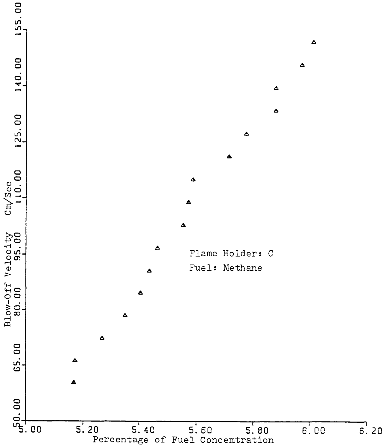
Fig.V-3. Blow-Off Velocity versus Fuel Concentration.
