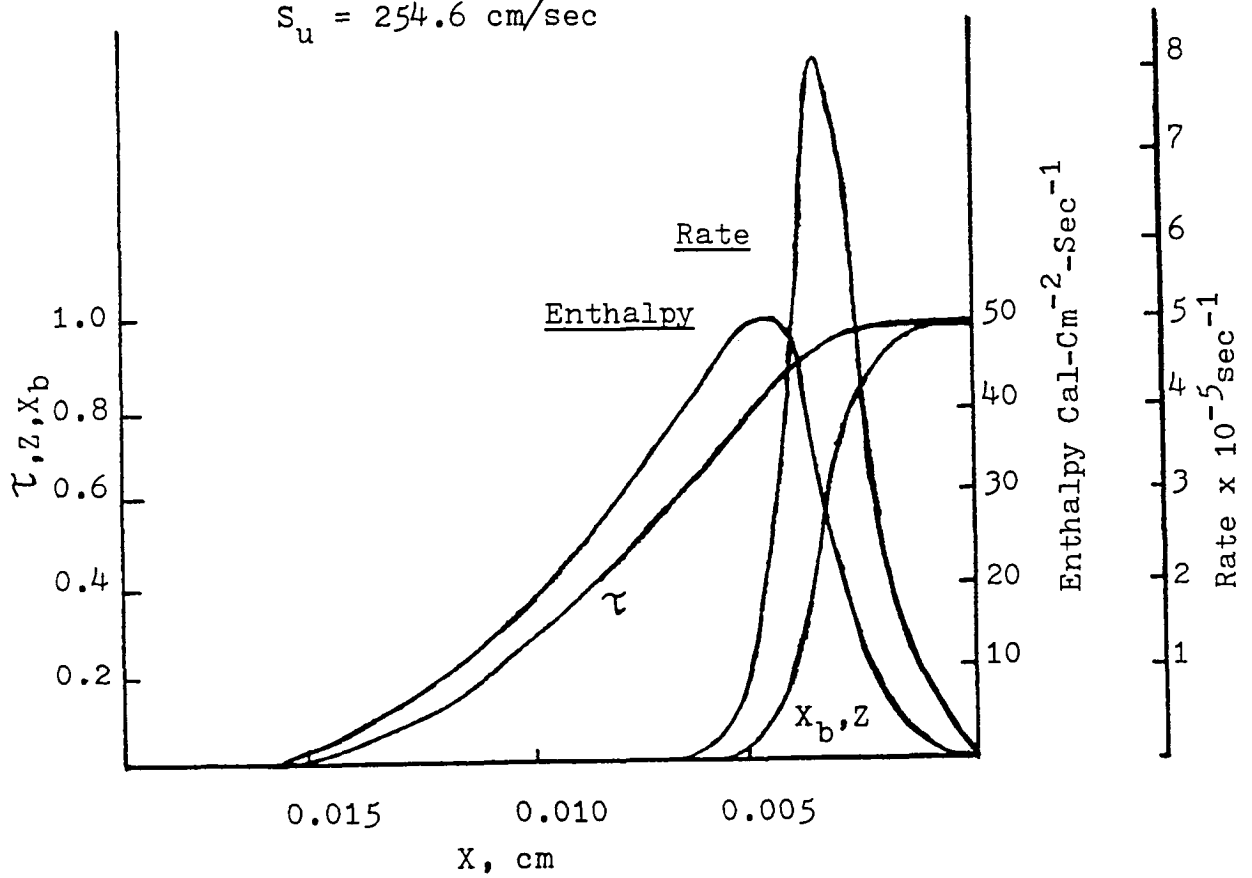
Fig. II-5b. Flame Structure for a flame with Lewis Number = 0.0 (13).
