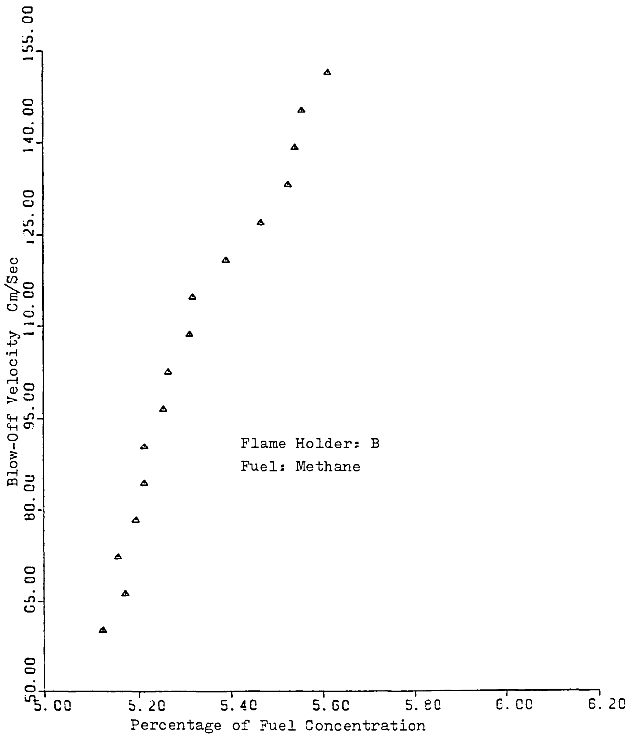
Fig.V-2. Blow-Off Velocity versus Fuel Concentration.
