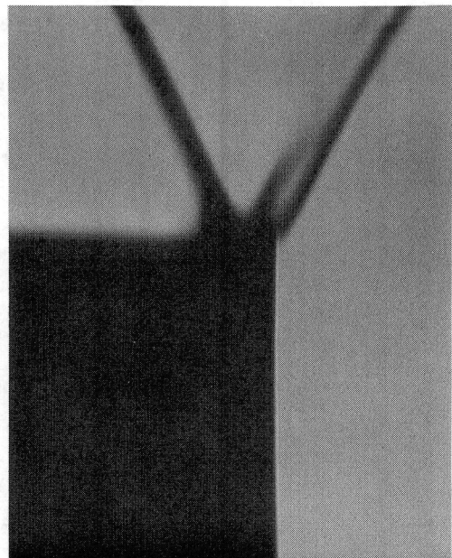
Fig.V-8b (contd.) Schlieren Pictures of Propane-Air Flame Stabilized Over Flame Holder D.
