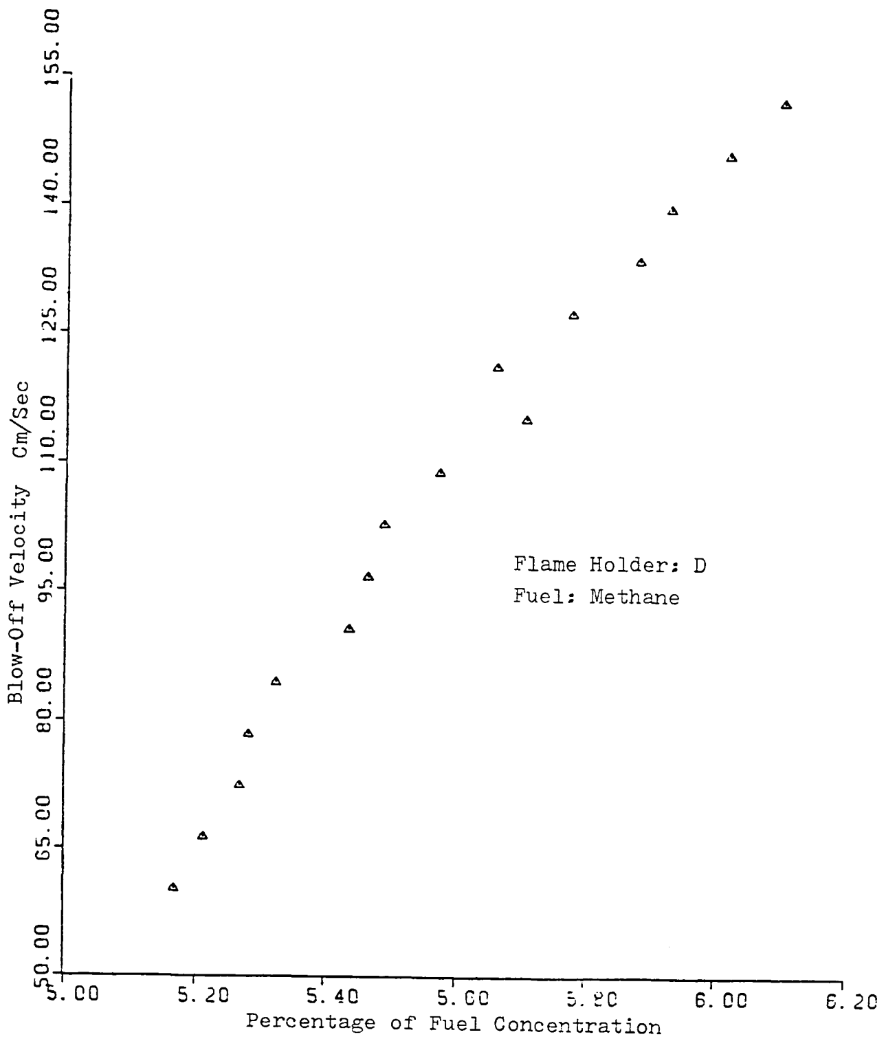
Fig.V-4a. Blow-Off Velocity versus Fuel Concentration.
