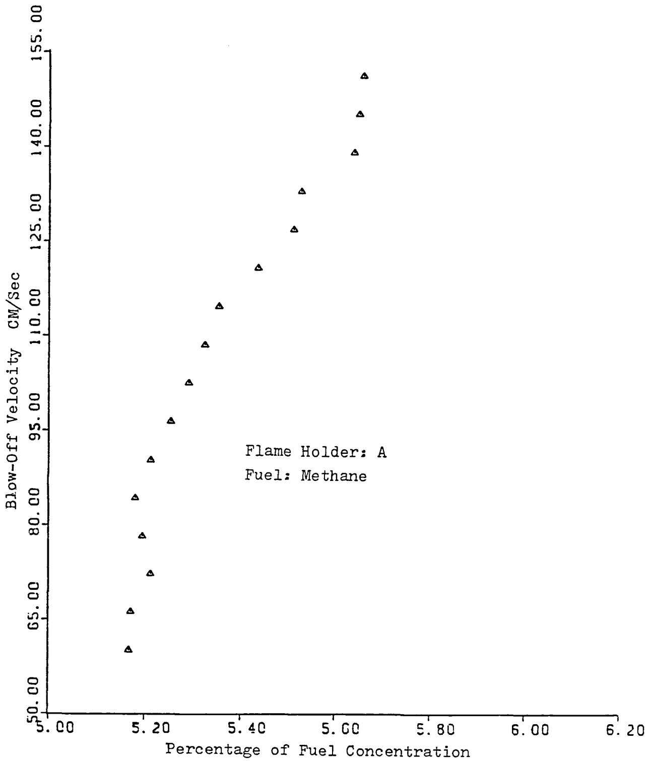
Fig.V-1a. Blow-Off Velocity versus Fuel Concentration.
