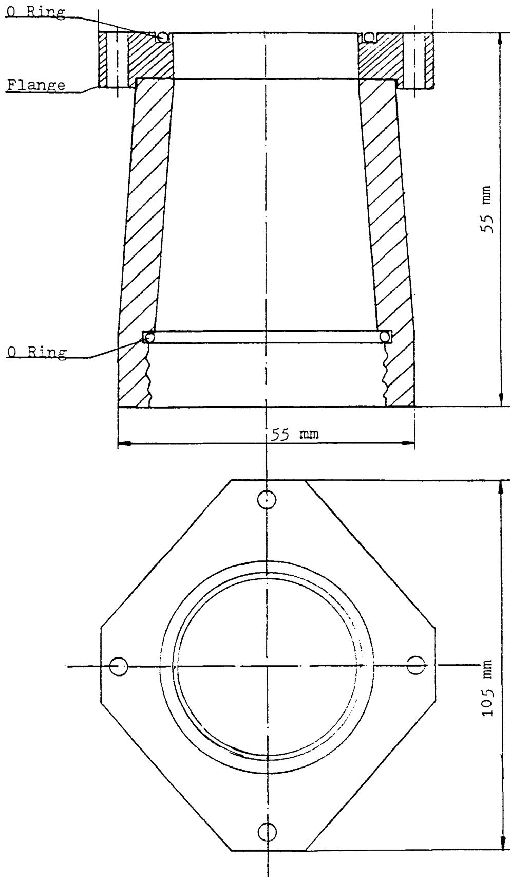
Fig. IV-3. Back Diffuser
