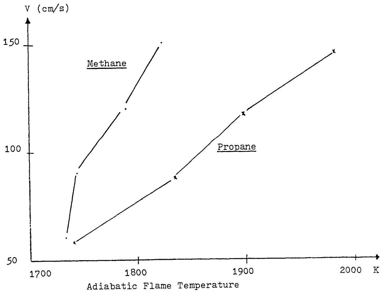
Fig.VI-6. Blow-Off Velocity vs Adiabatic Flame Temp.
