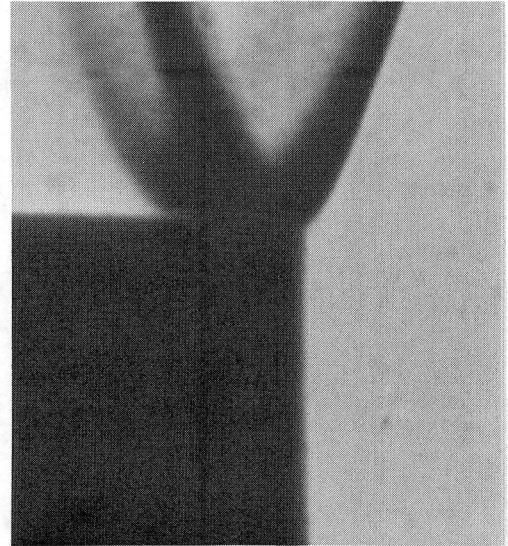
Fig.V-7 (contd.) Schlieren Pictures of Methane-Air Flame Stabilized Over Flame Holder C.
