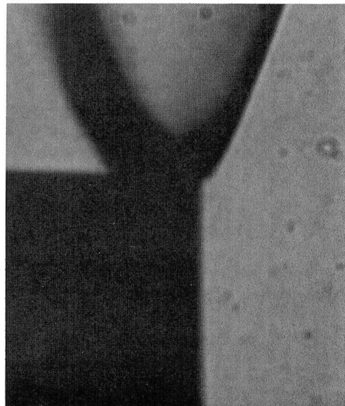
Fig.V-6. Schlieren Pictures of Methane-Air Flame Stabilized over Flame Holder B.
