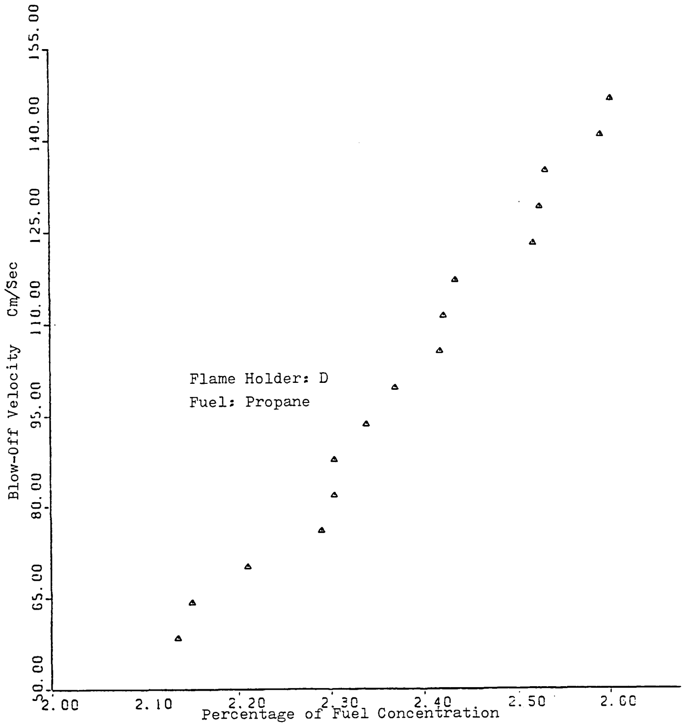
Fig.V-4b. Blow-Off Velocity versus Fuel Concentration
