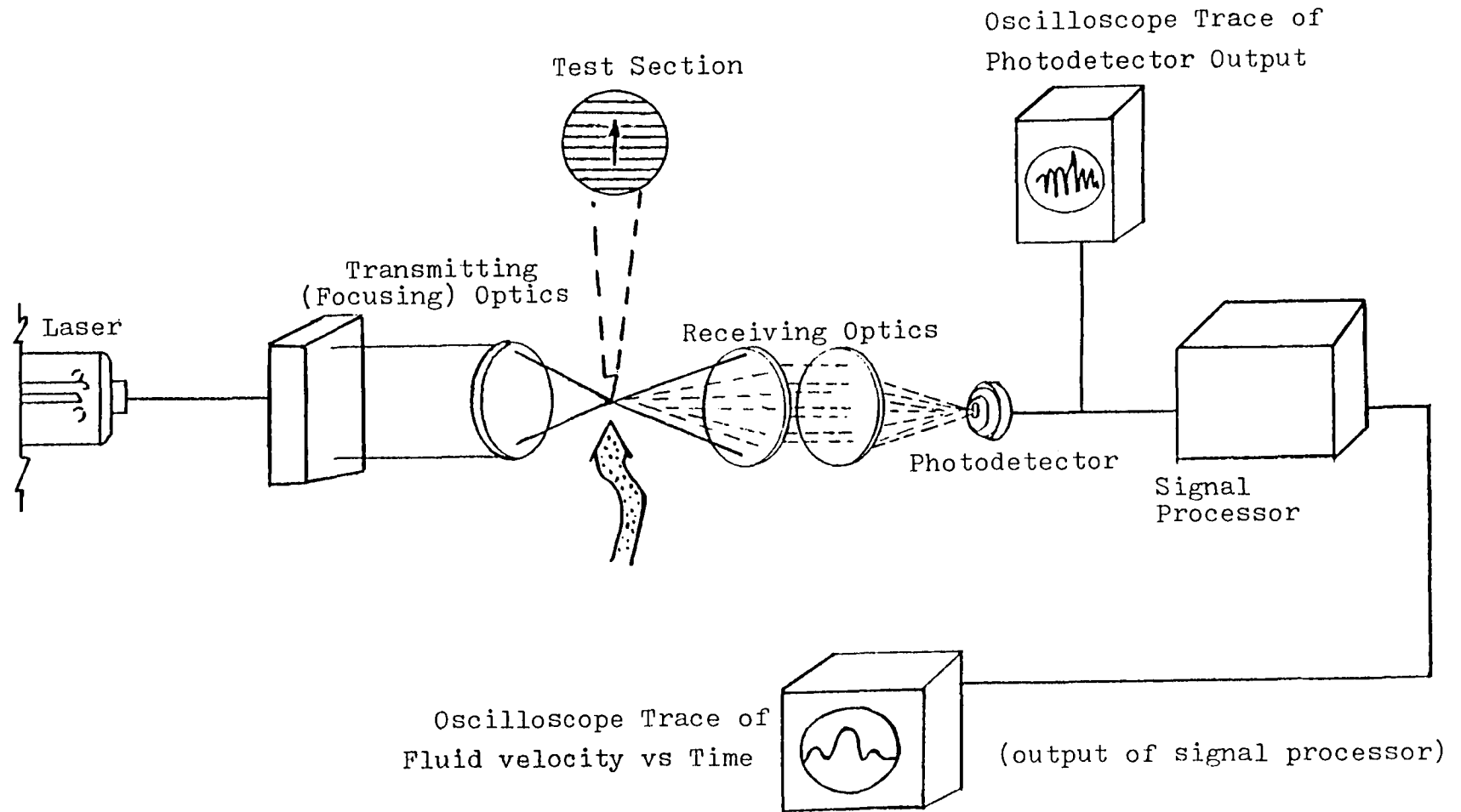
Fig. IV-11. Complete Dual Beam LDV System.
