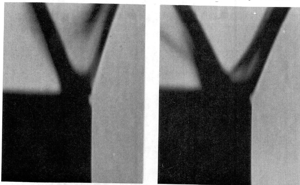
Fig.V-5b (contd.) Schlieren Pictures for Propane-Air Flame Stabilized Over Flame Holder A
