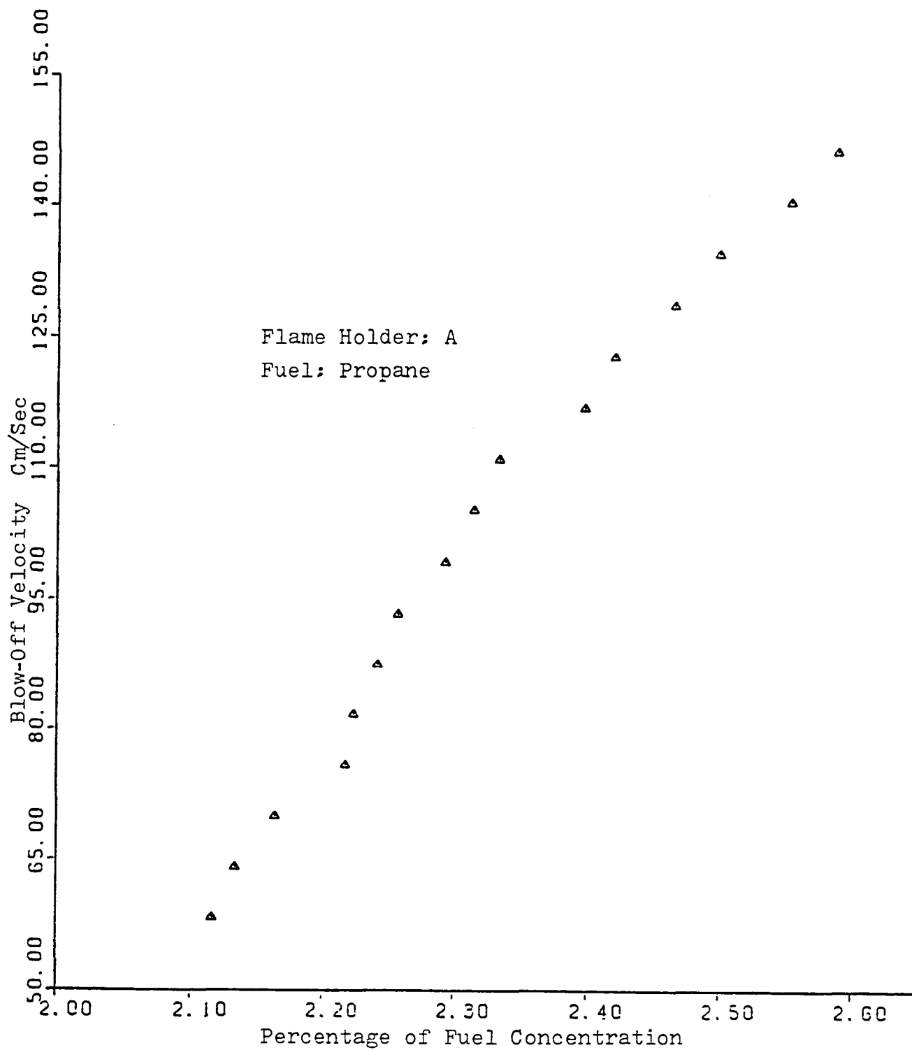
Fig.V-1b. Blow-Off Velocity versus Fuel Concentration.
