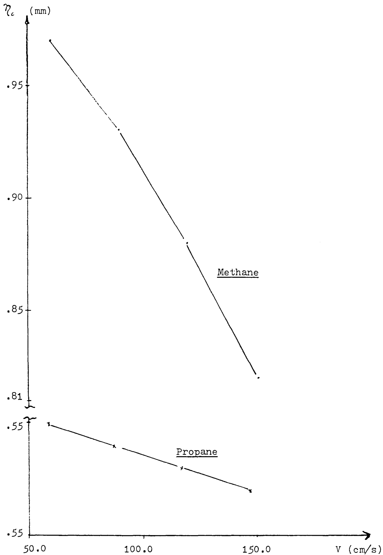
Fig.VI-5. \eta_c versus Blow-Off Velocity for Flame Holder A.
