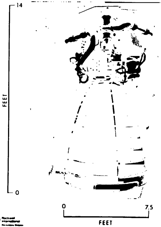
Figure 1. - Space shuttle main engine, main design specifications.
