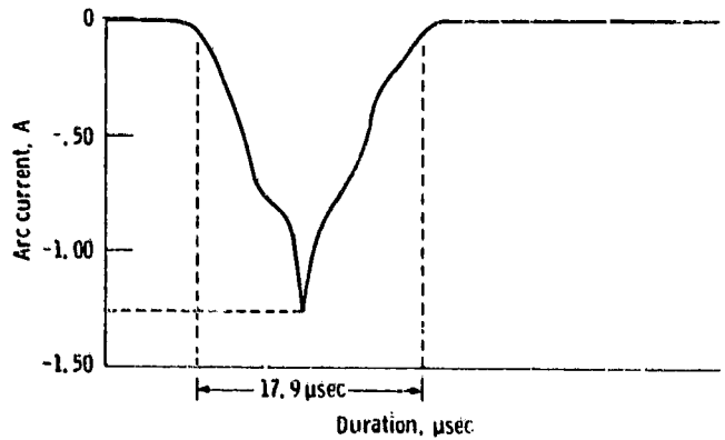
(c) Tungsten pin/disk with Kapton tape. Applied voltage, -800 V, capacitance, 0.01 \mu F.
