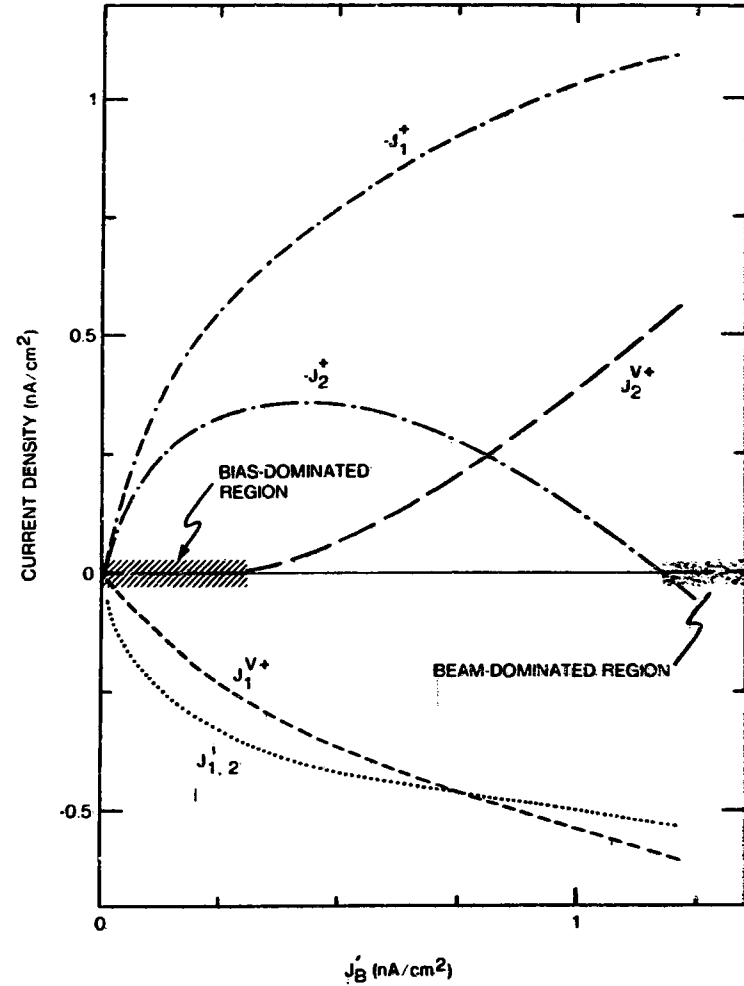
Figure 8. Collected Currents J_{1,2}^+ vs Electron Beam Current J_B' Modelled With a Positive Applied Bias, Assuming Constant G and H
