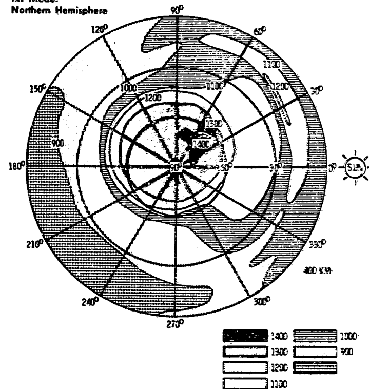
(b) Oxygen ion temperature at 400 km.
