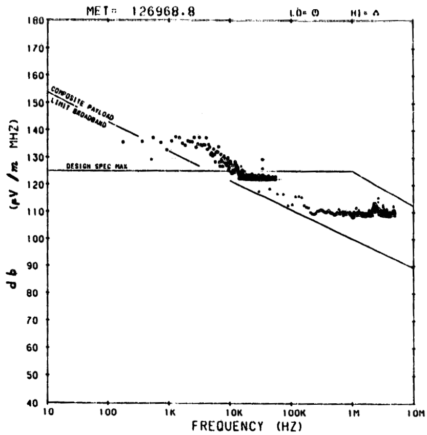
Figure 5. - Typical power spectrum of electrostatic noise.
