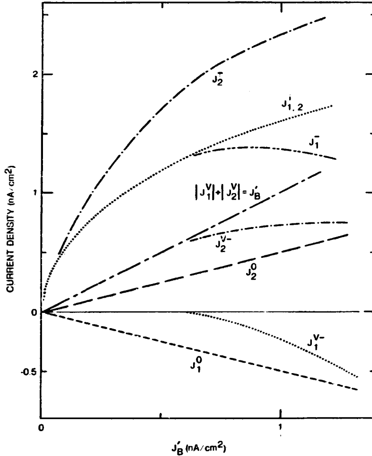
Figure 7. Collected Currents J_{1,2}^- vs Electron Beam Current J_B' Modelled With a Negative Applied Bias, Assuming Constant G and H (constituent parts result from injection at contacts J_{1,2}^i and from motion of beam-deposited charge J_{1,2}^{V-} )
