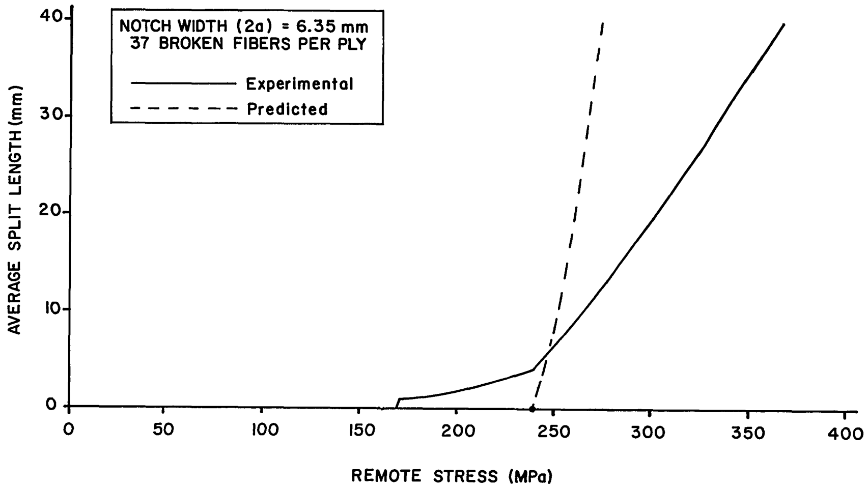
Figure 35. Average split length versus remote stress for 37 broken fibers: comparison of experimental and predicted behavior.
