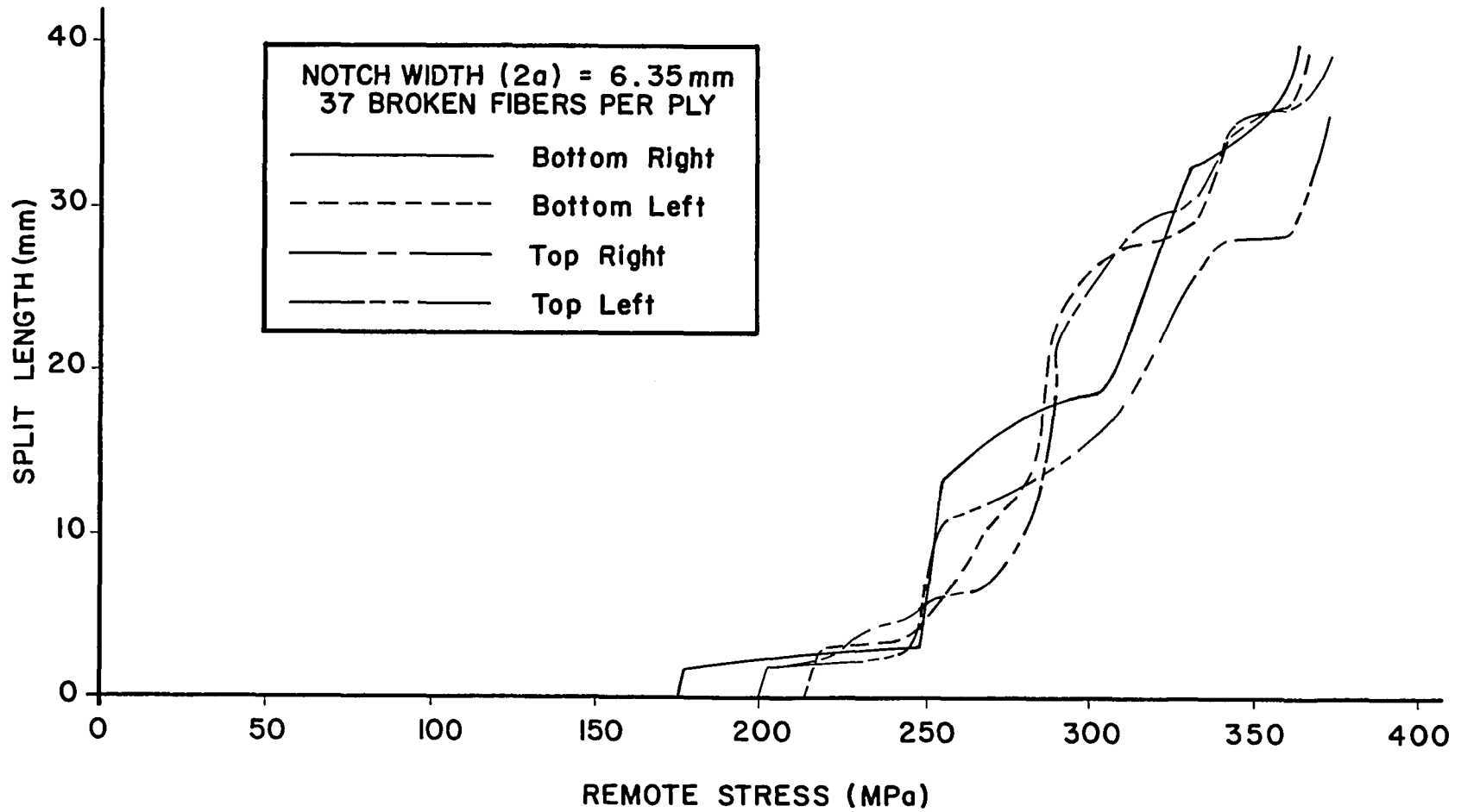
Figure 31. Experimental average split length versus remote stress showing the variation of growth rates among the splits of a single coupon.
