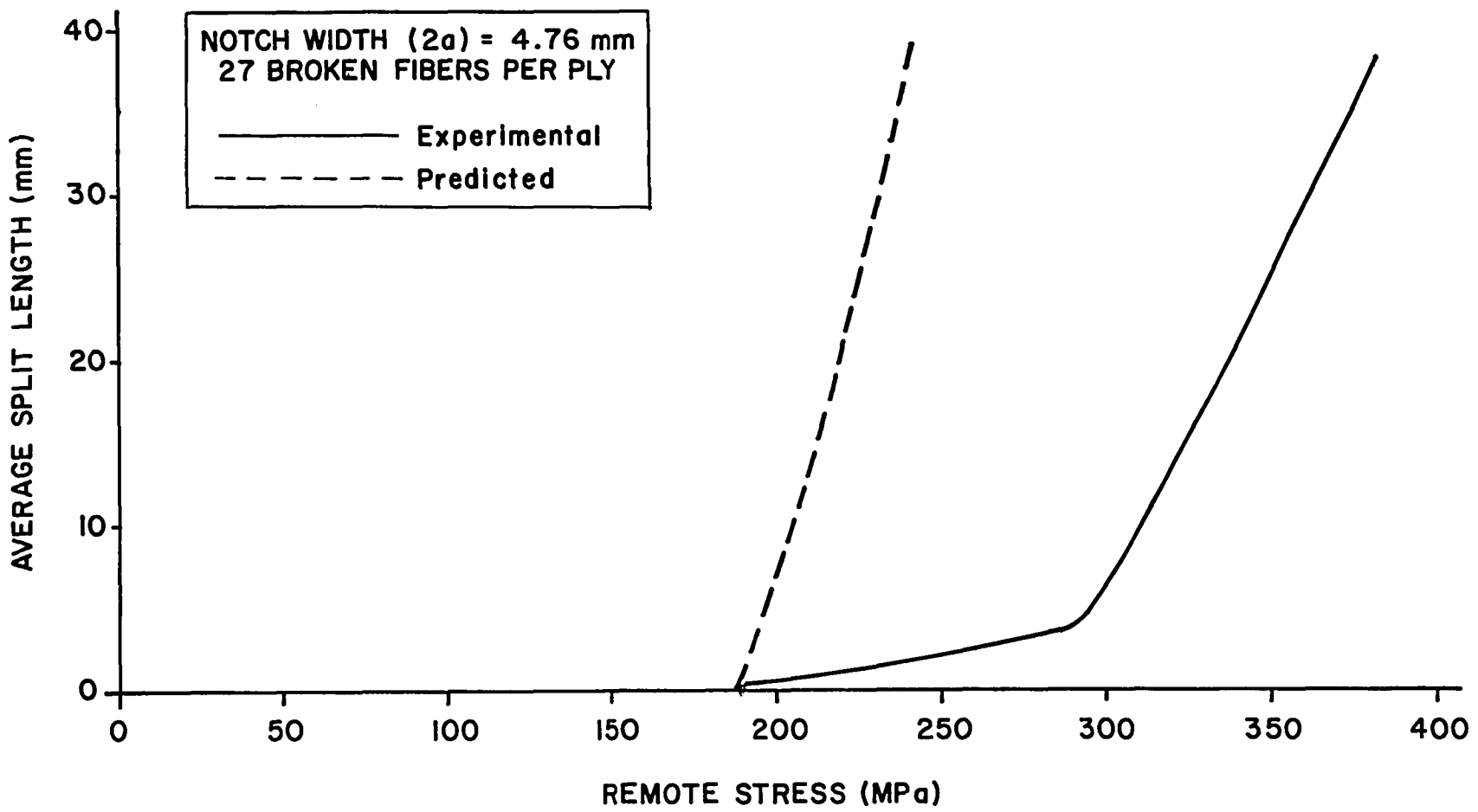
Figure 34. Average split length versus remote stress for 27 broken fibers: comparison of experimental and predicted behavior.
