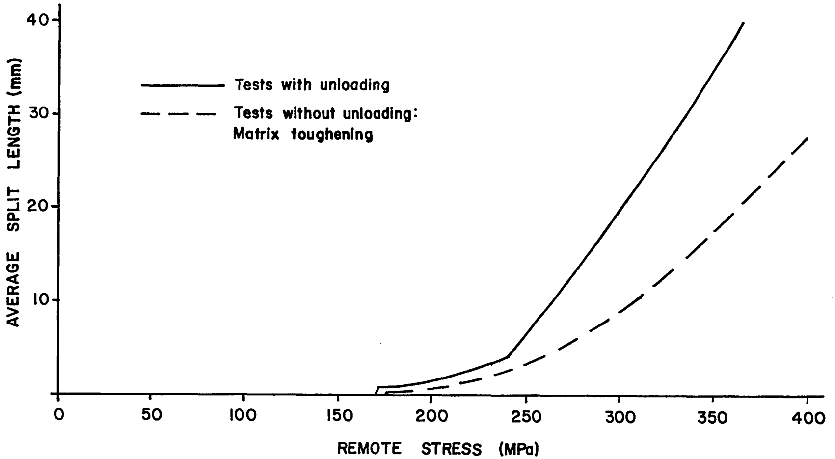
Figure 37. Experimental average split length versus remote stress for 37 broken fibers: comparison of test procedures.
