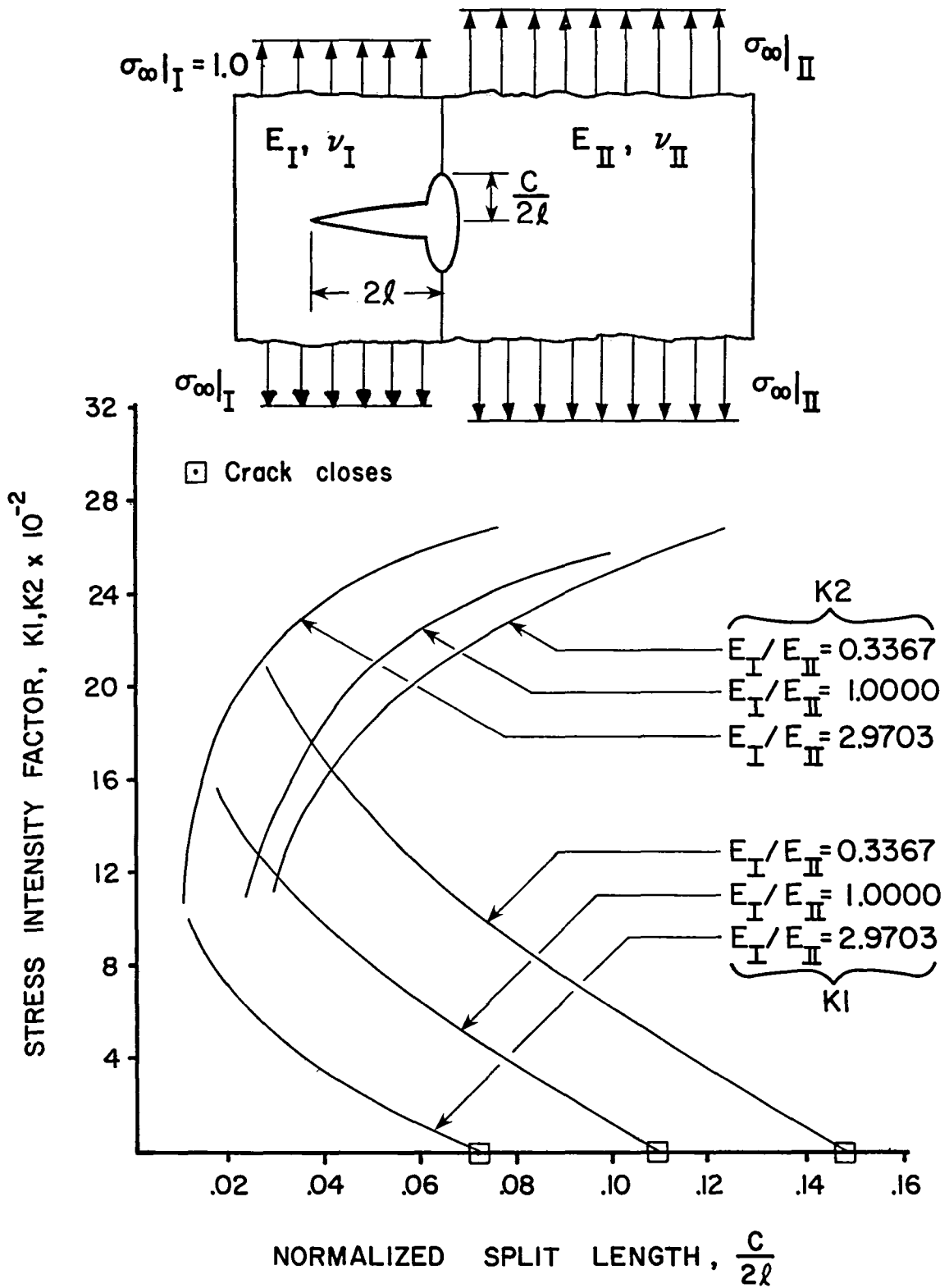
Figure 38. Stress intensity factors at the split tip, obtained from reference [28].
