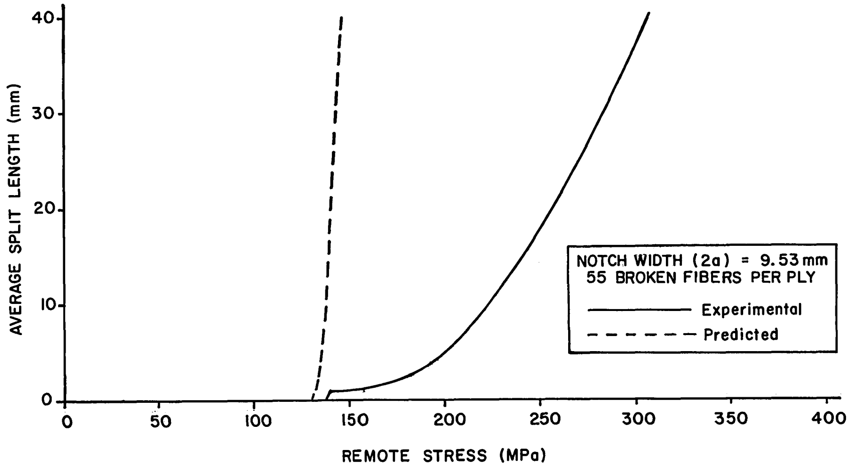
Figure 36. Average split length versus remote stress for 55 broken fibers: comparison of experimental and predicted behavior.
