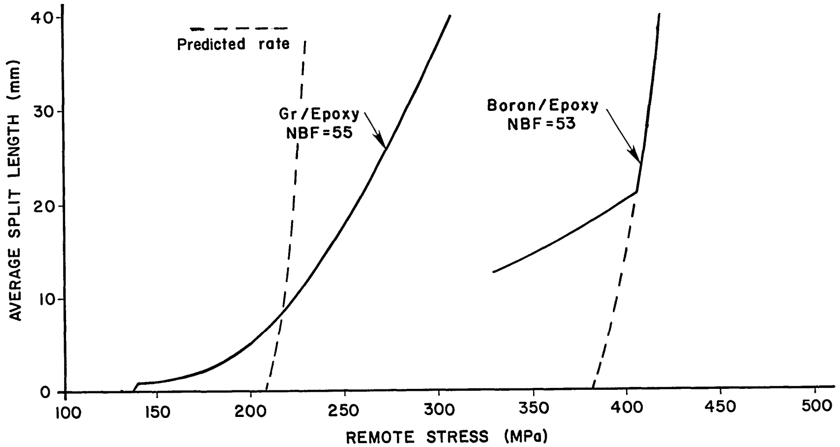
Figure 39. Average split length versus remote stress: comparison of graphite/epoxy and boron/epoxy split behavior to predicted split growth rates.
