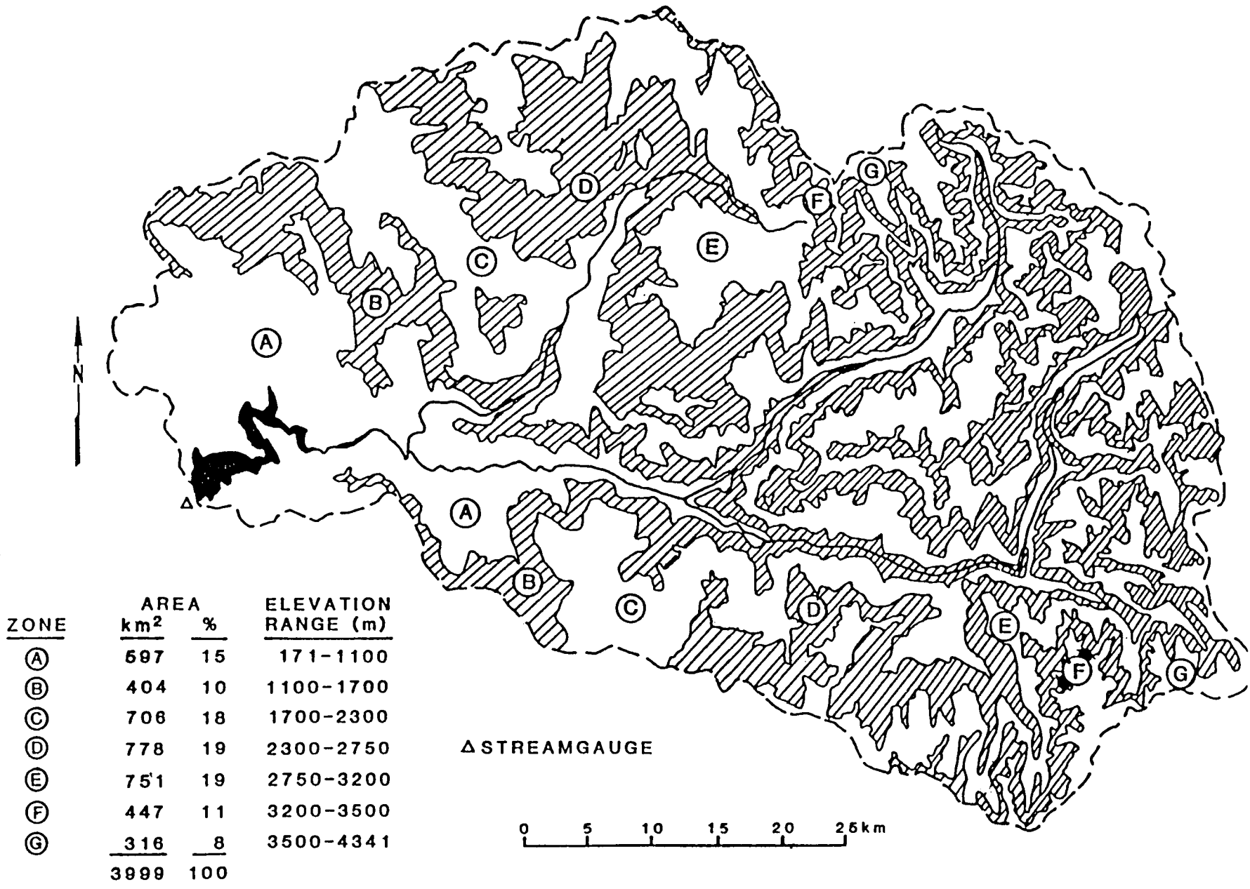
Figure 3. Elevation zones and areas of the Kings River Basin below Pine Flat Dam, California
