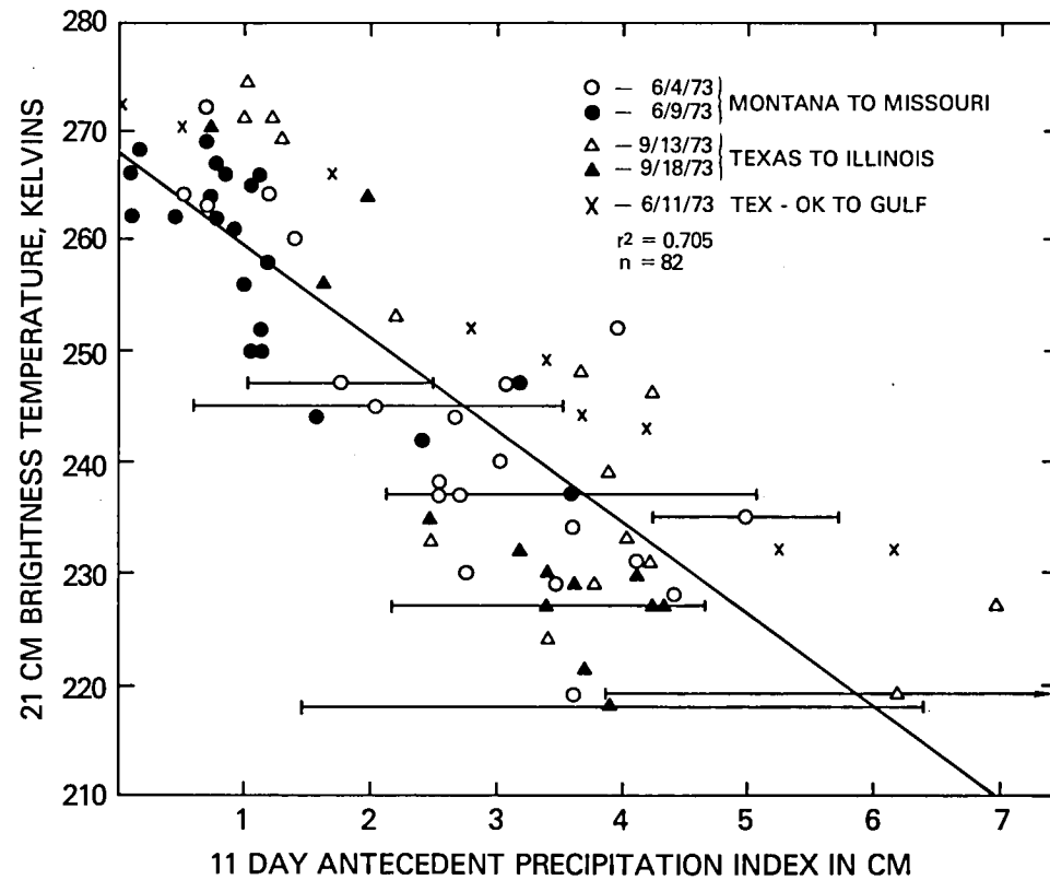
Figure 11. Satellite observations of T_B versus API.
