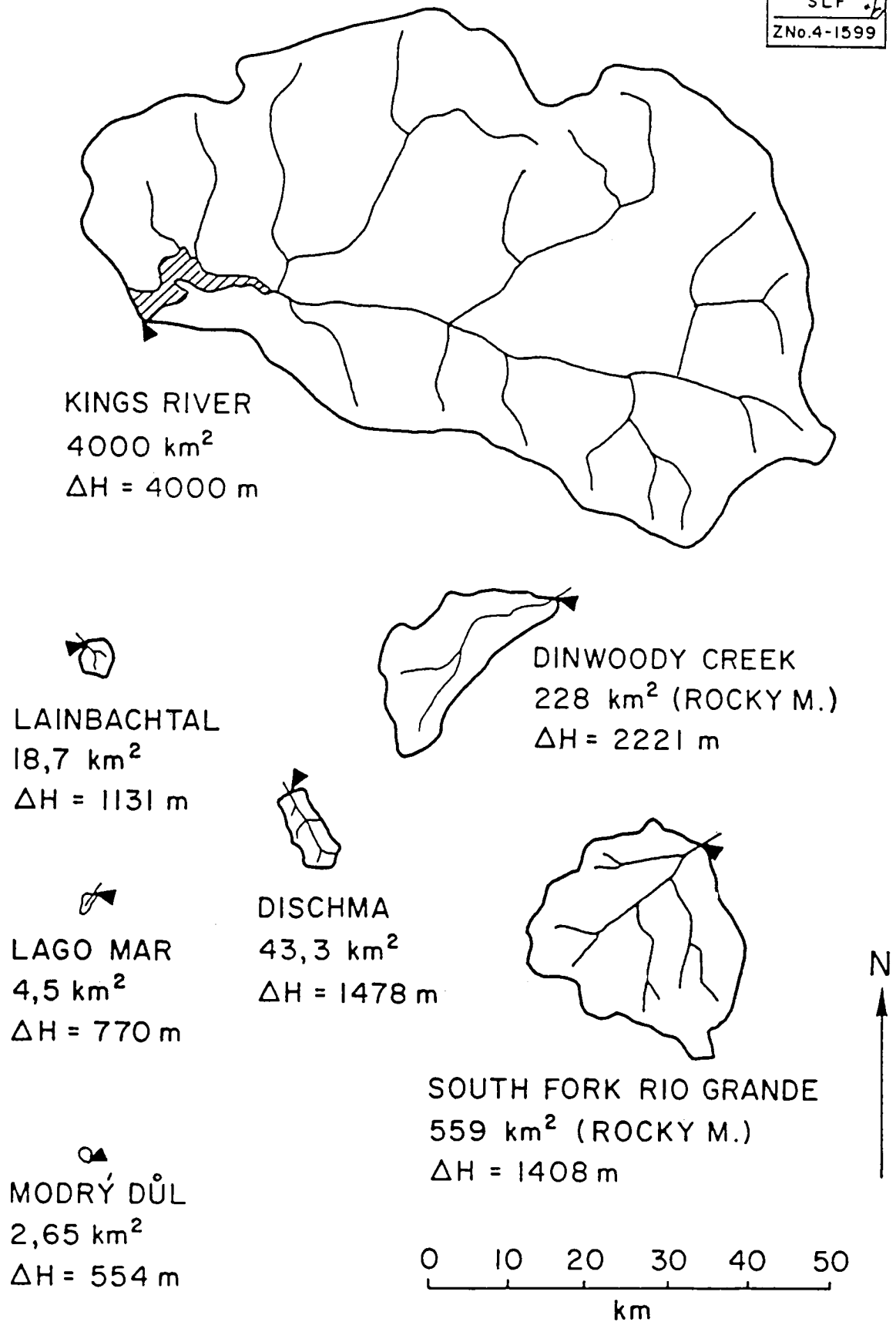
Figure 2. Size and elevation Range of some basins tested using SRM
