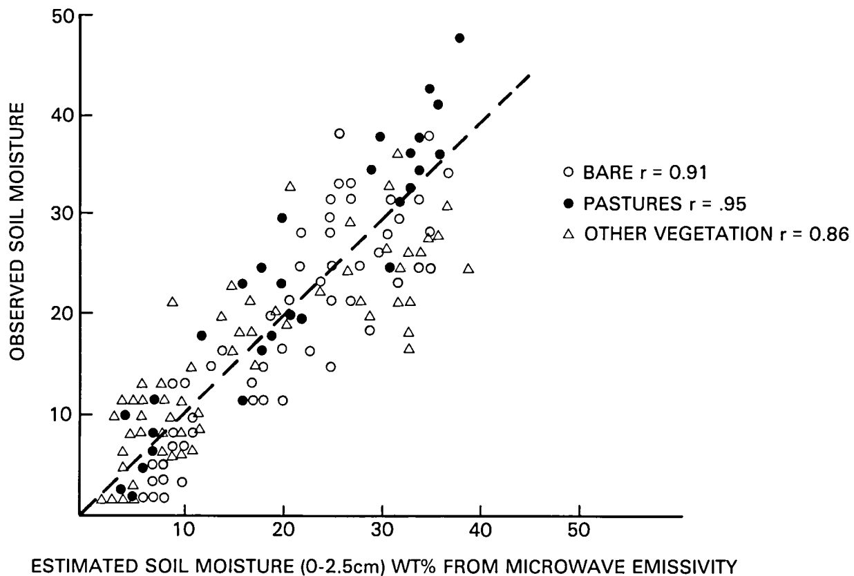
Figure 12. Comparison of measured and estimated values of soil moisture.
