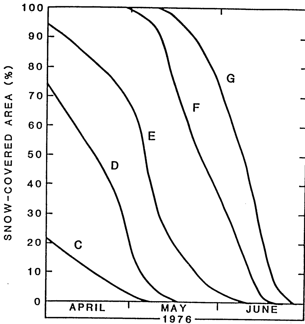
Figure 6. Landsat derived snow-cover depletion curves for elevation zones C, D, E, F and G in the Kings River Basin
