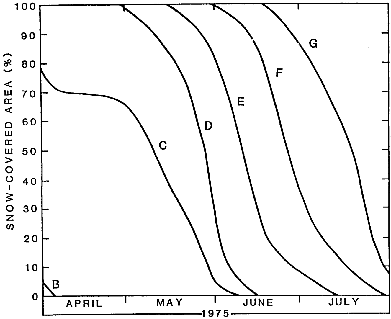
Figure 5. Landsat derived snow-cover depletion curves for elevation zones B, C, D, E, F and G in the Kings River Basin
