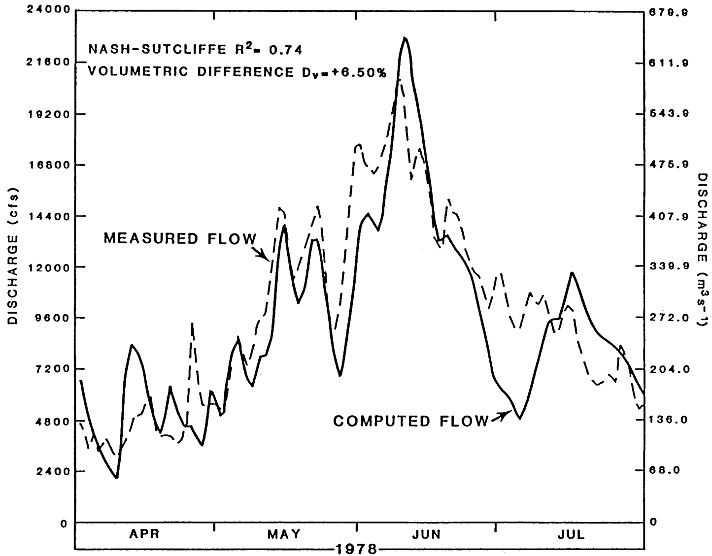
Figure 10. Discharge simulation for the Kings River Basin (3999 km 2 ), California using the snowmelt-runoff model
