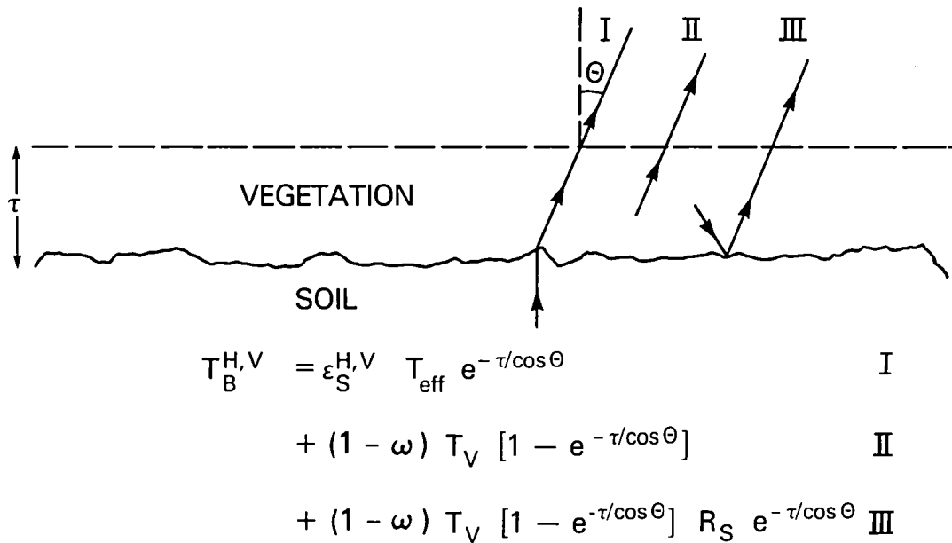
Figure 9. Schematic representation of the sources of microwave emission for a vegetated soil. For comparison L = \exp(+\tau) .
