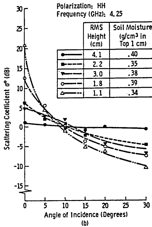
Figure 5. Angular variation of \sigma^0 in dB for 5 wet fields having RMS surface height variations as indicated. The measurements were made from a tower at the University of Kansas.
