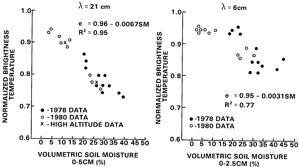
Figure 3. Observations of microwave emissivity at nadir from an aircraft at an altitude of 300 m.
