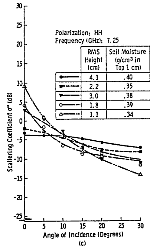
Figure 5. Angular variation of \sigma^0 in dB for 5 wet fields having RMS surface height variations as indicated. The measurements were made from a tower at the University of Kansas.
