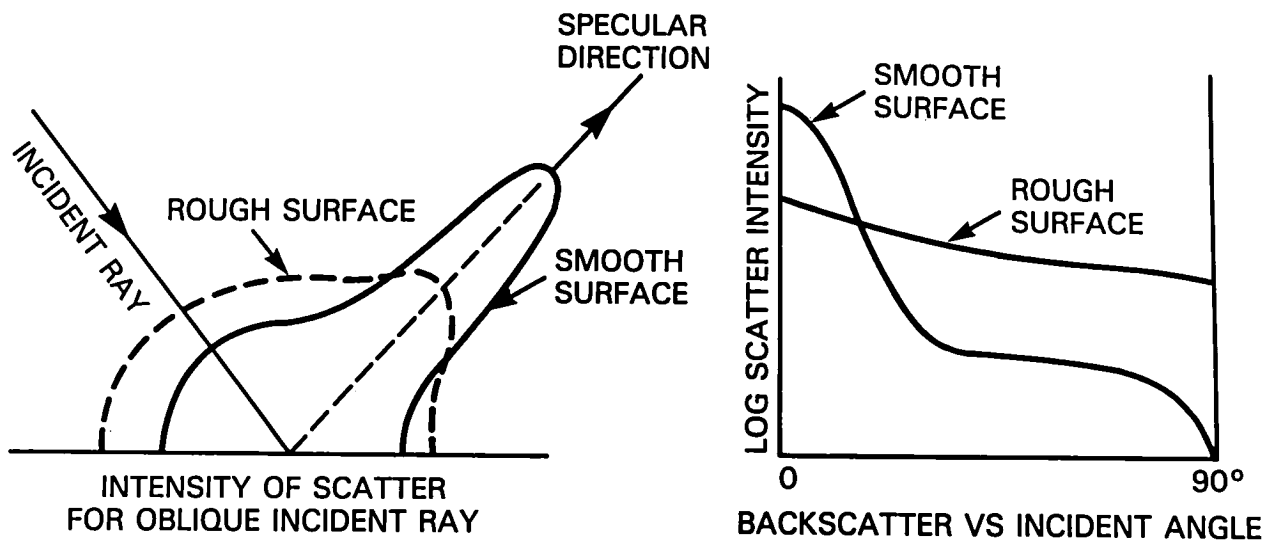
Figure 4. Schematic of radar intensity patterns showing the different behaviors of smooth and rough surfaces. The backscatter ( \sigma^\circ ) is the intensity in the direction of incidence.
