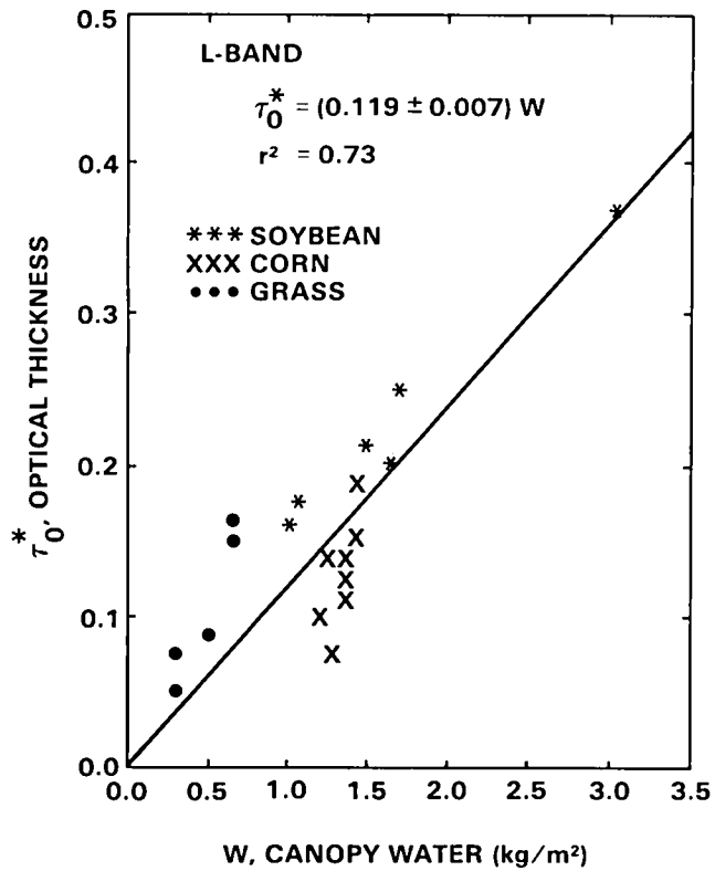
Figure 10. Variation of optical depth ( \tau ) with canopy water content for 3 crops. Results from tower measurements at 2 km.
