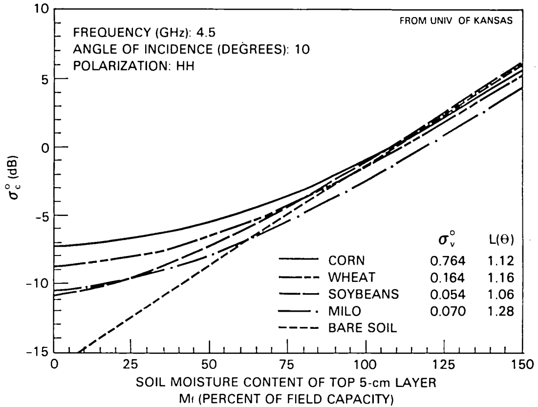
Figure 8. Variation of tower measurements of \sigma^0 for 4 crops.
