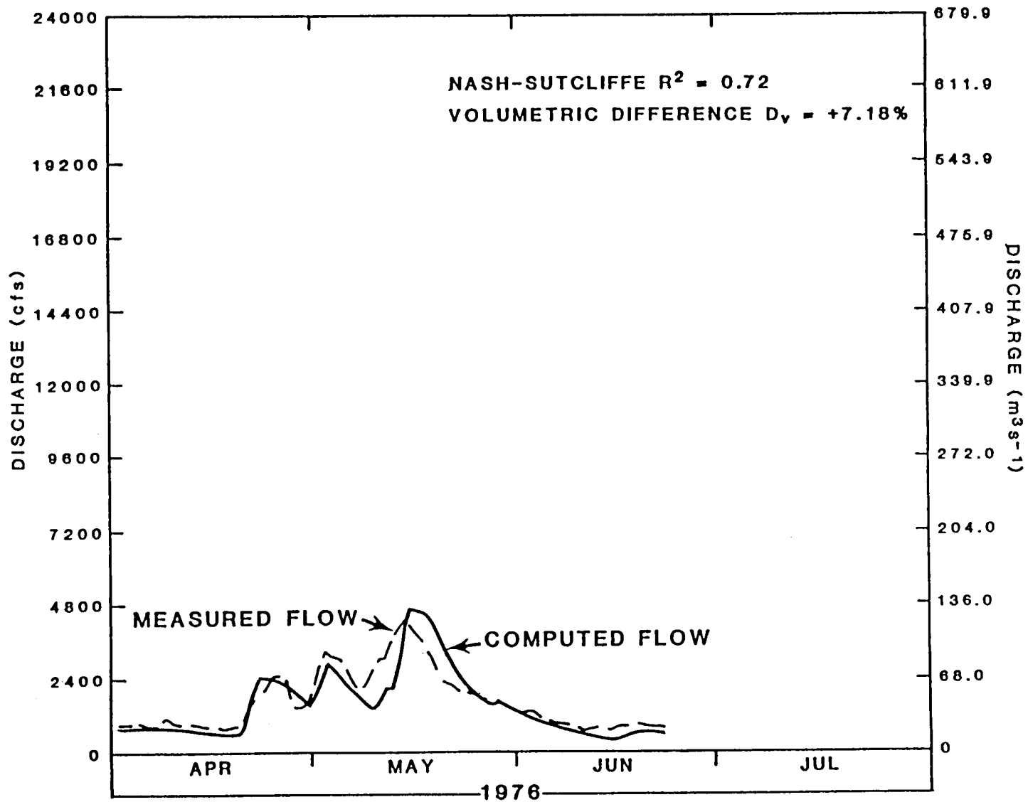
Figure 9. Discharge simulation for the Kings River Basin (3999 km 2 ), California using the snowmelt-runoff model
