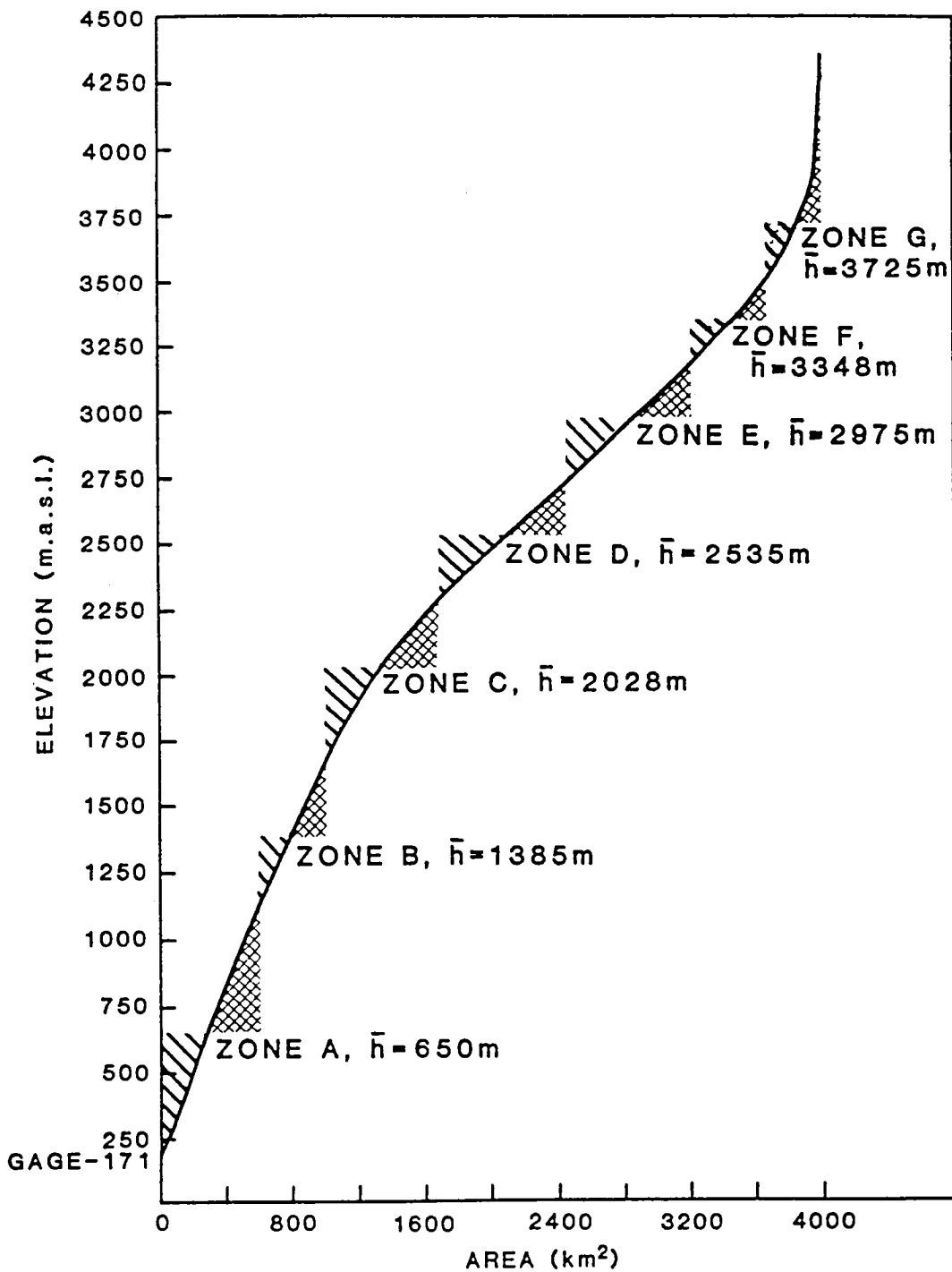
Figure 4. Determination of zonal mean hypsometric elevations ( \bar{h} ) using an area-elevation curve for the Kings River Basin, California
