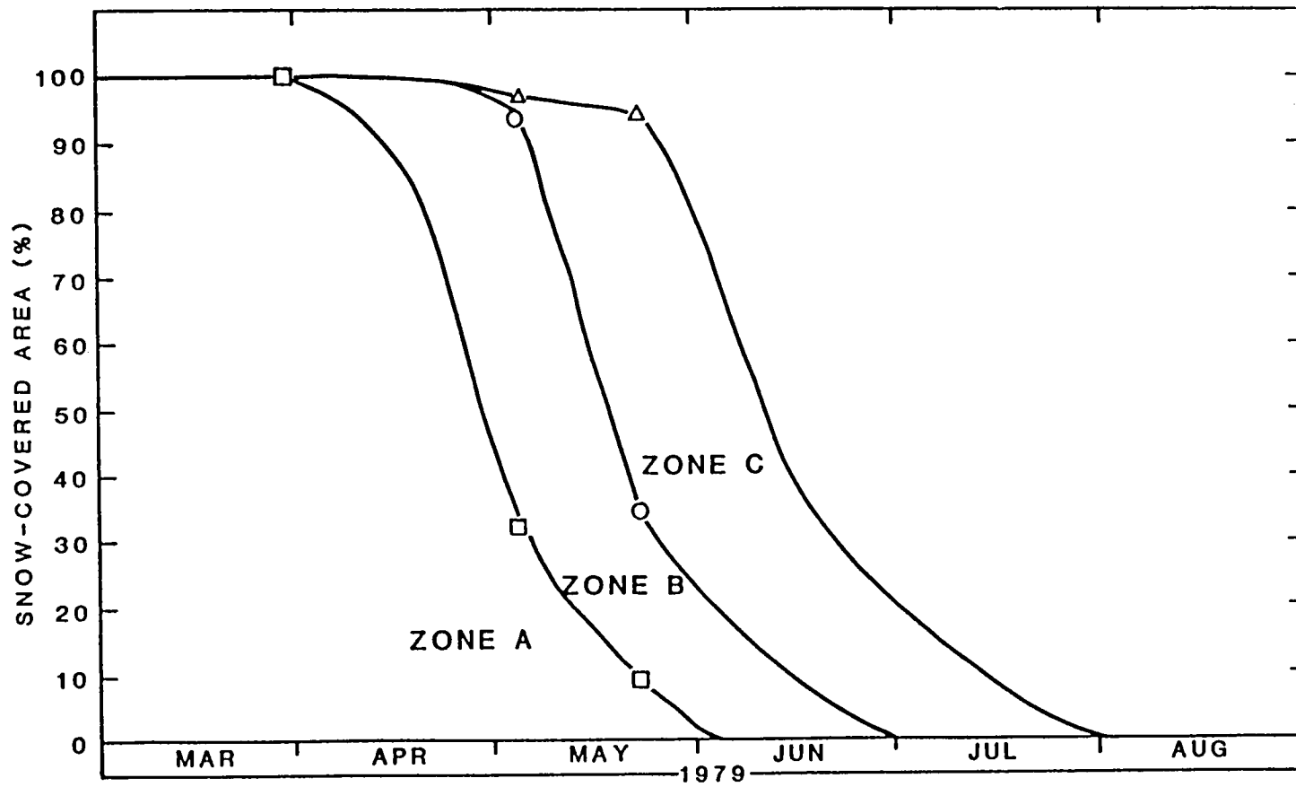
Figure 13. Landsat derived snow-cover depletion curves for elevation zones A, B and C in the Okutadami Basin
