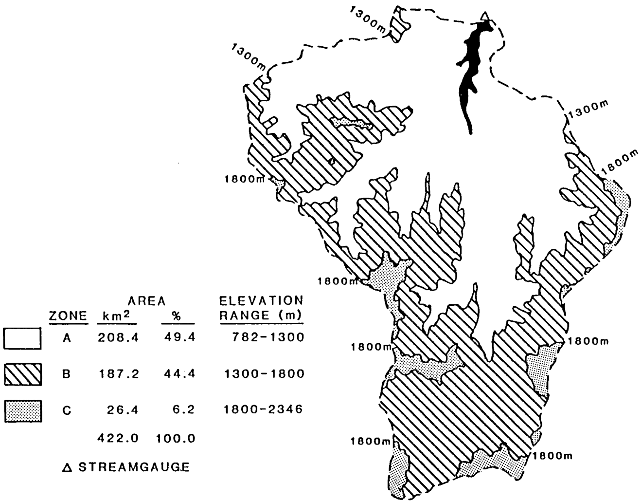
Figure 11. Elevation zones and areas of the Okutadami Basin, Japan
