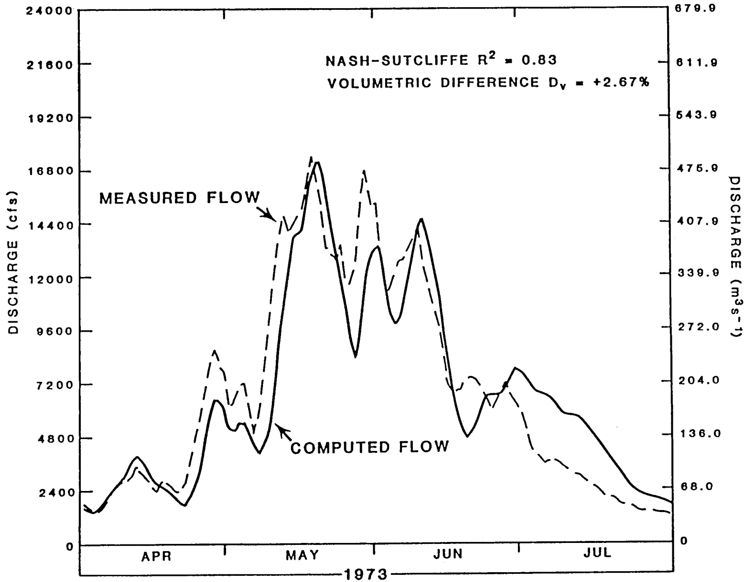
Figure 7. Discharge simulation for the Kings River Basin (3999 km 2 ), California using the snowmelt-runoff model
