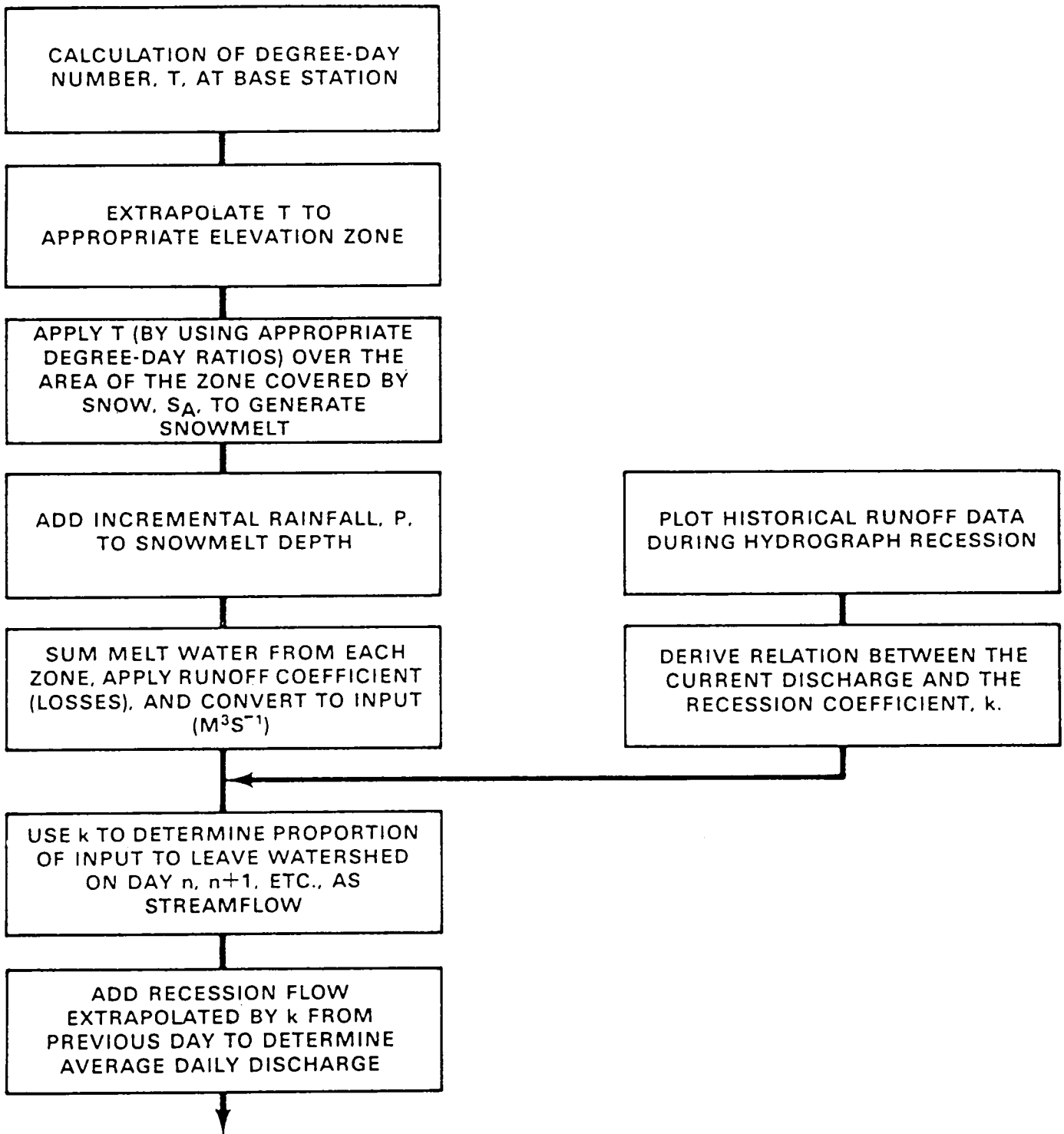
Figure 1. Flow Diagram for Snowmelt Runoff Model
