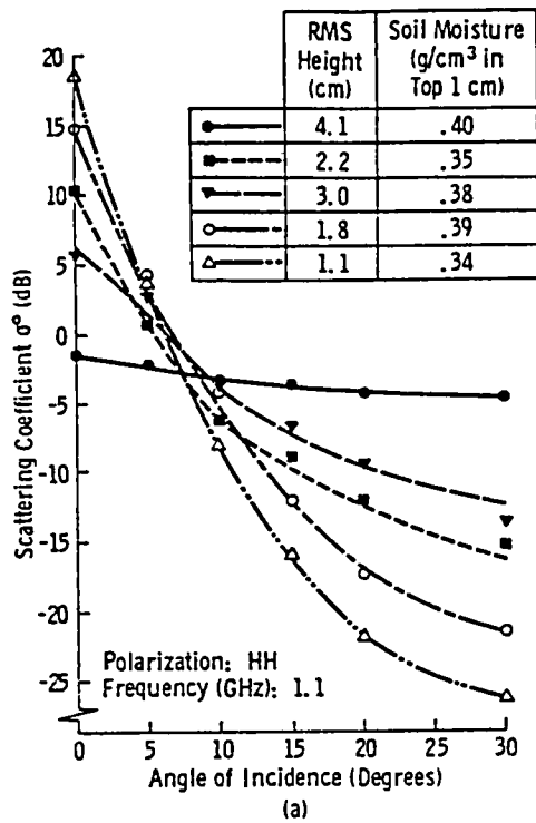
Figure 5. Angular variation of \sigma^0 in dB for 5 wet fields having RMS surface height variations as indicated. The measurements were made from a tower at the University of Kansas.
