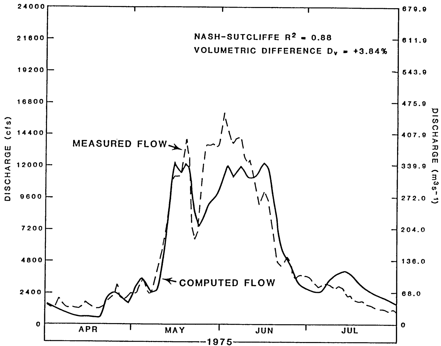
Figure 8. Discharge simulation for the Kings River Basin (3999 km 2 ), California using the snowmelt-runoff model
