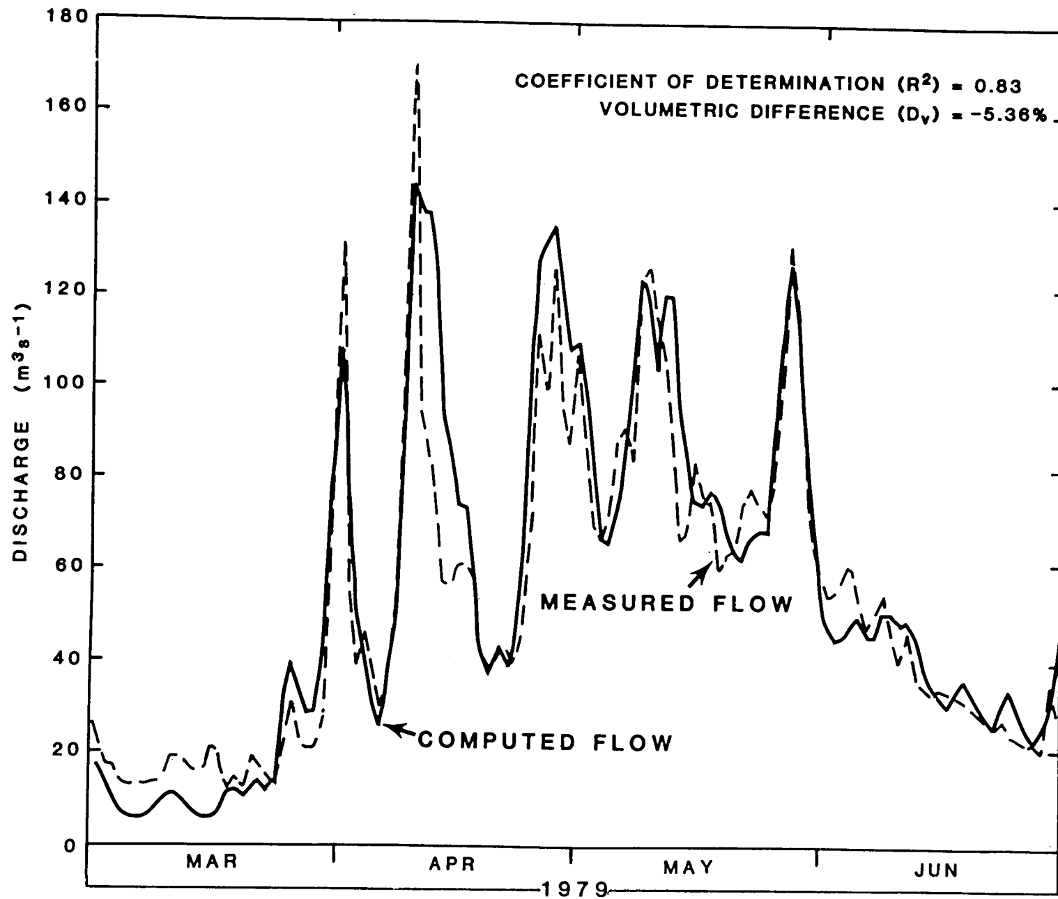
Figure 14. Discharge simulation for the Okutadami Basin ( 422 \text{ km}^2 ), central Japan using the snowmelt-runoff model
