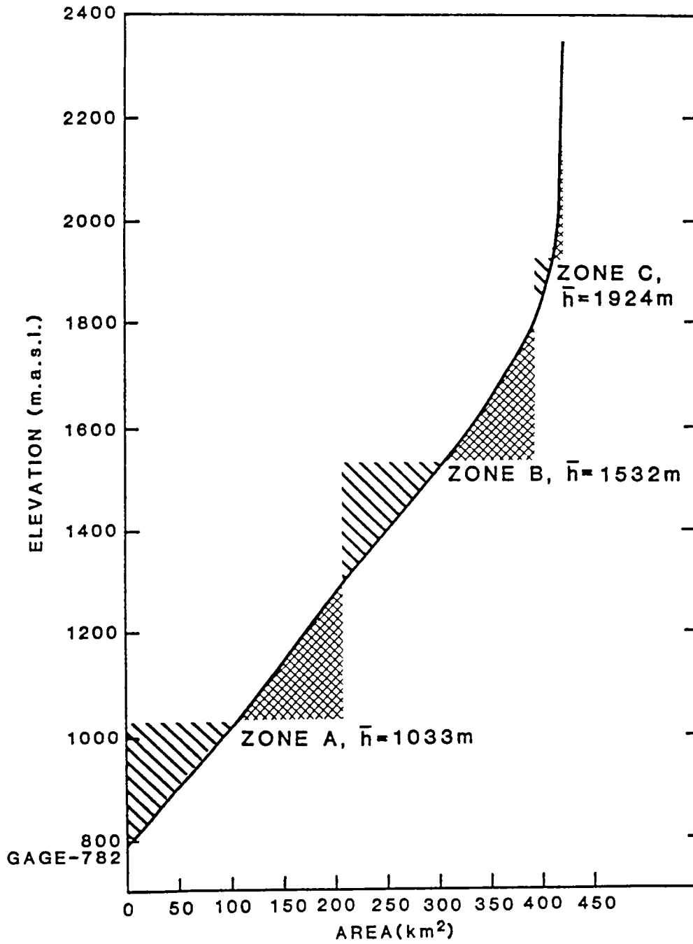
Figure 12. Determination of zonal mean hypsometric elevations ( \bar{h} ) using an area-elevation curve for the Okutadami Basin, Japan
