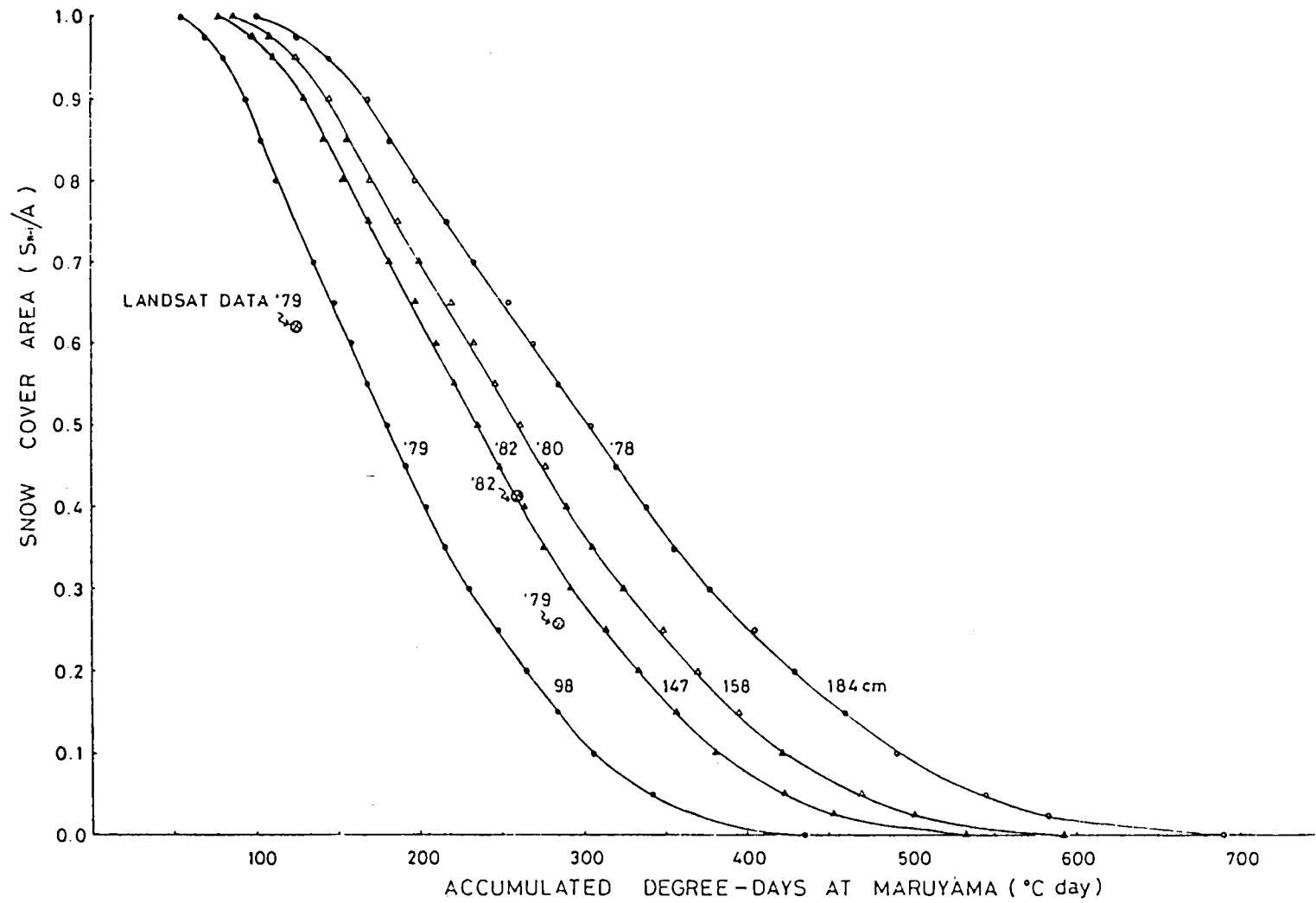
Figure 7. Relationship Between Depletion of Snow Cover Area and Accumulated Degree Days at Maruyama (Parameter: Basin-Wide Snow Amount at Maximum Stage)
