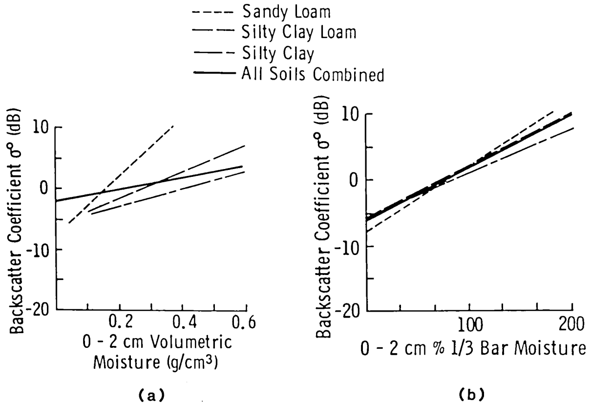
Figure 6. Regression results of tower measurements of \sigma^0 vs. soil moisture.
