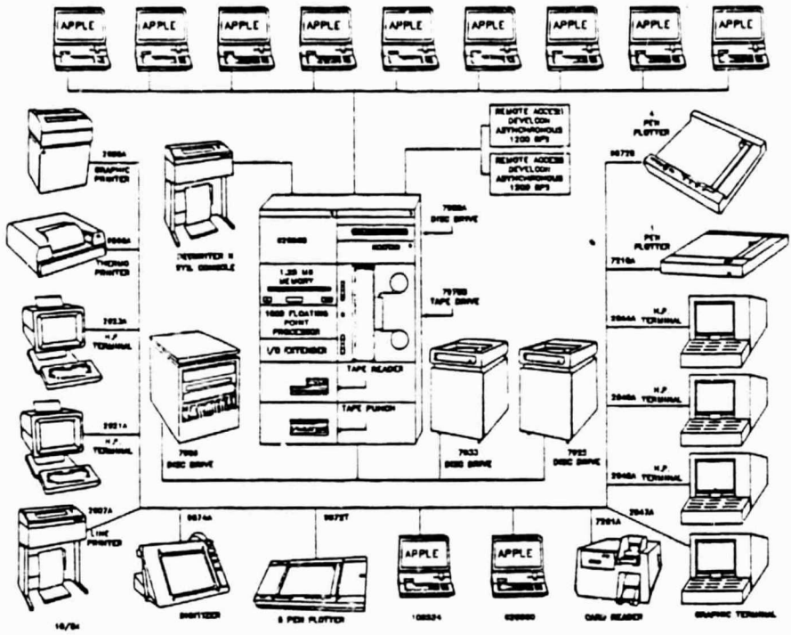
Figure 3-1. Hewlett Packard 1000F Computer System
