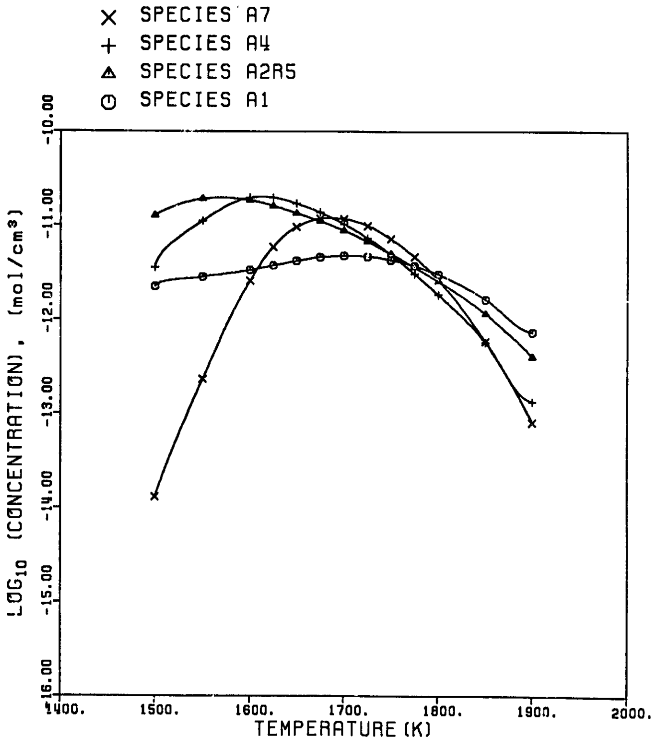
Figure 63. Temperature dependence of computed concentrations of intermediate- and large-sized aromatic molecules for the test case at a reaction time of 0.5 ms. The structure for each species is presented in Table II. The symbols designate computational results, the lines cubic spline fits.
