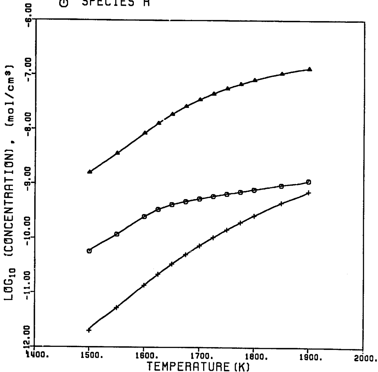
Figure 59. Temperature dependence of computed concentrations of H, H 2 and H eq for the test case at a reaction time of 0.5 ms. H eq is the hypothetical concentration of hydrogen atoms which would be in equilibrium with the computed concentration of H 2 . The symbols designate computational results, the lines cubic spline fits.
