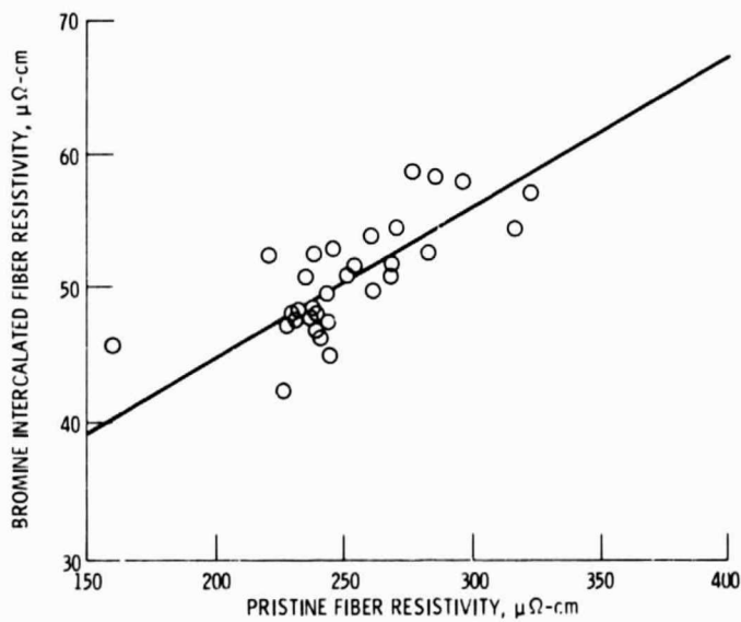
Figure 4. - Resistivity of Bromine intercalated fiber as a function of Pristine fiber resistivity.
