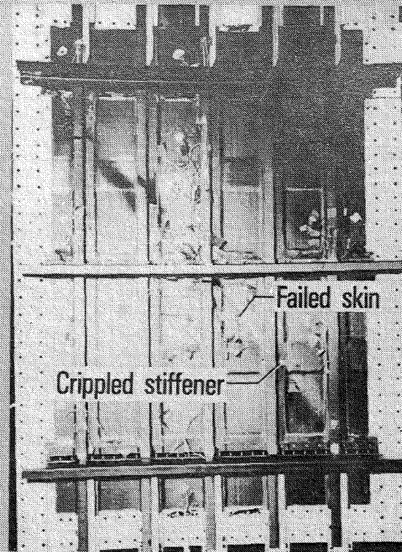
FAILED SPECIMEN
