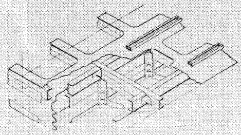
Corrugated beam/notched corner concept
