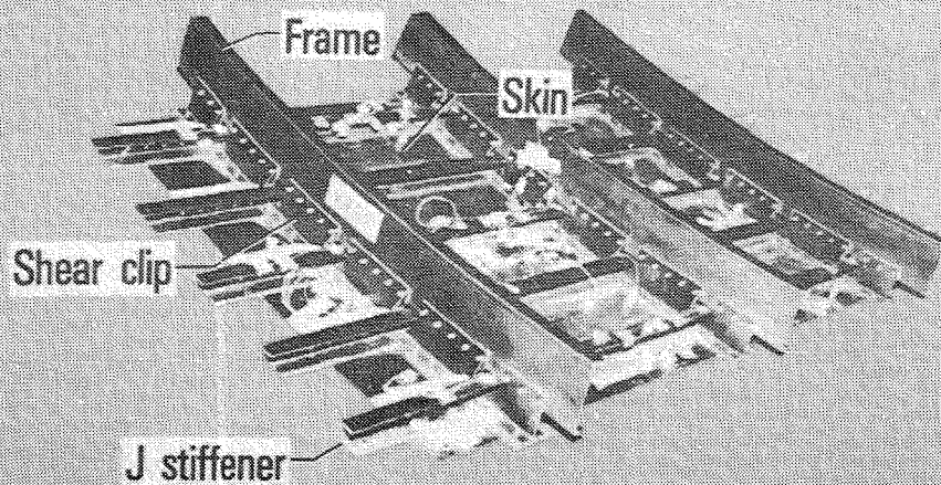
TYPICAL SPECIMEN
