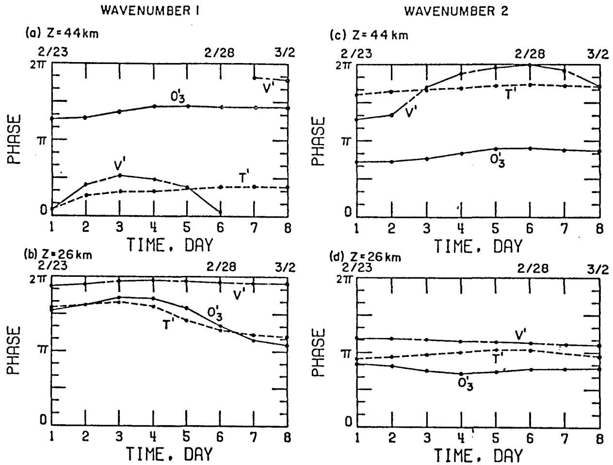
FIG. 5.10: The time variation of the phase relationship between ozone (solid line), temperature (dashed line), and eddy meridional velocity (solid and dashed line) waves during the late February 1979 warming. Phase increases westward. (a) Wavenumber 1 at altitude 44 km; (b) Wavenumber 1 at 26 km; (c) Wavenumber 2 at 44 km; and, (d) Wavenumber 2 at 26 km.
