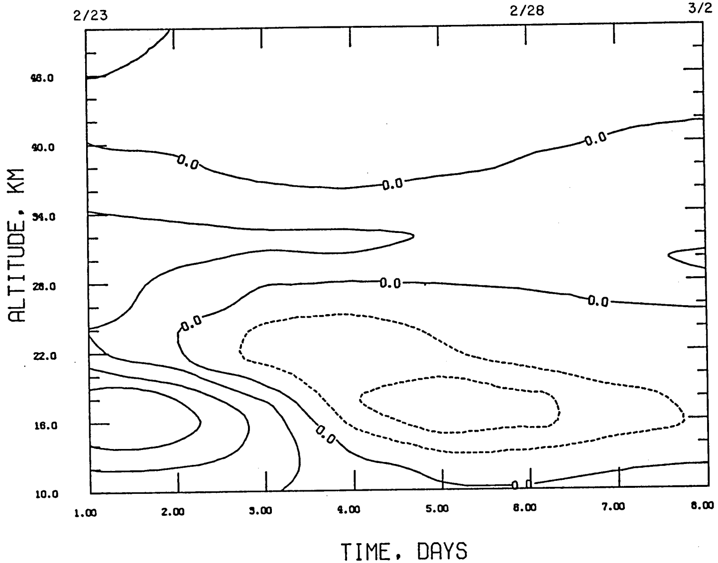
FIG. 5.7b: Time variations of eddy ozone mass transport, in unit molecule \text{cm}^{-3} \text{ms}^{-1} , due to wavenumber 2, contour interval 1. Molecule \text{cm}^{-3} \text{ms}^{-1} . Scaled by 10^{-12} .
