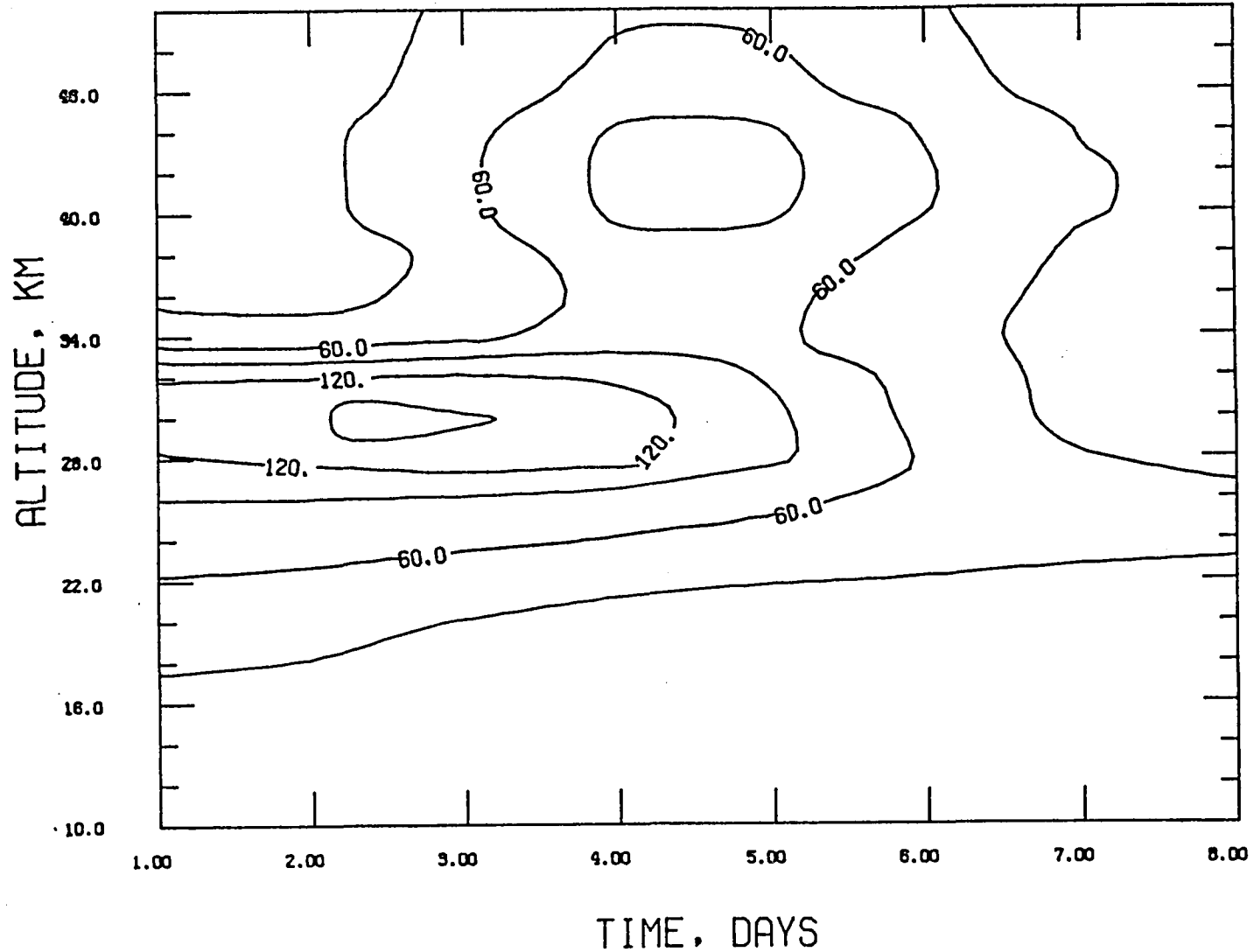
FIG. 5.8c: Time variation of eddy heat flux, sum of the first three waves, contour interval 30^{\circ}\text{C ms}^{-1} , in unit ^{\circ}\text{K ms}^{-1} .
