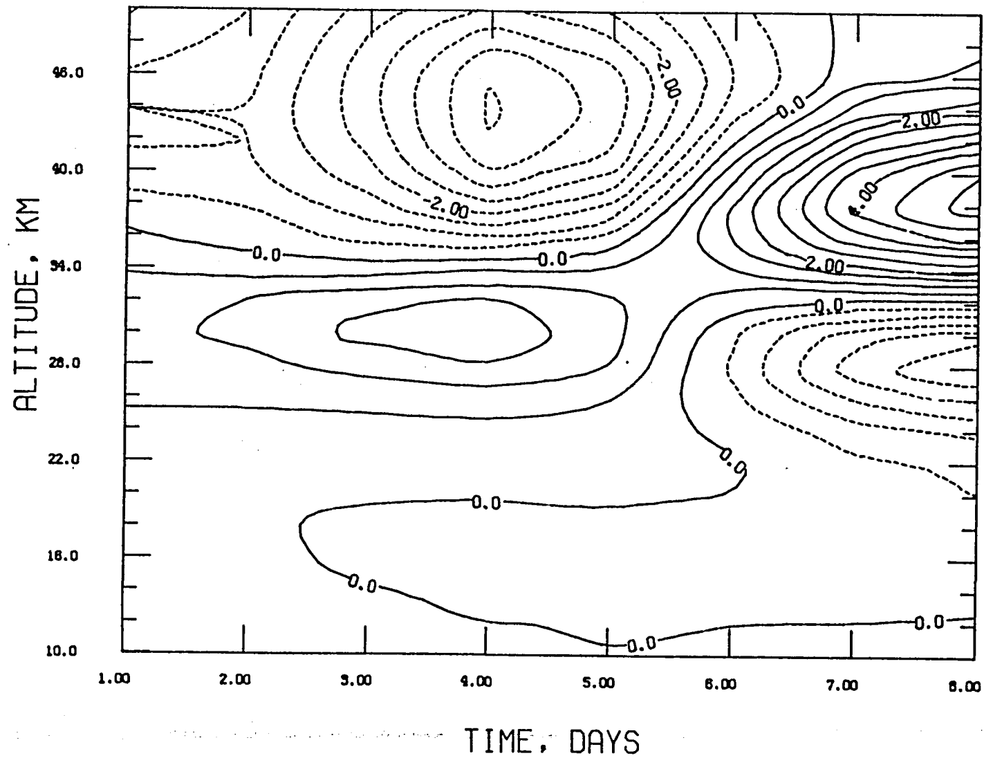
FIG. 5.6a: Time variations of eddy ozone flux, in unit ppm ms -1 , due to wavenumber 1, contour interval 1 ppm ms -1 .
