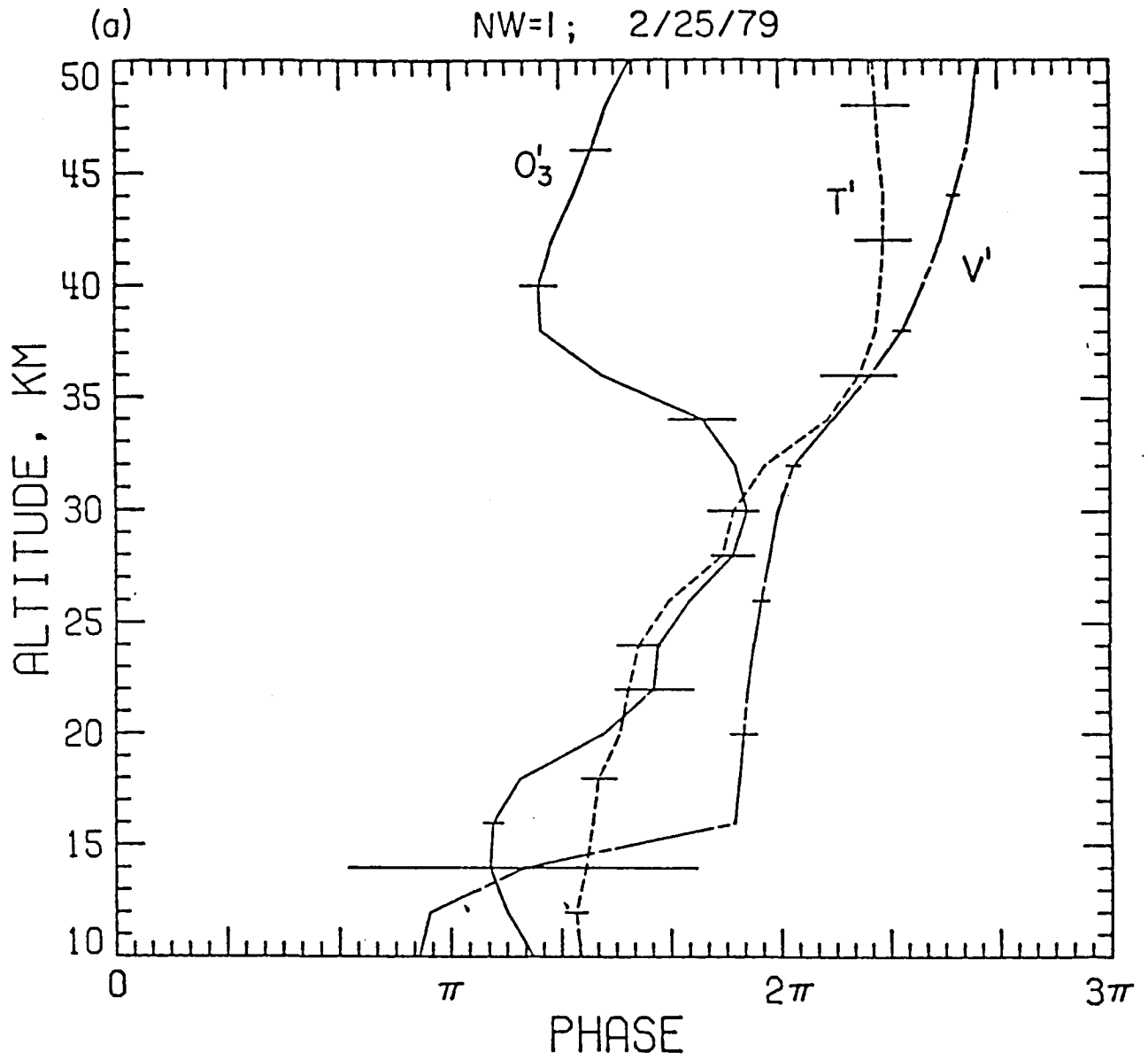
FIG. 5.9a: The phase relationship between ozone (solid line), temperature (dashed line), and eddy meridional velocity (solid and dashed line) for wavenumber 1, February 25, 1979. Phase increases westward.
