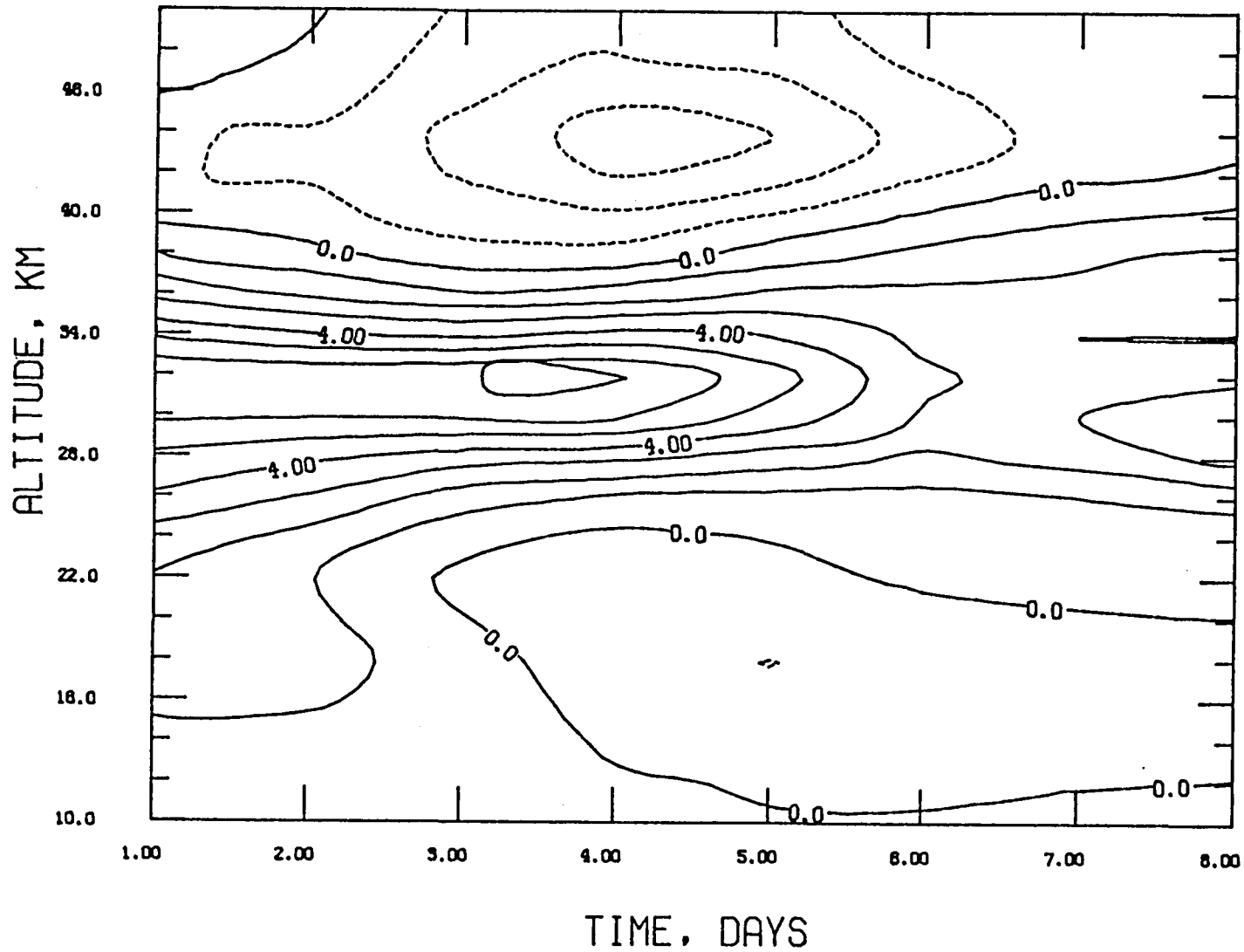
FIG. 5.6b: Time variations of eddy ozone flux, in unit ppm ms -1 , due to wavenumber 2, contour interval 2 ppm ms -1 .
