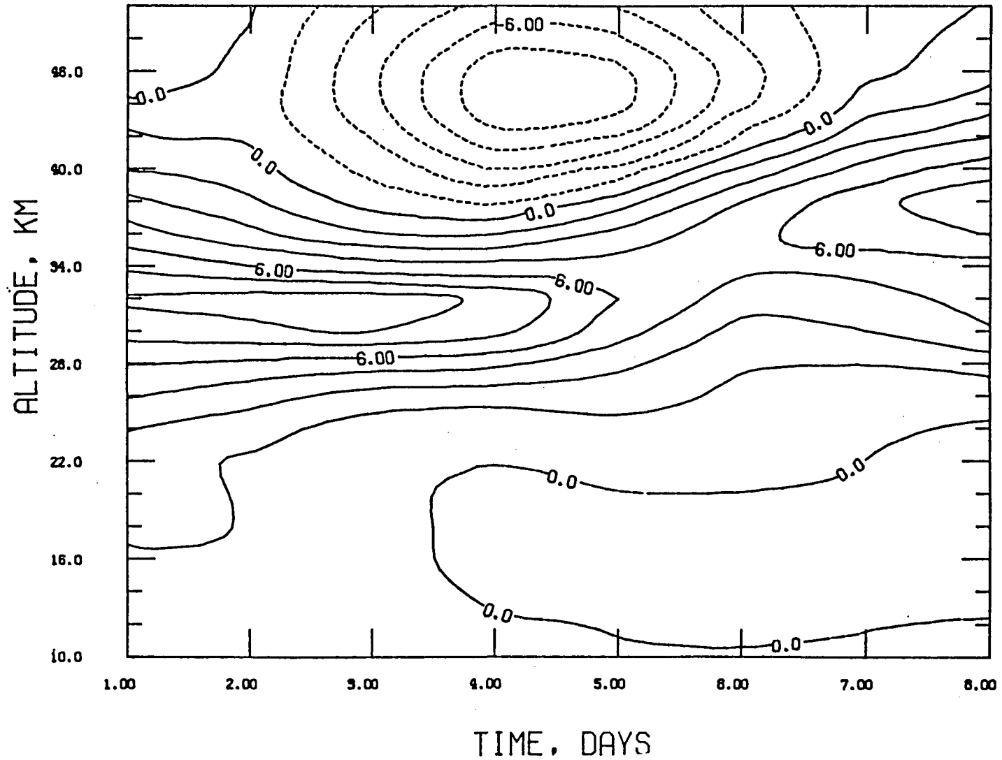
FIG. 5.6c: Time variations of eddy ozone flux (sum of the first three waves) in unit \text{ppm ms}^{-1} . Contour interval 3 \text{ ppm ms}^{-1} .
