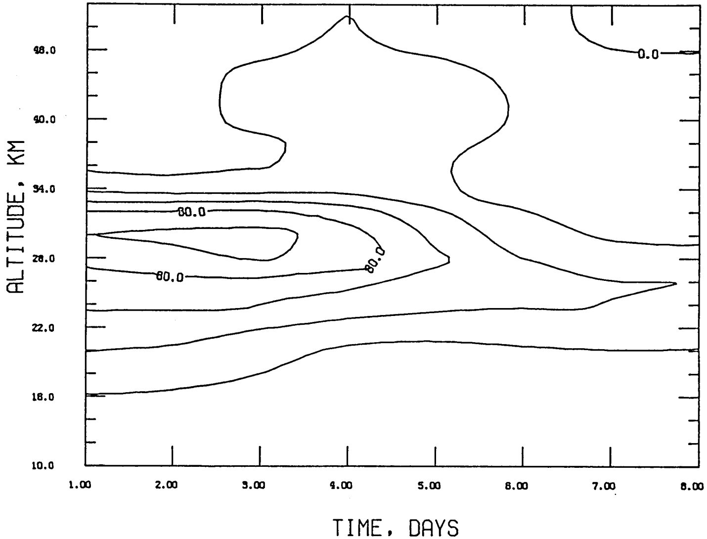
FIG. 5.8b: Time variation of eddy heat flux, wavenumber 2, contour interval 20°C ms -1 , in unit °K ms -1 .
