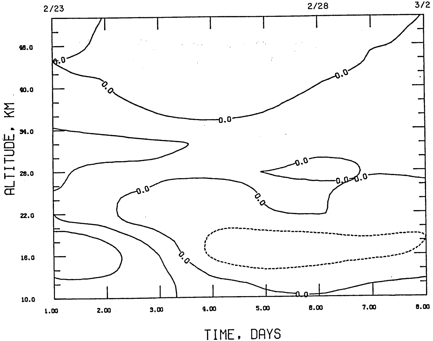
FIG. 5.7c: Time variations of eddy ozone mass transport (sum of the first three waves) in unit molecule \text{cm}^{-3} \text{ms}^{-1} . Contour interval 1.5 \text{ molecule cm}^{-3} \text{ms}^{-1} . Scaled by 10^{-12} .
