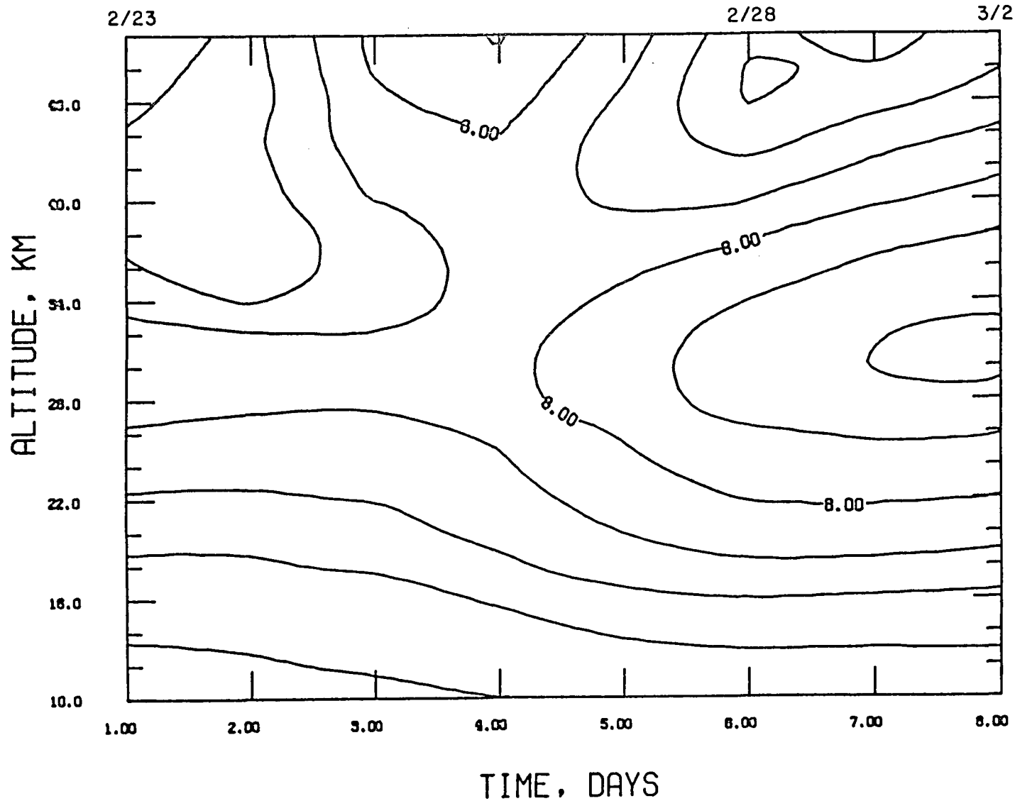
FIG. 5.3a: Evolution of the wavenumber 1 amplitudes (in unit m/s) of meridional velocity waves during the late February 1979 warming (~55°N). Contour interval 2 m/s.
