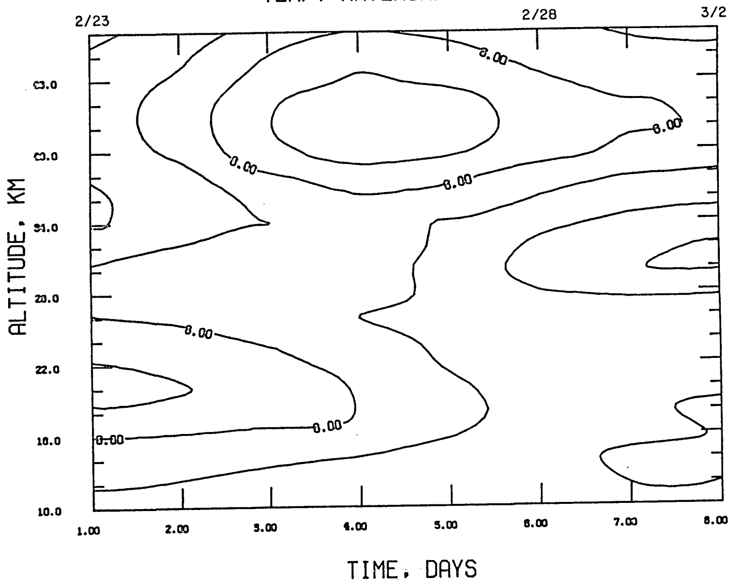
FIG. 5.2b: Evolution of the amplitudes (in unit ^{\circ}\text{C} ) of the temperature wavenumber 2 during the late February 1979 warming ( \sim 55^{\circ}\text{N} ). Contour interval 2^{\circ}\text{C} , zonal mean temperature, \text{K}^{\circ} (Contour interval 3^{\circ}\text{C} ).
