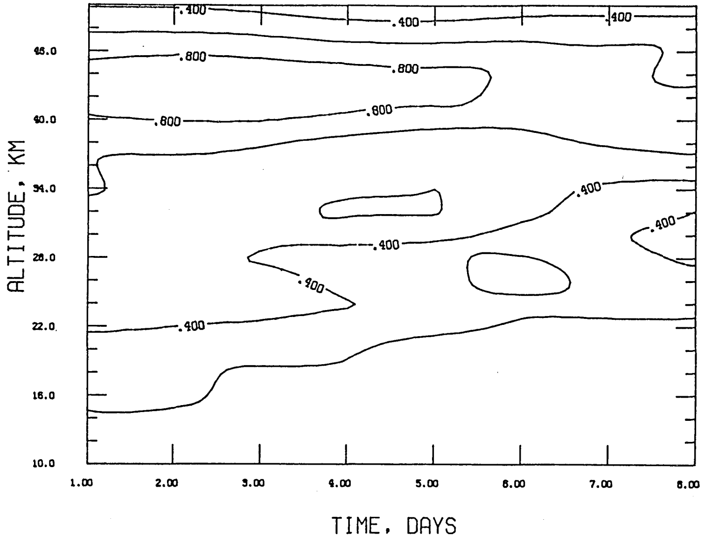
FIG. 5.4b: Evolution of the ozone wavenumber 2 amplitudes during the late February 1979 warming (in unit ppmv). Contour interval .2 ppmv.
