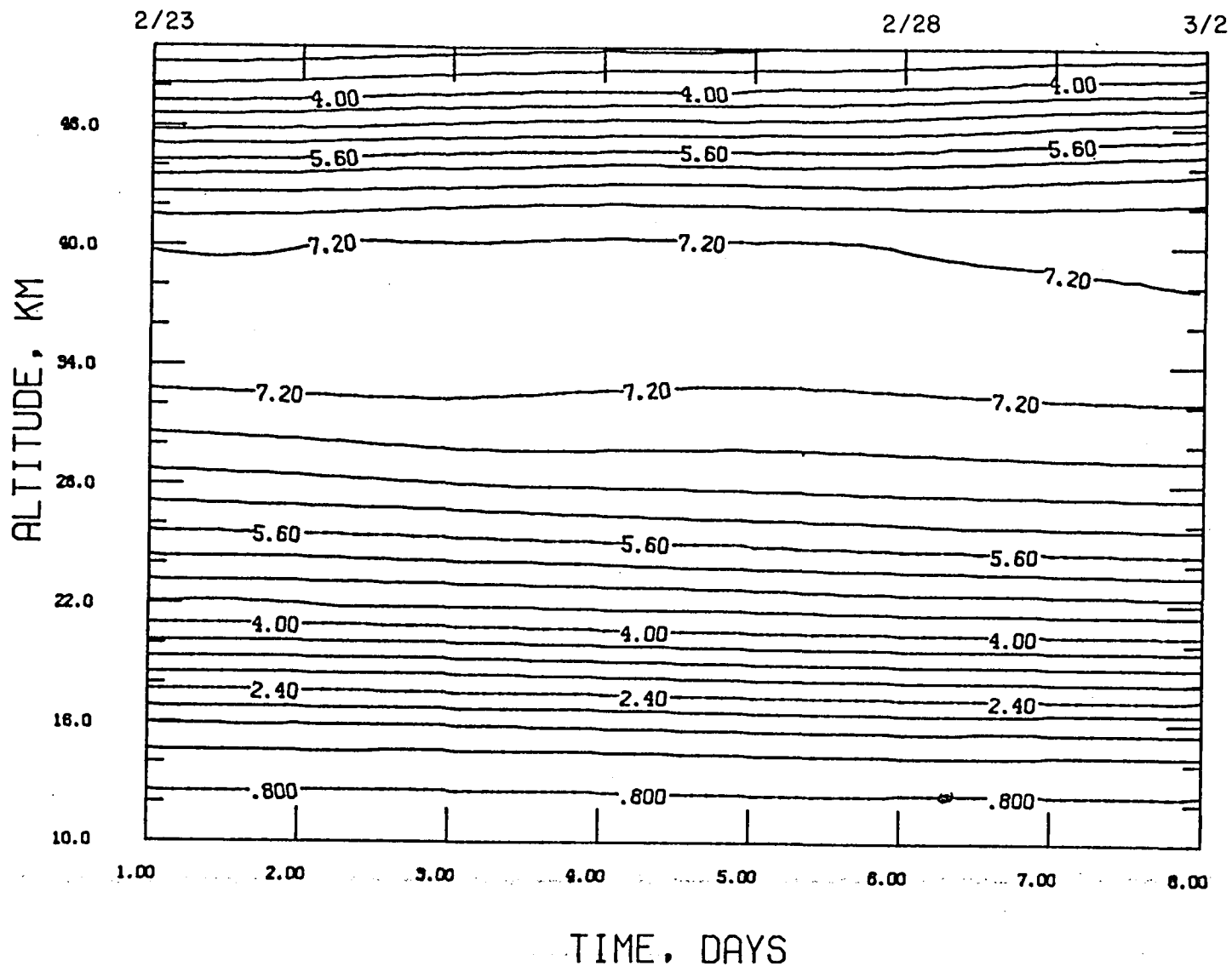
FIG. 5.4c: Evolution of zonal mean ozone during the late February 1979 warming (in unit ppmv). Contour interval .8 ppmv.
