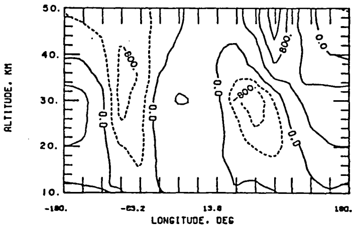
FIG. 5.1: Typical height-longitude distribution ( \sim 55^{\circ}\text{N} ) of (a) ozone mixing ratio, ppmv, contour interval 2 ppmv; (b) temperature, ^{\circ}\text{K} , contour interval 10^{\circ}\text{C} ; and, (c) height deviation, m, contour interval 400 m (February 25, 1979).
