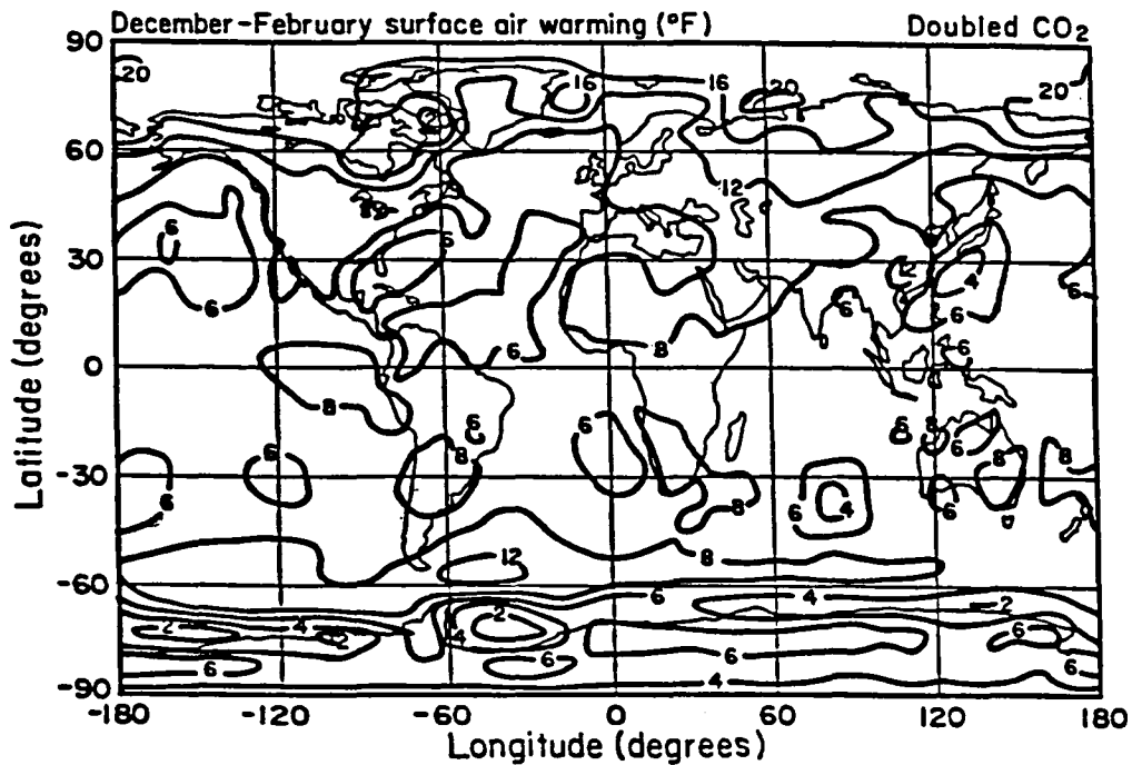
Fig. 4. Change in atmospheric surface air temperature during winter between the experiment with doubled \text{CO}_2 and the control run.
