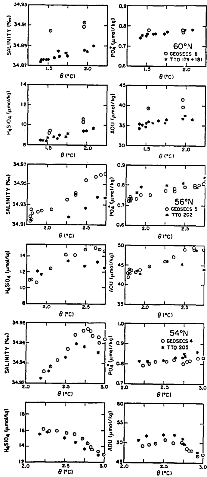
Fig. 2. Salinity, initial phosphate ( PO_4^{\circ} ), dissolved silica ( H_4SiO_4 ) and apparent oxygen utilization (AOU) for three GEOSECS stations and nearest TTO stations.
