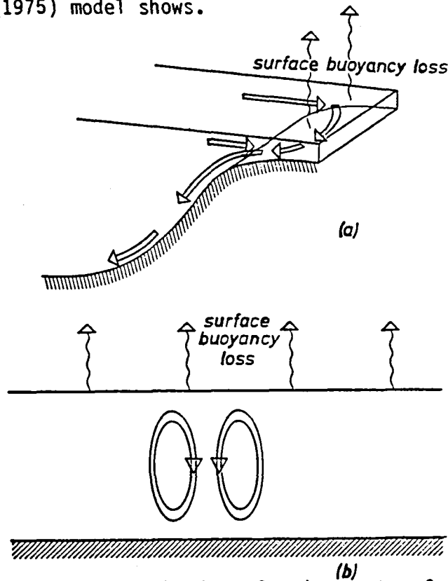
Fig. 1. Two basic mechanisms for deep water formation.
