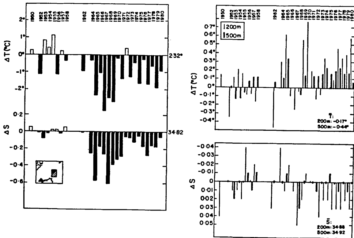
Fig. 3. Temperature and salinity anomalies in June within the rectangular area between 67^{\circ} and 69^{\circ}\text{N} , and 11^{\circ} and 15^{\circ}\text{W} referred to the 1950-1958 mean. Left: Variations 25 m; right: variations at 200 and 500 m. After Malmberg (1983).
