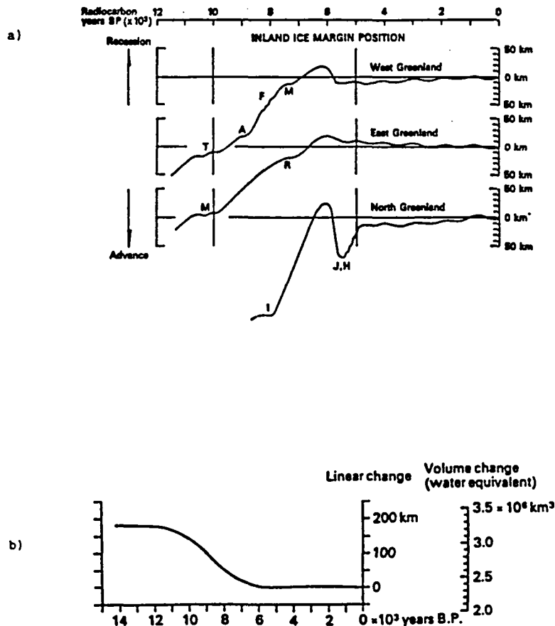
Fig. 3. a) Ice margin fluctuations in Greenland since 12000 B.P. (from Weidick, 1975b). b) Average recession of the Greenland Ice Sheet margin. The recession is also converted to volume shrinkage (from Weidick, 1975a).
