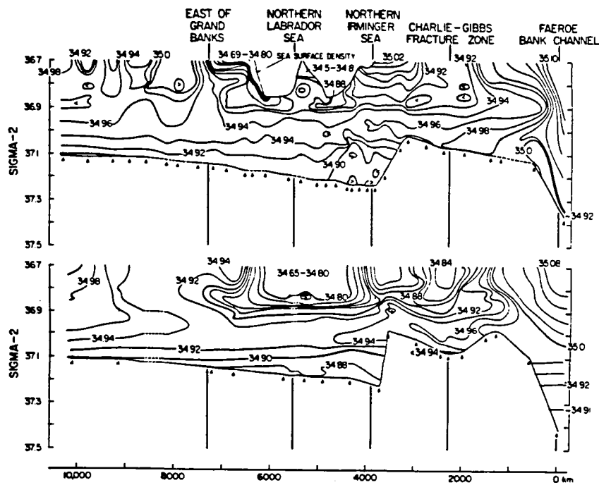
Fig. 2. Sections of salinity ( \times 10^3 ) versus \sigma_2 on a long, winding path from the Faeroe Bank Channel to the waters off the U.S. east coast (location shown in Figure 3). The upper section is drawn from a composite of historical data (Chain, 1960 and 1972; Crawford, 1960 and 1965; Erika Dan, 1962; Atlantis, 1964; Hudson, 1967; Knorr, 1972 and 1976) and the lower section is drawn from April-October 1981 TTO/NAS data. The only post-1972 data in the upper section is a single Knorr 1976 station in the Faeroe-Shetland Channel. The 1981 data from layers where \sigma_2 > 36.9 show an average freshening of ca. 0.02 \times 10^{-3} , and since layer densities are about the same, there was also a cooling of ca. 0.15^{\circ}\text{C} . The principal deep layers are LSW, near \sigma_2 = 36.9 , NEADW or Iceland-Scotland overflow water, near \sigma_2 = 37.0 , and NWABW or Denmark Strait overflow water, below 37.05 in the northwest Atlantic. All displayed the \theta -S shift. See Swift (1984a) for a more thorough discussion of this figure and related results.
