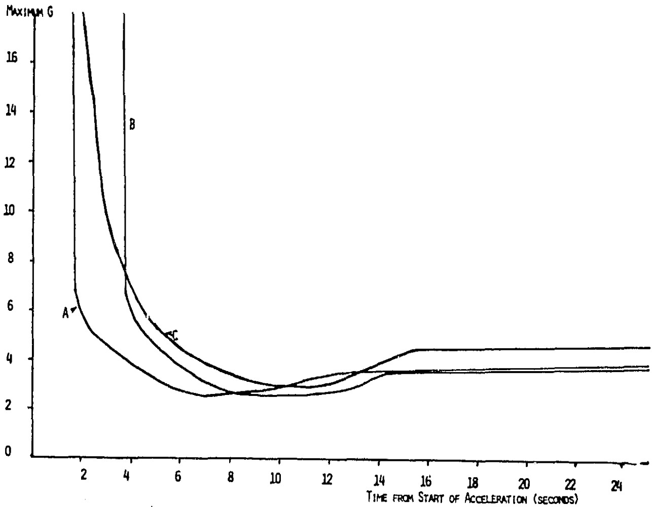
Figure 7: Comparison of experimental and simulated G-tolerance curves A. Simulated curve with PFI at SLOC of 60 mmHg B. Simulated curve with PFI at SLOC of 60 mmHg and with compensation for 2-second delay C. Curve generated from experimental data by Stoll (21)
