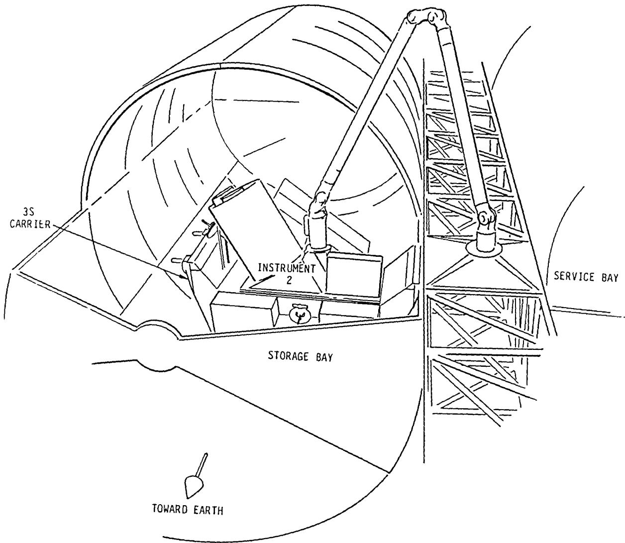
Figure 3-17. 3S Storage Carrier Installed in Storage Bay
