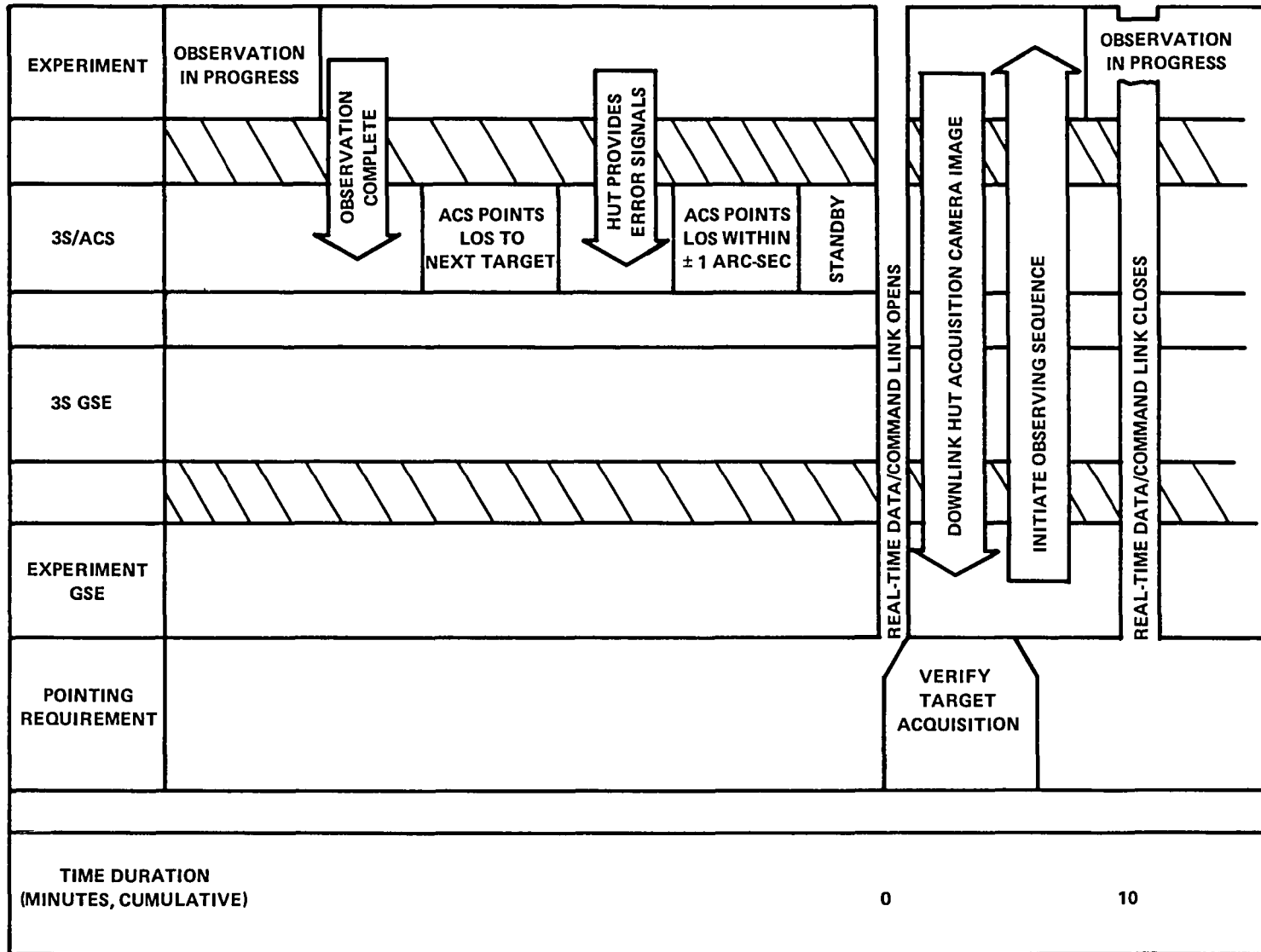
Figure 4-4. Automated Target Acquisition Sequence for a 3S Astronomy Payload
