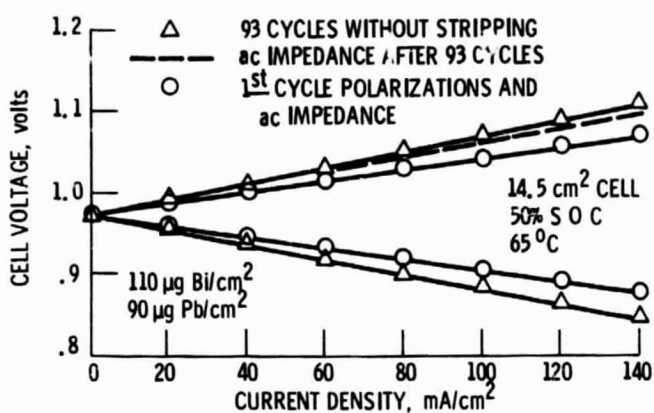
Figure 5. - Performance of mismatch-lead catalyzed system.
