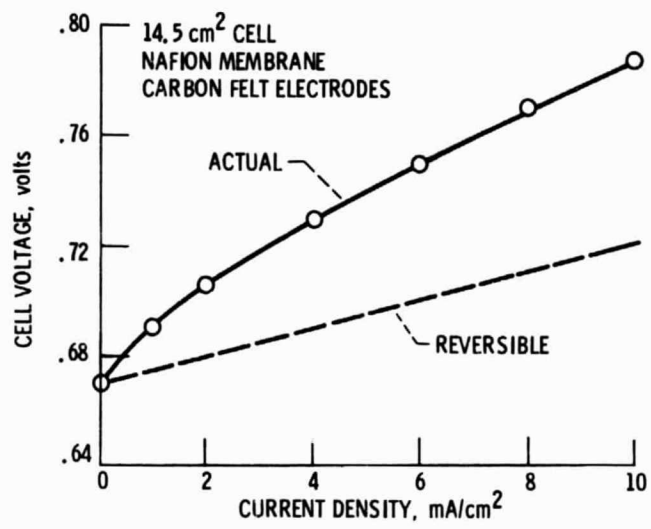
Figure 11. - Iron-Chlorine recharge cell polarization performance.
