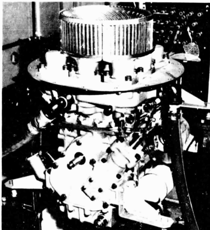
Figure 9-8. 4-95 Standard Involute Heat Exchanger
