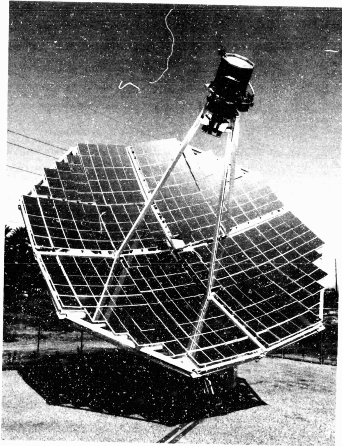
Figure 10-1. Vanguard Dish/Stirling Module
