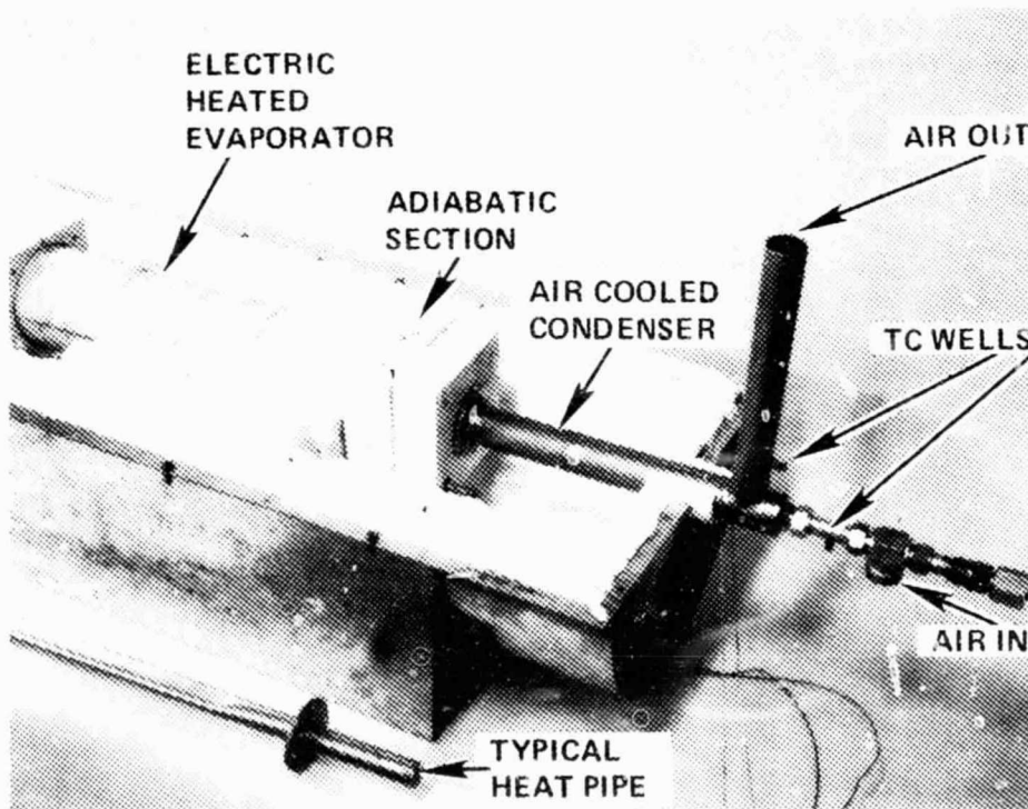
Figure 7-16. Heat Pipe Test Facility
