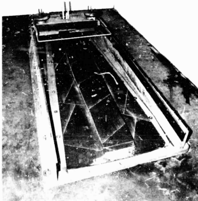
Figure 7-6. Cellular Glass Contouring Apparatus
