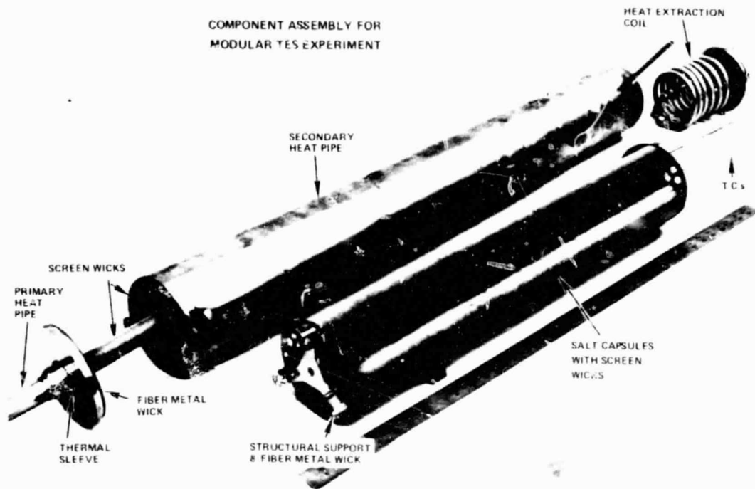
Figure 7-18. TES Modular Experiment Components
