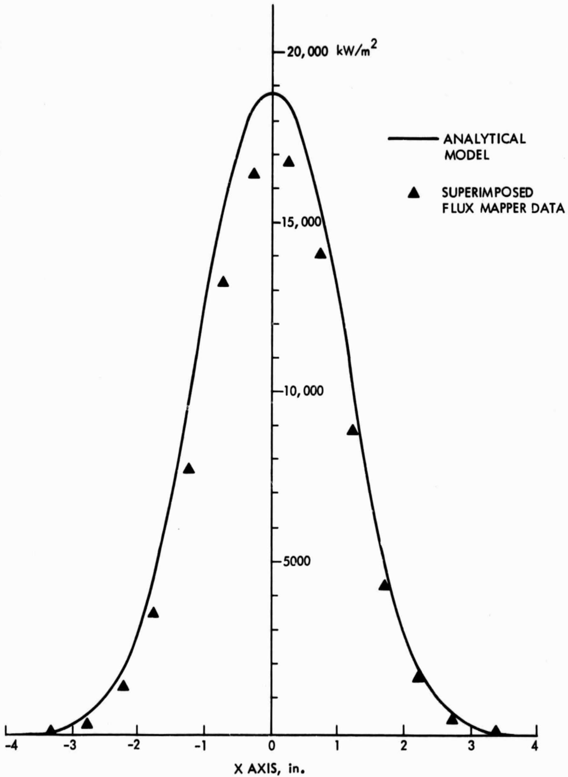
Figure 8-5. Aperture Plane Flux Profiles (100% Mirror Configuration)
