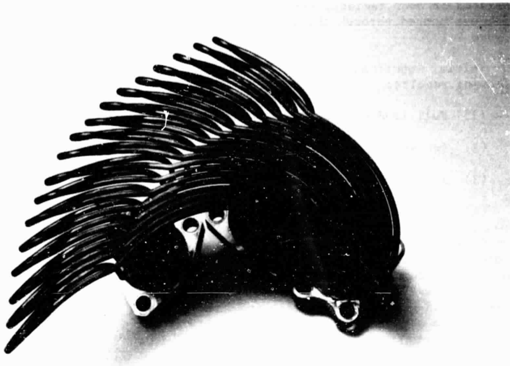
Figure 9-14. ESOR-IV Quadrant, Including Cylinder and Regenerator Housings
