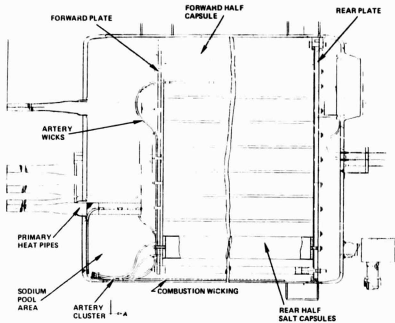
Figure 7-21. Secondary Heat Pipe Wicking
