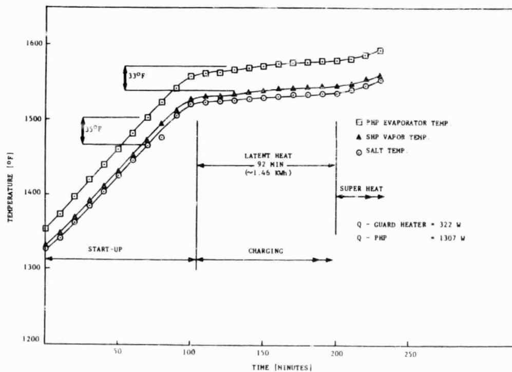
Figure 7-19. Typical TES Charging Curve for the Modular Experiment
