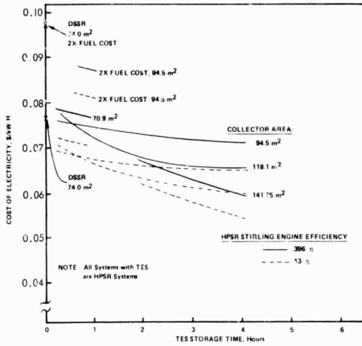
Figure 7-15. Cost of Electricity versus TES Storage Time for Systems with Combustors
