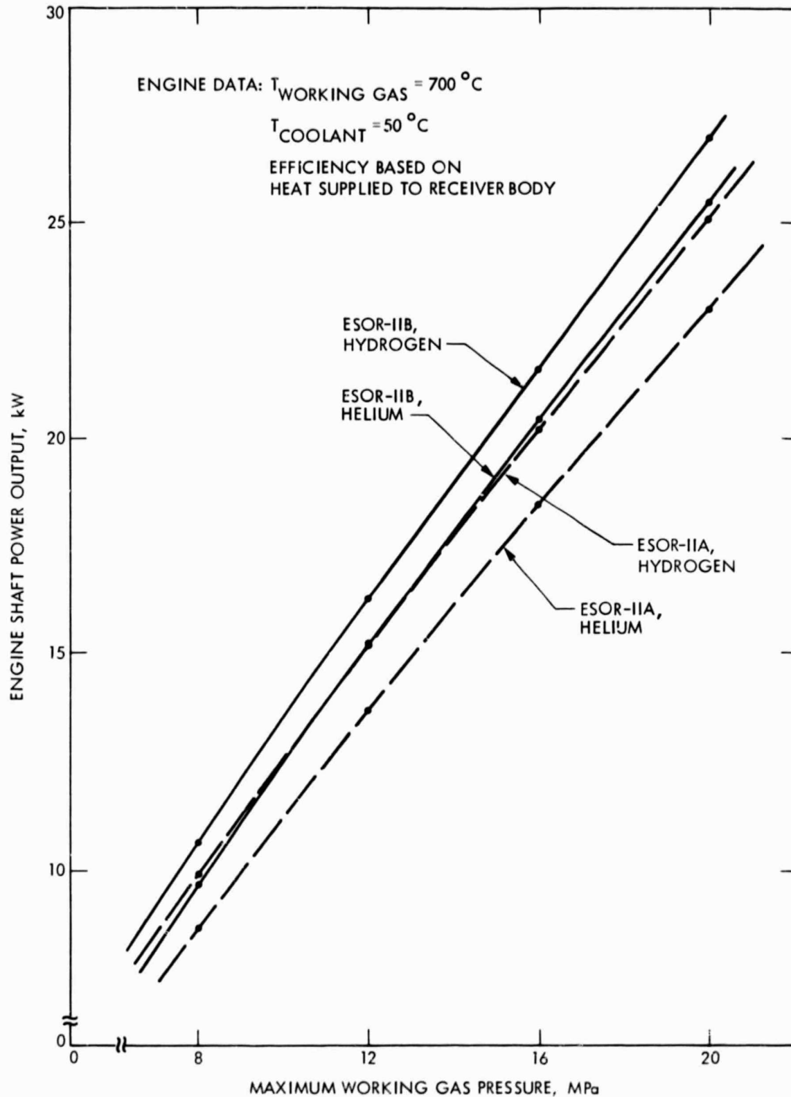
Figure 9-6. Calculated Performance of ESOR-IIA and ESOR-IIB, Power Output versus Maximum Working Gas Pressure
