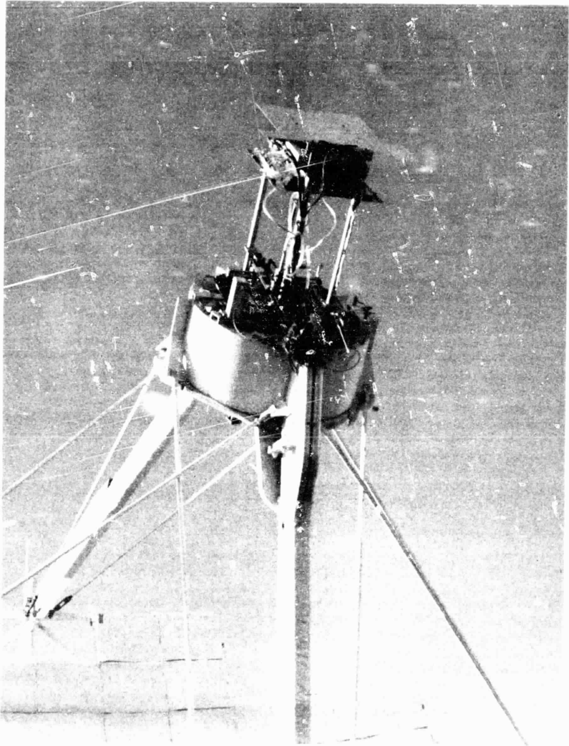
Figure 8-2. Close-Up of Flux Mapper from Outer End
