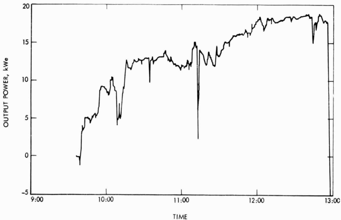
Figure 9-9. Variation of Output Power with Time
