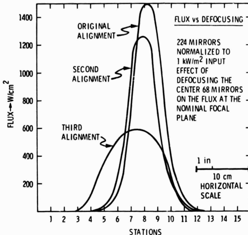
Figure 8-3. Solar Flux Measurements on Test Bed Concentrators
