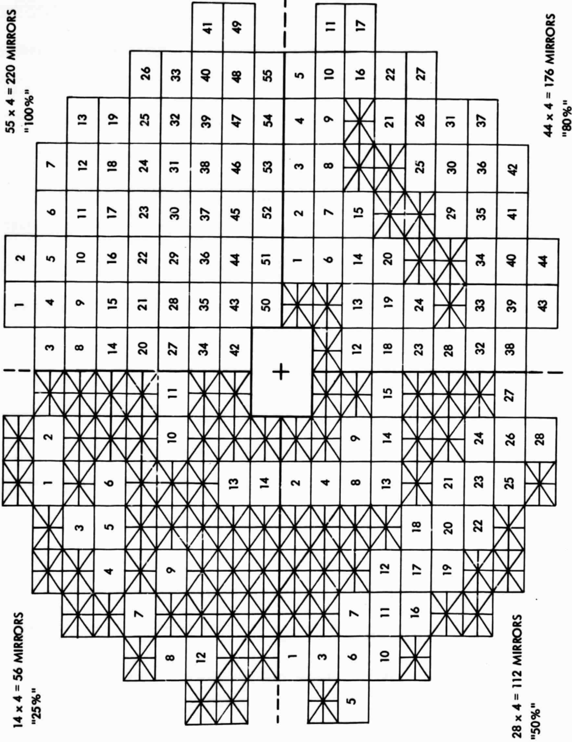
Figure 8-12. TBC Mirror Configurations
