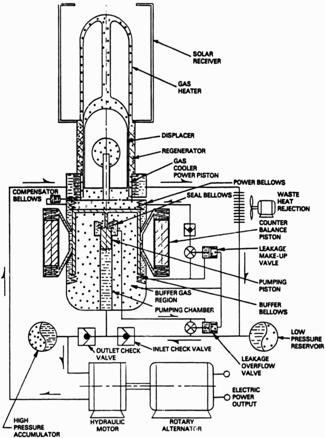
Figure 7-12. Stirling Hydraulic System Schematic
