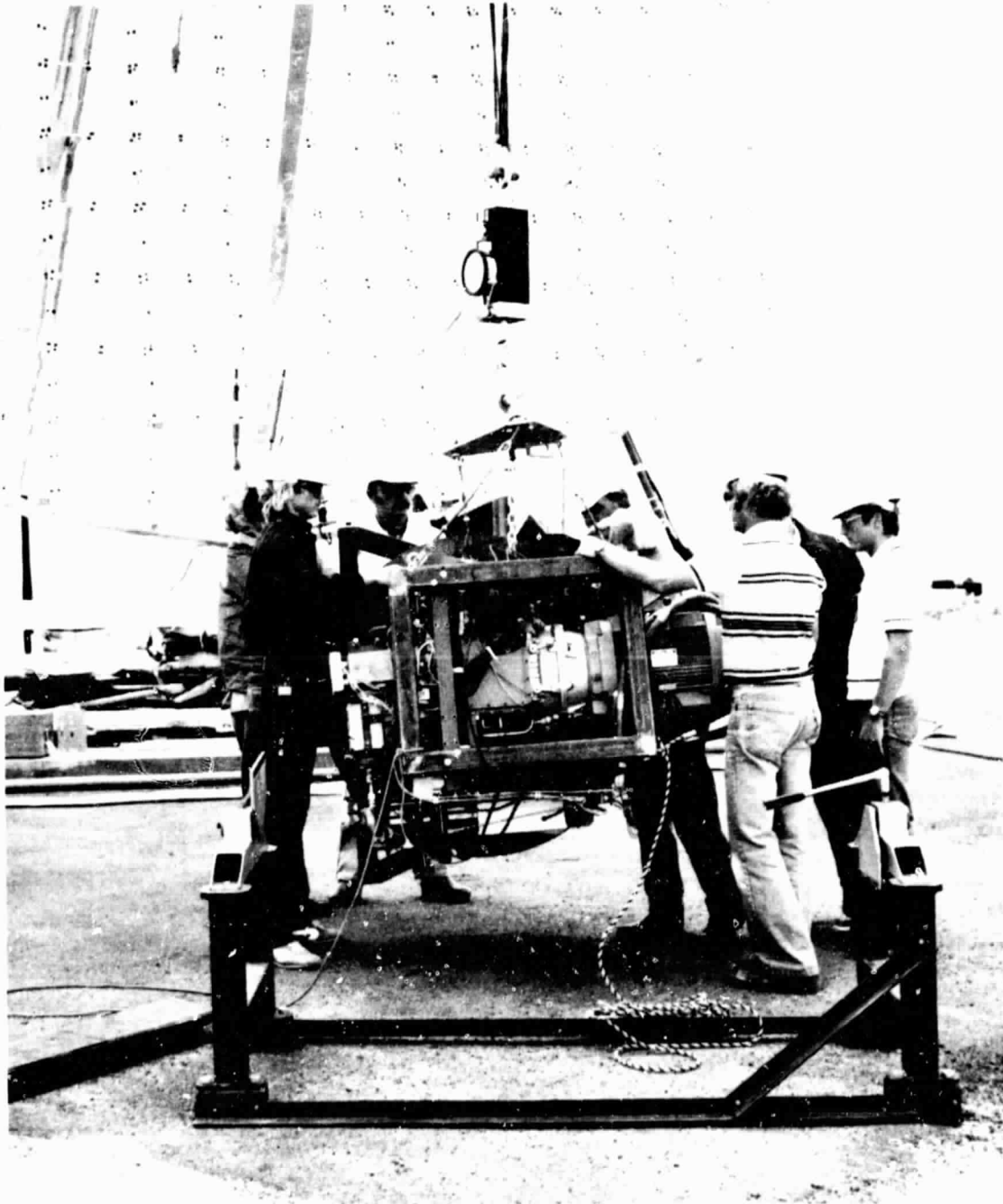
Figure 8-15. First Dish/Stirling Power Conversion Unit Being Mounted on TBC-2
