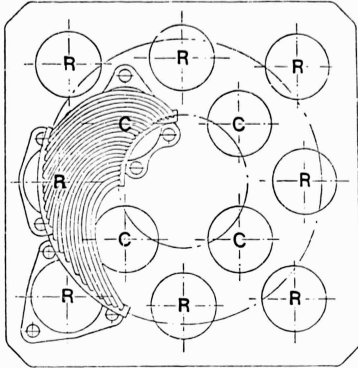
Figure 8-17. P-40 Cylinder and Regenerator Arrangement
