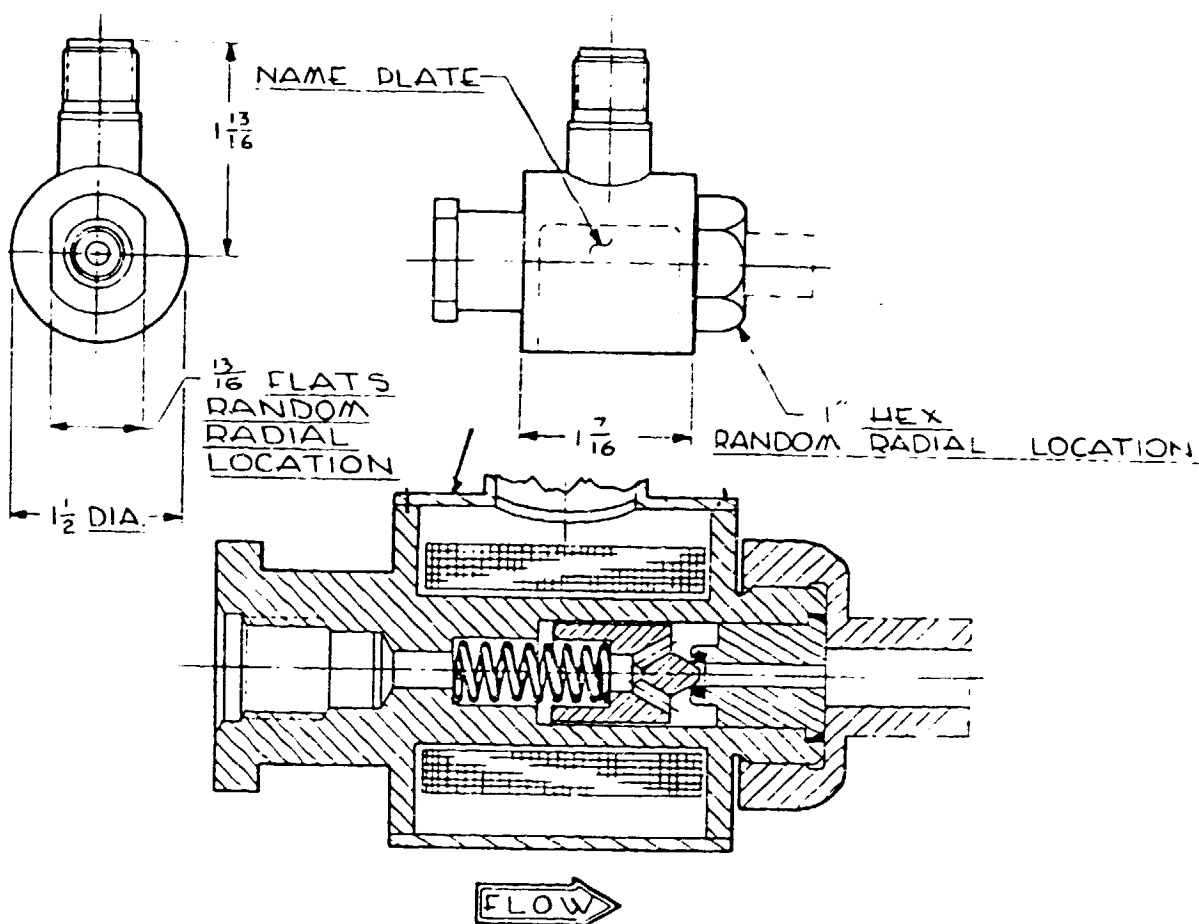
SCHEMATIC SECTIONAL VIEW
