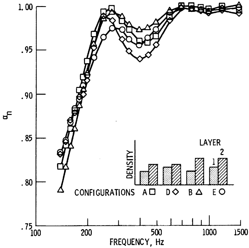
Figure 9. - Measured normal absorption coefficients of 2 layer configurations with variations in the first layer density.
