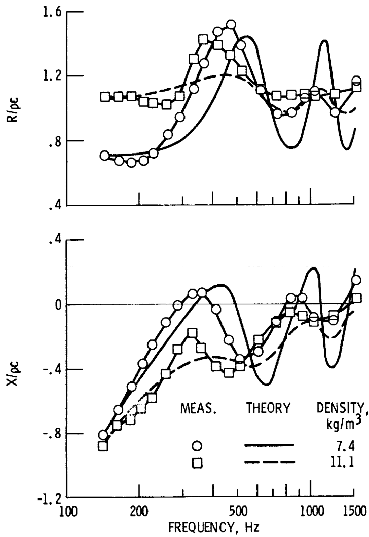
Figure 4. - Specific acoustic impedance of uniform density bulk absorbers with depth of 30.5 cm (12 in).
