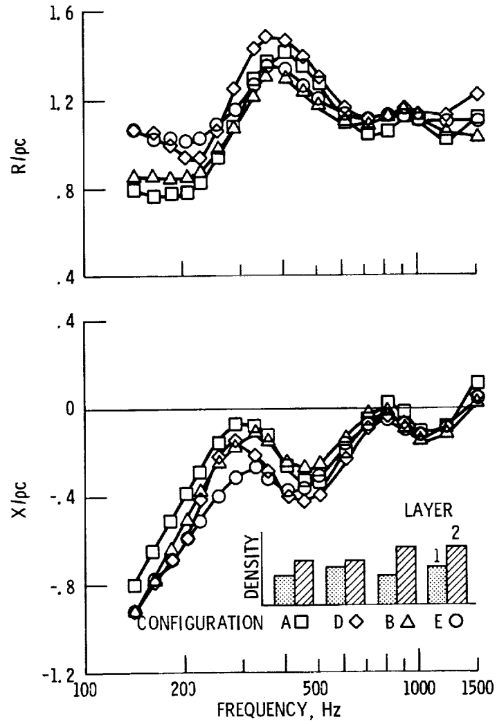
Figure 8. - Measured specific acoustic impedance of 2 layer configurations with variations in the first layer density.
