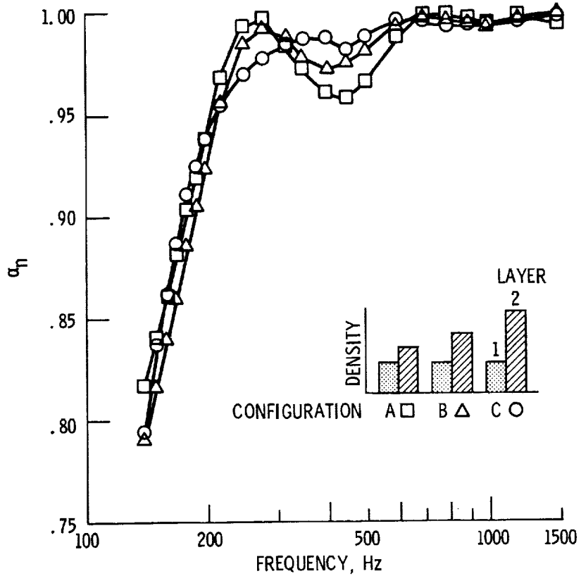
Figure 7. - Measured normal absorption coefficients of 2 layer configurations with variations in the second layer density.
