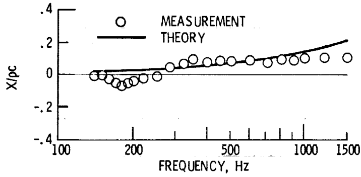
Figure 3. - Specific acoustic reactance of a 40% open perforated plate.
