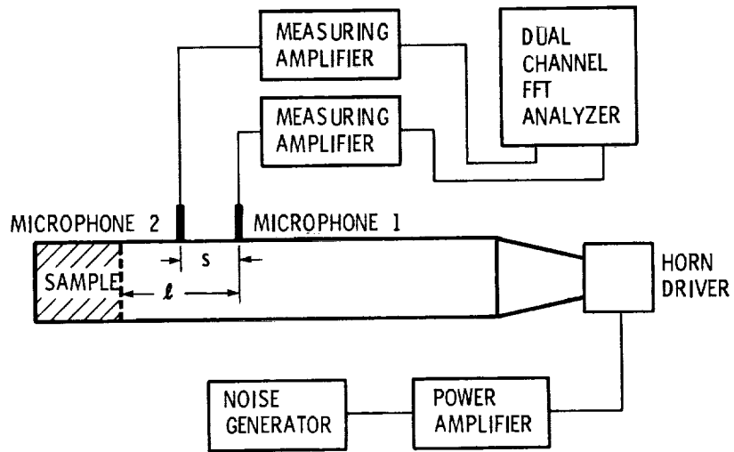
Figure 1. - Acoustic impedance tube schematic and equipment block diagram.
