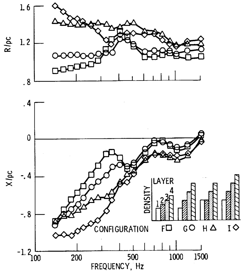
Figure 10. - Measured specific acoustic impedance of 4 layer configurations.
