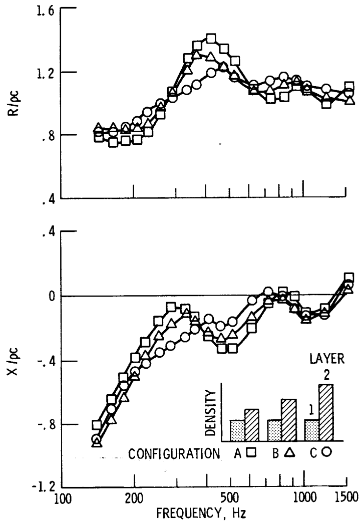
Figure 6. - Measured specific acoustic impedance of 2 layer configurations with variations in the second layer density.
