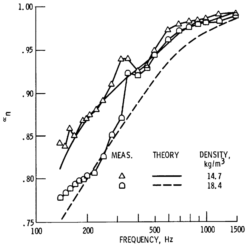
Figure 5. - Normal absorption coefficient of uniform density bulk absorbers with depth of 30.5 cm (12 in).
