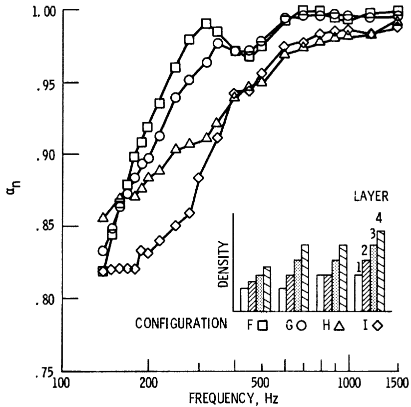
Figure 11. - Measured normal absorption coefficients of 4 layer configurations.
