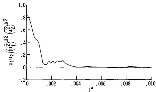
Figure 4. - Calculated correlation coefficient for two velocity components plotted against dimensionless time. No mean shear; (\overline{u_0^2})^{1/2} x_0/\nu = 2217 ; 32^3 grid points.
