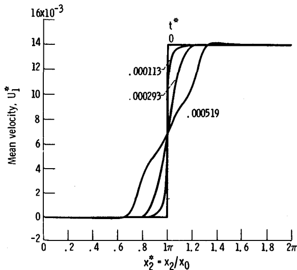
Figure 26. - Calculated development of shear layer mean-velocity profile with dimensionless time. (\overline{u_0^2})^{1/2} x_0/\nu = 554 ; v^* = 2216 in eq. (71); 32^3 grid points.
