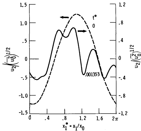
Figure 17. Nonlinear solution for u_2 / (\overline{u_0^2})^{1/2} plotted against x_1^* . x_2^* = 9\pi/8 ; x_3^* = 3\pi/8 ; (dU_1/dx_2)^* = 4434 ; (\overline{u_0^2})^{1/2} x_0/\nu = 1108 ; 32^3 grid points.
