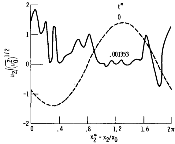
Figure 16. - Nonlinear solution for u_2 / (\overline{u_0^2})^{1/2} plotted against x_2^* . x_1^* = 9\pi/8 ; x_3^* = 3\pi/8 ; (dU_1/dx_2)^* = 4434 ; (\overline{u_0^2})^{1/2} x_0/\nu = 1108 ; 32^3 grid points.
