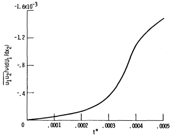
Figure 27. - Calculated time variation of ratio of turbulent-to-viscous shear stress for developing shear layer at x_2^* = \pi \cdot \left(\frac{2}{\psi_0}\right)^{1/2} x_0/v = 554 ; v^* = 2216 in eq. (71); 32^3 grid points.
