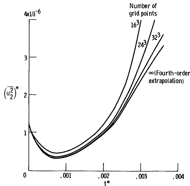
Figure 20. Effect of numerical mesh size on evolution of \overline{u_2^2}^* . (dU_1/dx_2)^* = 4434 ; (\overline{u_0^2})^{1/2} x_0/\nu = 1108 .
