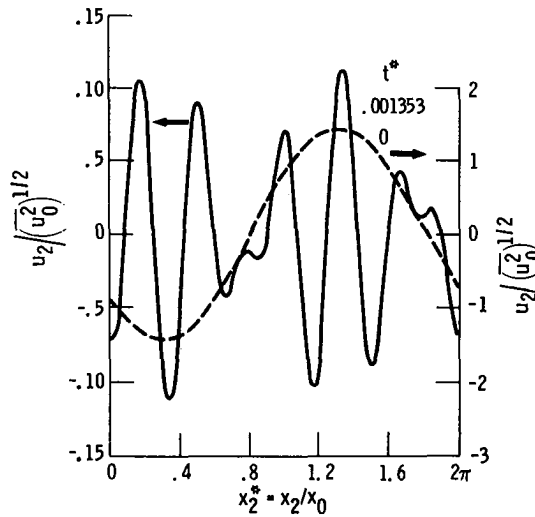
Figure 15. - Linearized analytical solution for u_2 / (\frac{2}{u_0})^{1/2} plotted against x_2^* for unbounded (eq. (60)). x_1^* = 9\pi/8; x_3^* = 3\pi/8; (dU_1/dx_2)^* = 4434; (\frac{2}{u_0})^{1/2} x_0/\nu = 1108 .
