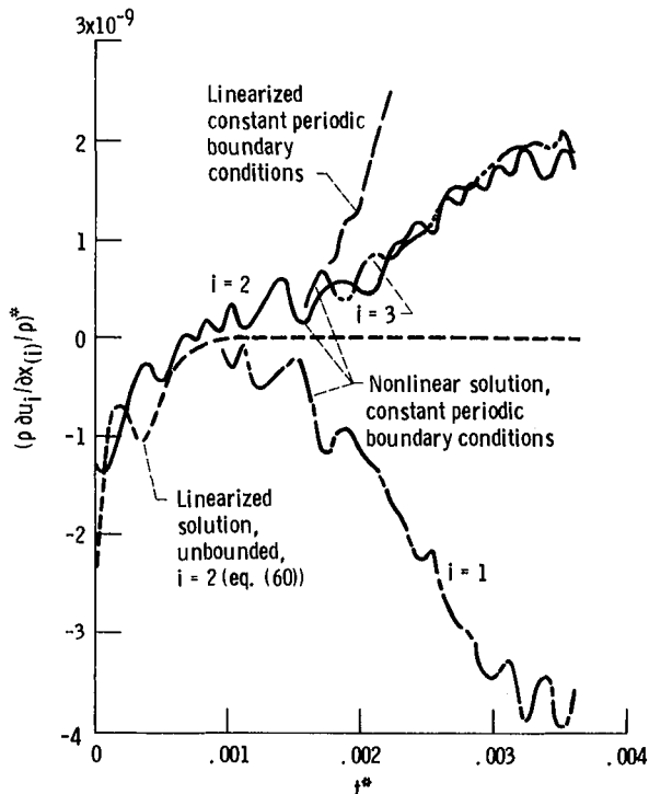
Figure 21. - Calculated evolution of pressure-velocity-gradient correlations. (dU_1/dx_2)^* = 4434 ; (\overline{u_0^2})^{1/2} x_0/\nu = 1108 ; 32^3 grid points.
