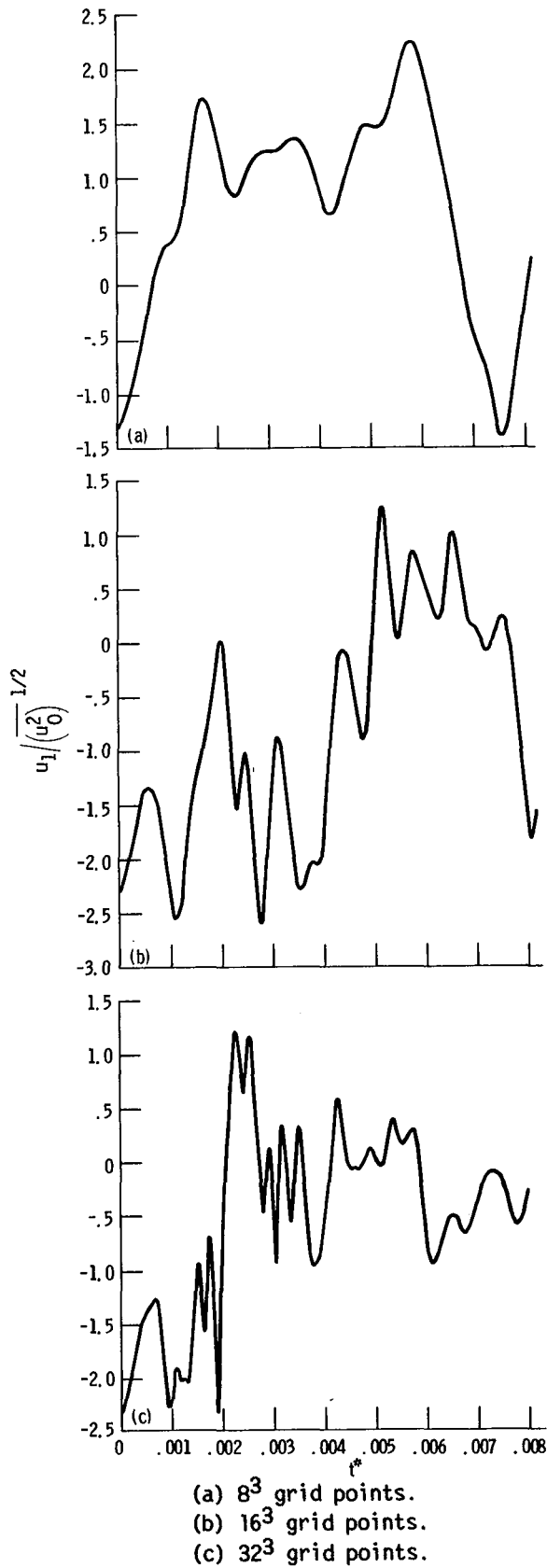
Figure 2. - Effect of numerical mesh size on calculated evolution of velocity fluctuations. No mean shear; (\overline{u_0^2})^{1/2} x_0/\nu = 2217 ; x_1^* = \pi (at grid center).
