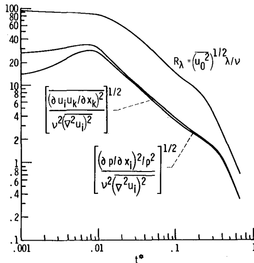
Figure 12. - Three measures of relative importance of inertial and viscous effects plotted against dimensionless time. No mean shear; \frac{\overline{u_0^2}}{2}^{1/2} x_0 / \nu = 69.3 ; i = 1, 2, \text{ or } 3 ; extrapolated to zero mesh size.
