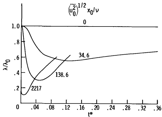
Figure 9. - Calculated evolution of microscale of velocity fluctuations (normalized by initial value) for various initial Reynolds numbers. No mean shear; extrapolated to zero mesh size.
