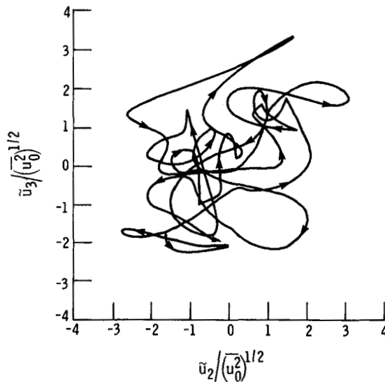
Figure 32. - Calculated trajectory of phase point projected on u_2 - u_3 plane at numerical grid center with a spatially periodic body force. 0.26 < t^* < 0.32 ; (\bar{u}_0^2)^{1/2} x_0/\nu = 138.6 ; 32^3 grid points. Arrows indicate direction of time.
