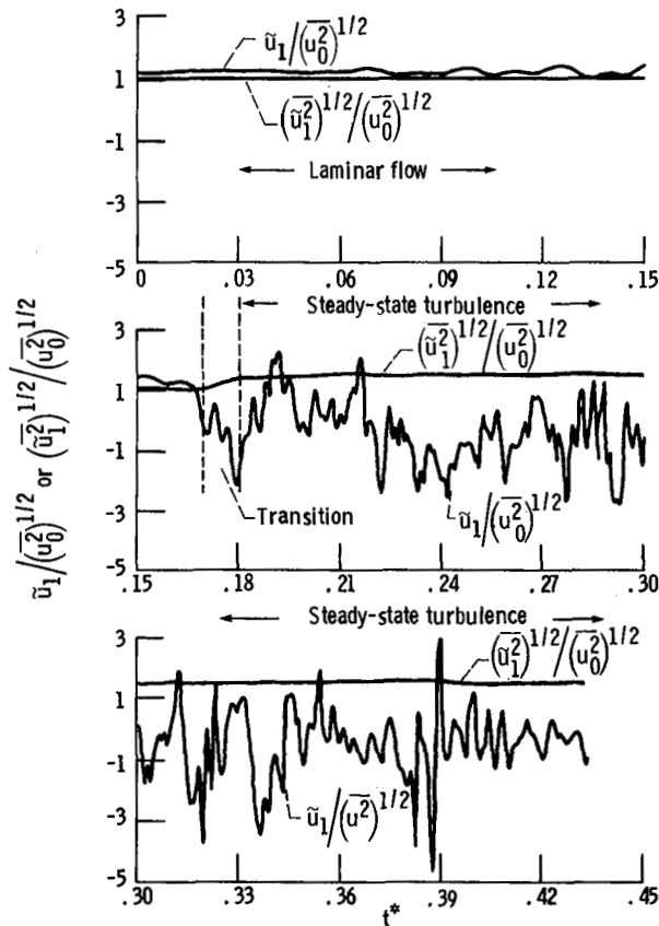
Figure 31. - Calculated evolution of turbulent velocity fluctuations (normalized by initial condition) with a spatially periodic body force. (\bar{u}_0^2)^{1/2} x_0/\nu = 138.6 ; x_1^* = x_2^* = 9\pi/8 ; x_3 = 3\pi/8 for unaveraged fluctuations. Root-mean-square fluctuations spatially averaged; 32^3 grid points.
