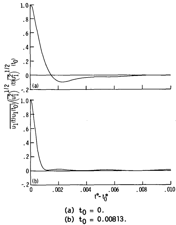
Figure 3. - Calculated correlation coefficient for velocities at dimensionless times t_0^* and t_0^* plotted against t^* - t_0^* . No mean shear; (\overline{u_0^2})^{1/2} x_0/\nu = 2217 ; 32^3 grid points.
