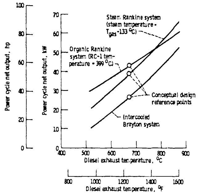
Figure 26.—Sensitivity of alternative power cycle performance to diesel exhaust temperature. (Diesel exhaust flow rate 1309 kg/hr (2886 lb/hr).)
