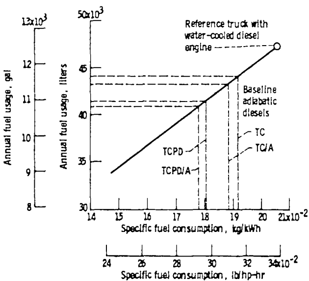
Figure 5.—Correlation of engine specific fuel consumption to annual fuel usage for the fuel saver truck configuration.
