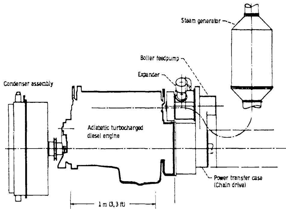
Figure 9.—Diesel/steam system layout.
