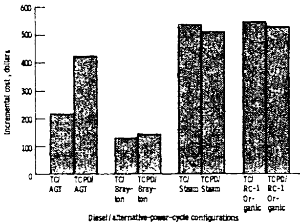
Figure 20.—Incremental annual maintenance and repair costs for various diesel/alternative-power-cycle combinations normalized to 261 kW (350 hp) total power. The incremental price is based on the TCPD/A diesel cost of $4015 per year.
