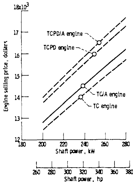
Figure 6.—Diesel engine price correlations.
