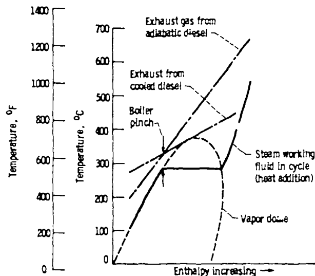
Figure 25.—Heat addition profile of steam Rankine cycle.
