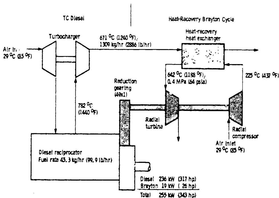
Figure 13.—Diesel/pressurized Brayton system schematic.
