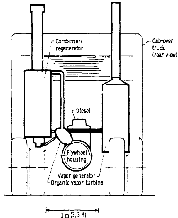
Figure 11.—Diesel/organic system layout.
