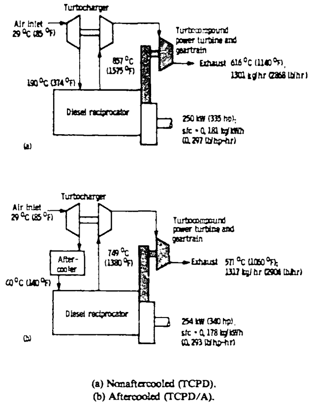
(a) Nonaftercooled (TCPD). (b) Aftercooled (TCPD/A). Figure 2.—Turbocompound diesel configurations.
