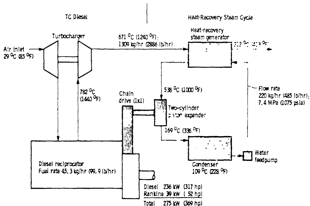
Figure 8.—Diesel/steam system schematic. Rankine cycle power output is based on highway operation with condenser fan declutched.
