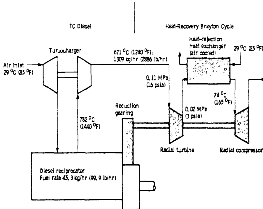
Figure 12.—Diesel/subatmospheric Brayton system schematic.
