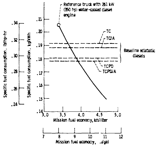
Figure 4.—Correlation of engine specific fuel consumption to truck fuel economy for the fuel saver truck configuration.
