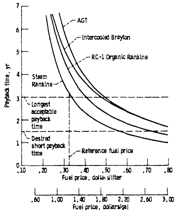
Figure 23.—Payback time for various TCPD diesel/alternative-power-cycle combinations with the TCPD/A diesel as a baseline for payback comparison.
