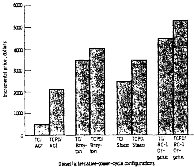
Figure 19.—Incremental price of various diesel/alternative-power-cycle combinations normalized to 261 kW (350 hp) total power. The incremental price is based on the TCPD/A diesel price of $16 838.
