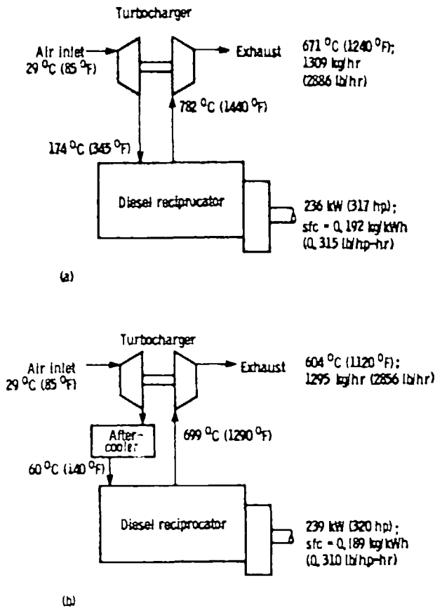
(a) Nonaftercooled (TC). (b) Aftercooled (TC/A). Figure 1.—Turbocharged diesel configurations.
