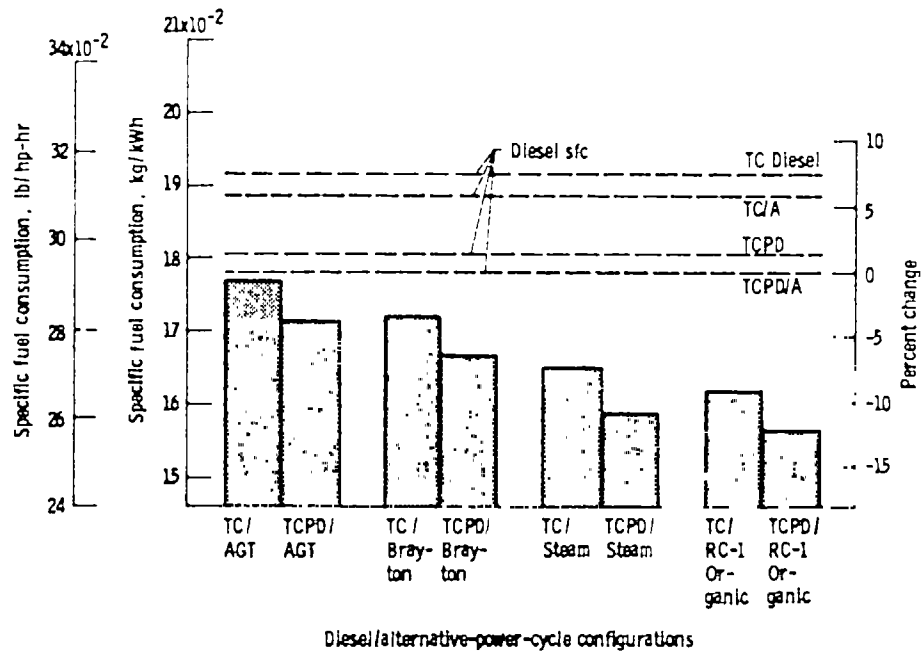
Figure 16.—Specific fuel consumption (sfc) for various diesel/alternative-power-cycle combinations.
