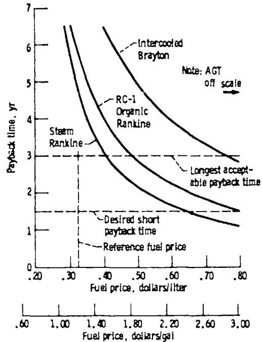
Figure 22.—Payback time for various TC diesel/alternative-power-cycle combinations with the TCPD/A diesel as a baseline for payback comparison.
