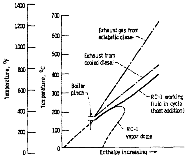
Figure 24.—Heat addition profile of RC-1 organic Rankine cycle.
