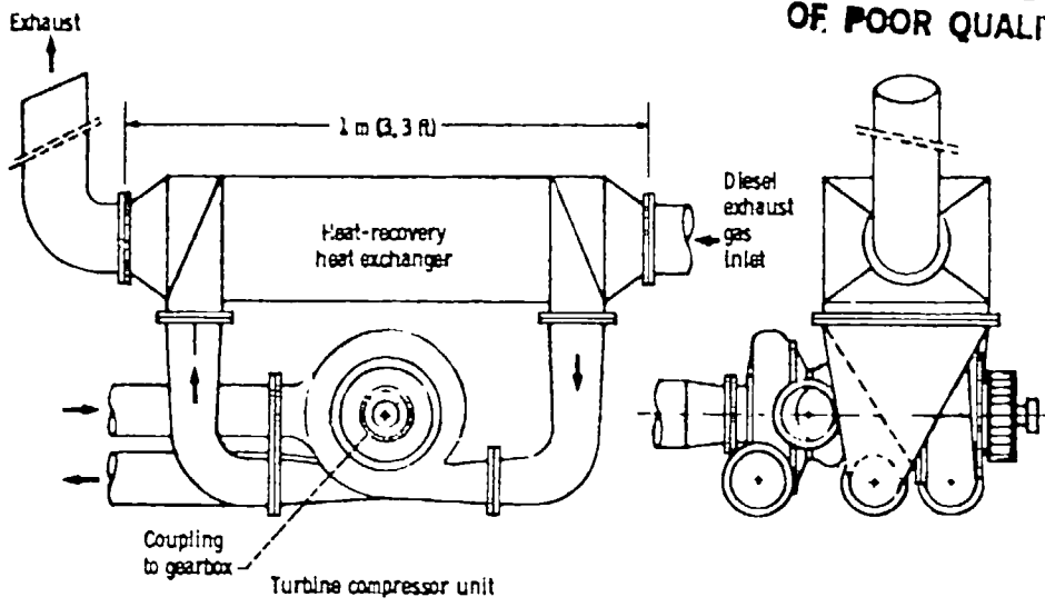
Figure 15.—Pressurized (intercooled) Brayton system layout.
