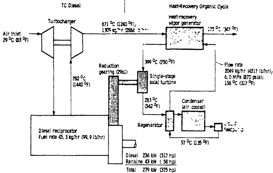
Figure 10.—Diesel/RC-1 organic system schematic. Rankine cycle power output is based on highway operation with condenser fan declutched.
