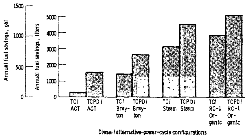
Figure 17.—Incremental annual fuel savings resulting from use of various diesel/alternative power cycles based on the TCPD/A diesel as the baseline configuration and 161 000 km (100 000 mi) annual use.
