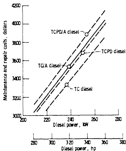
Figure 7.—Diesel maintenance and repair cost correlations. Levelized annual costs are based on a 7-year maintenance and repair contract and 161 000 km (100 000 mi) annual use.
