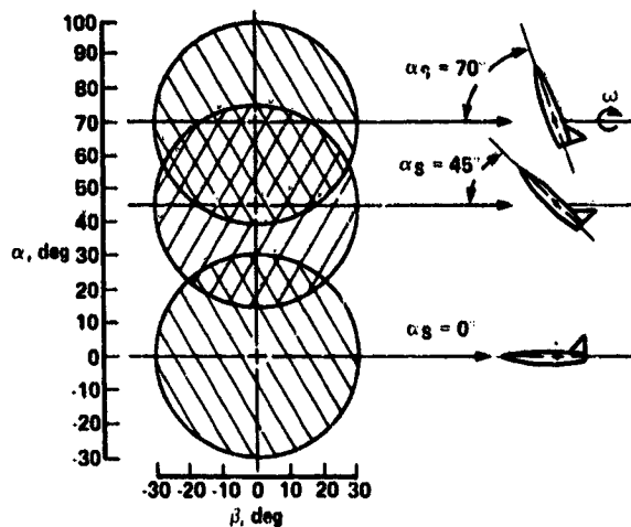
Fig. 4. Attitude envelope for large-scale rotary-balance apparatus.
