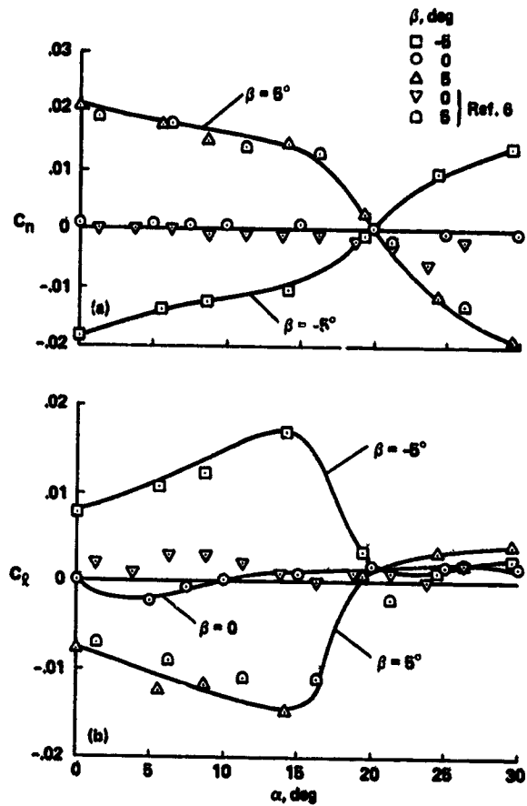
Fig. 21. Lateral-directional aerodynamic coefficients for Standard Dynamics Model. (a) Yawing-moment coefficient. (b) Rolling-moment coefficient.
