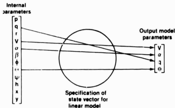
Fig. 2 Selection of state variables for linear model.
