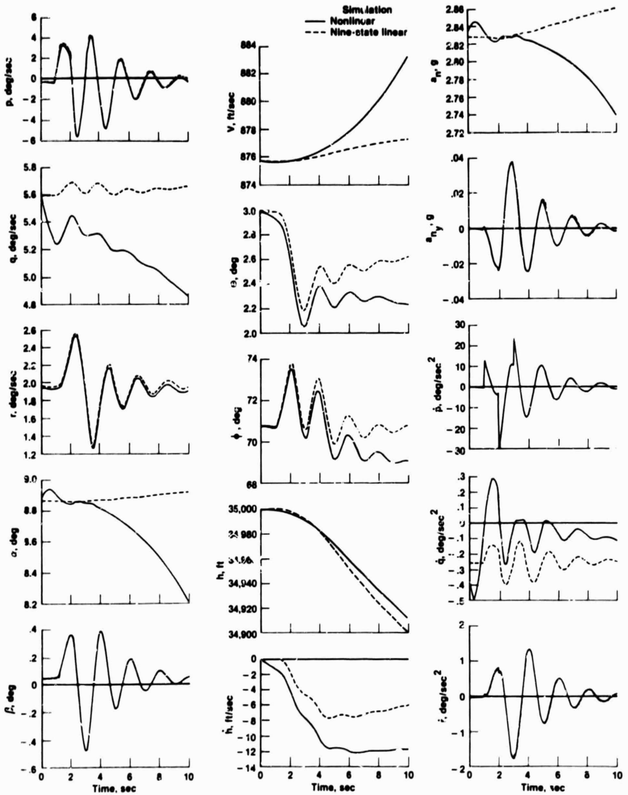
Fig. 5 Comparison of nonlinear and linear simulations of a high-performance aircraft for an aileron doublet; 3g level turn; 0.9 Mach number; at 35,000 ft altitude.
