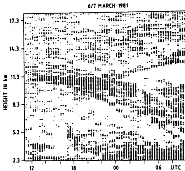
Figure 2. Modified (mean profile subtracted) height-time intensity plot showing sloping layers of enhanced radar reflectivity due to frontal boundaries and tropopause (after ROTTGER, 1981), observed with the SOUSY-VHF Radar.
