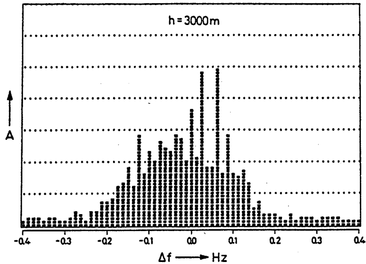
Figure 1. Doppler spectrum of signal measured with vertical antenna beam and 150 m height resolution, averaged over 8 min (from ROTTGER, 1980).
