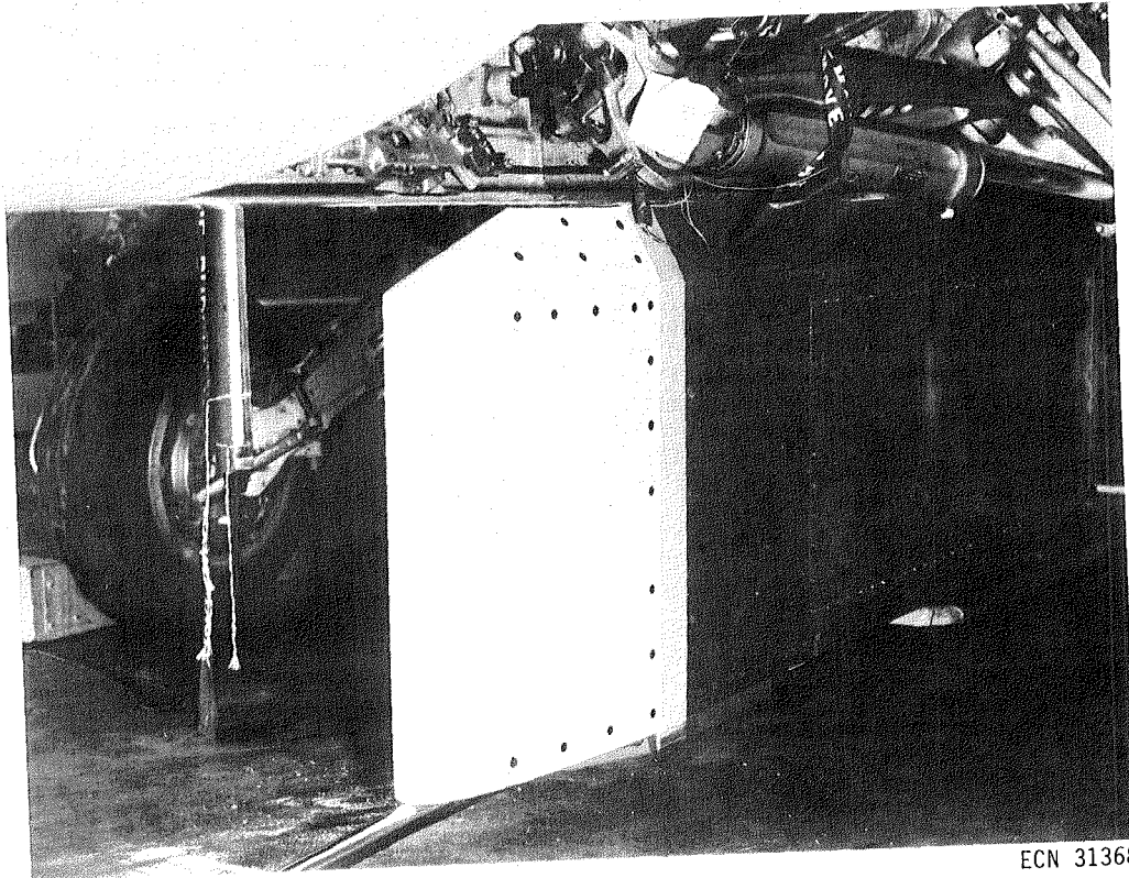
Fig. 2 Flight test fixture.
