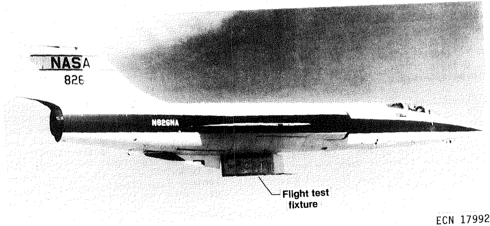
Fig. 1 F-104G aircraft with flight test fixture.
