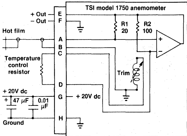
Fig. 4 Constant-temperature hot-film anemometer.
