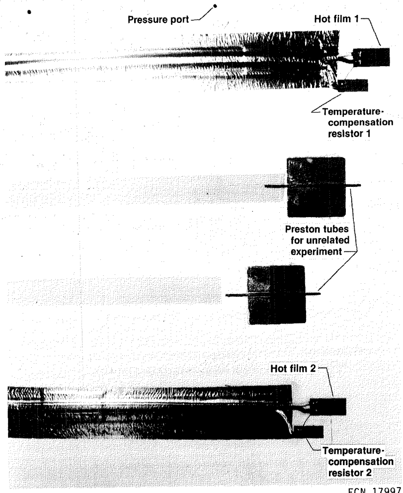
Fig. 3 Hot-film installation.
