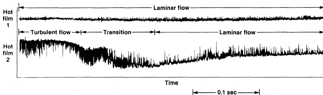
Fig. 7 Hot-film dynamic output for sideslip maneuver.
