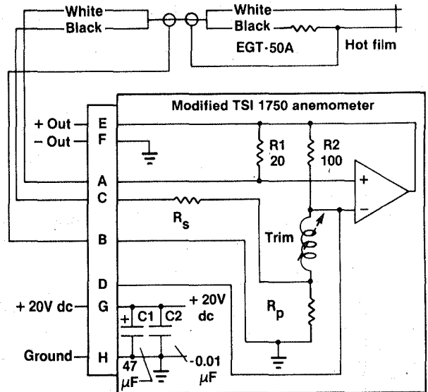
Fig. 5 Temperature-compensated hot-film anemometer.
