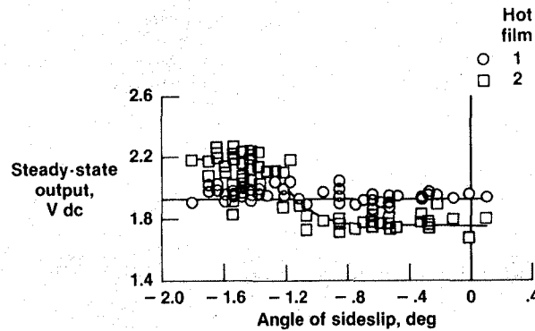
Fig. 6 Hot-film steady-state output for sideslip maneuver. Mach 0.8; altitude = 10,000 ft.
