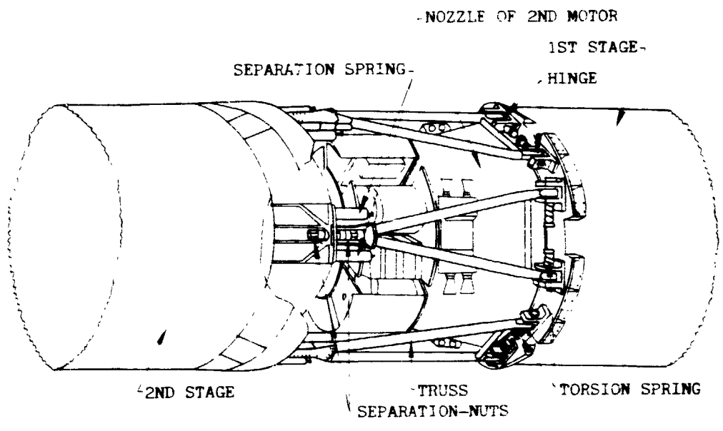
(a) Before Separation
