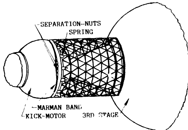
Figure 9. Inter-Stage Joint Between Kick Motor and 3rd Stages
