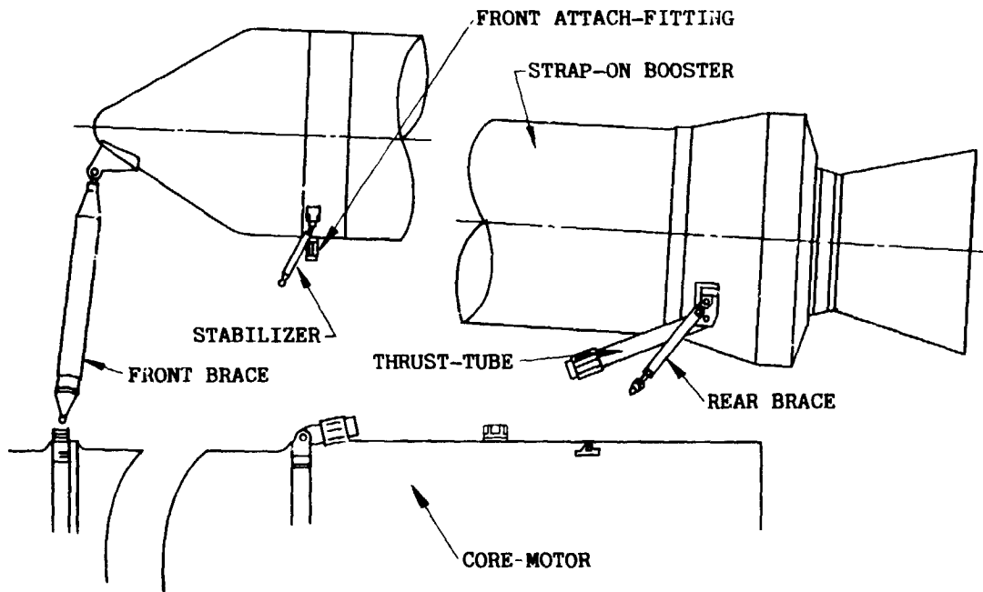
Figure 6 (b). Strap-on Booster Separation System (After Separation)
