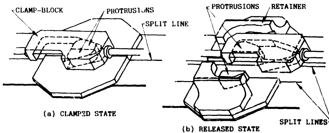
Figure 2. Clamp Mechanism Along Split Line
